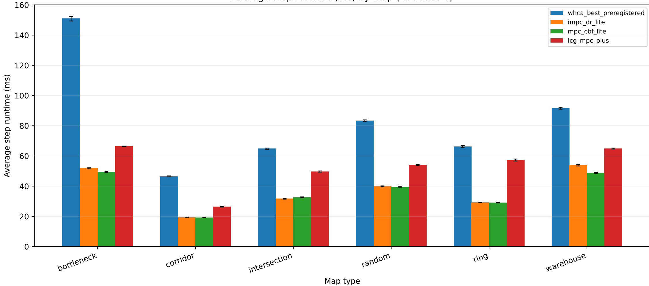
Average step runtime (ms) by map (100 robots)
