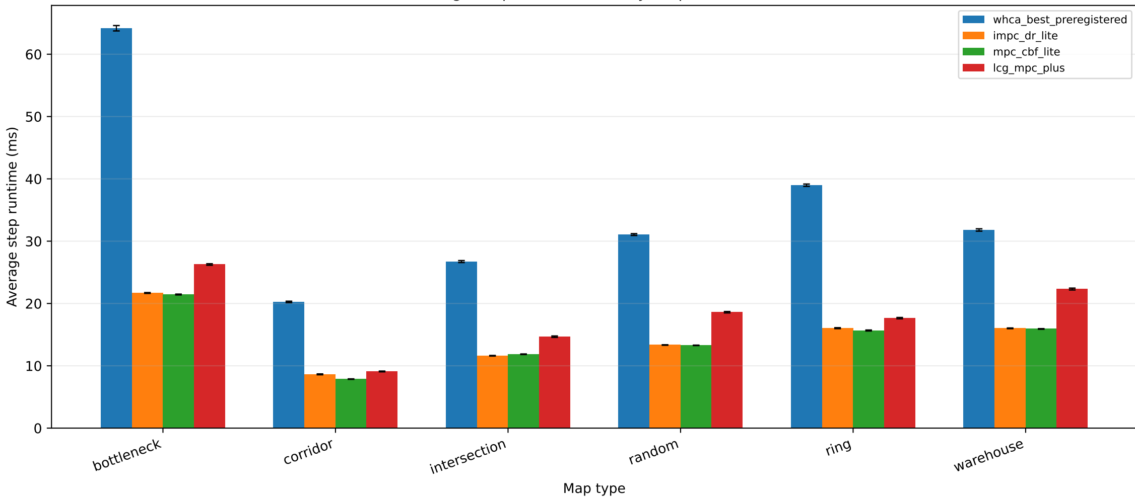
Average step runtime (ms) by map (56 robots)
