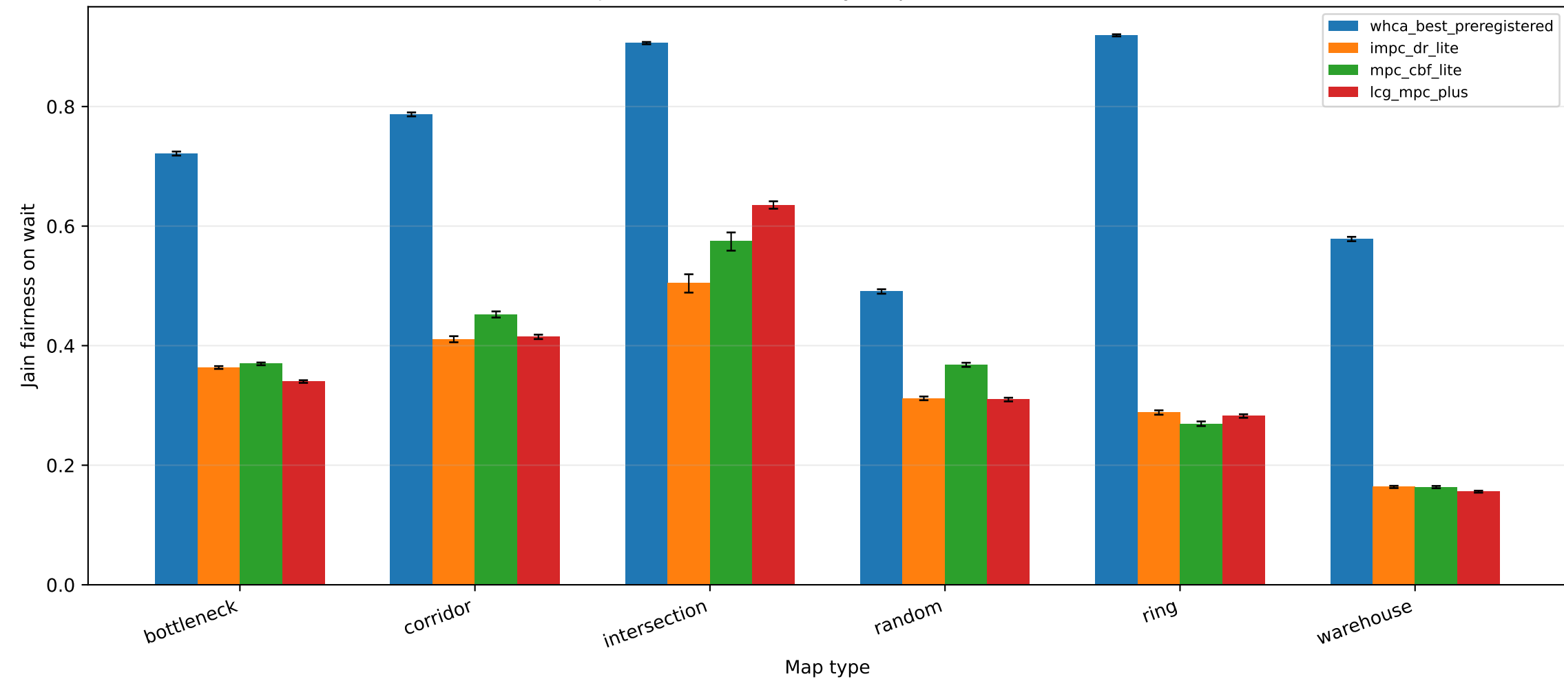
Jain fairness on wait by map (100 robots)
