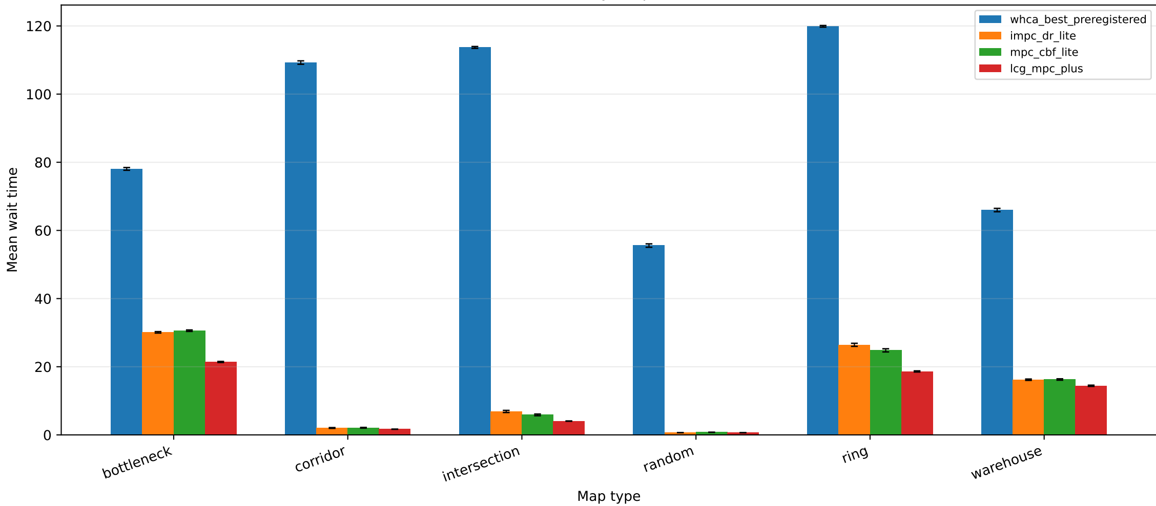
Mean wait time by map (100 robots)
