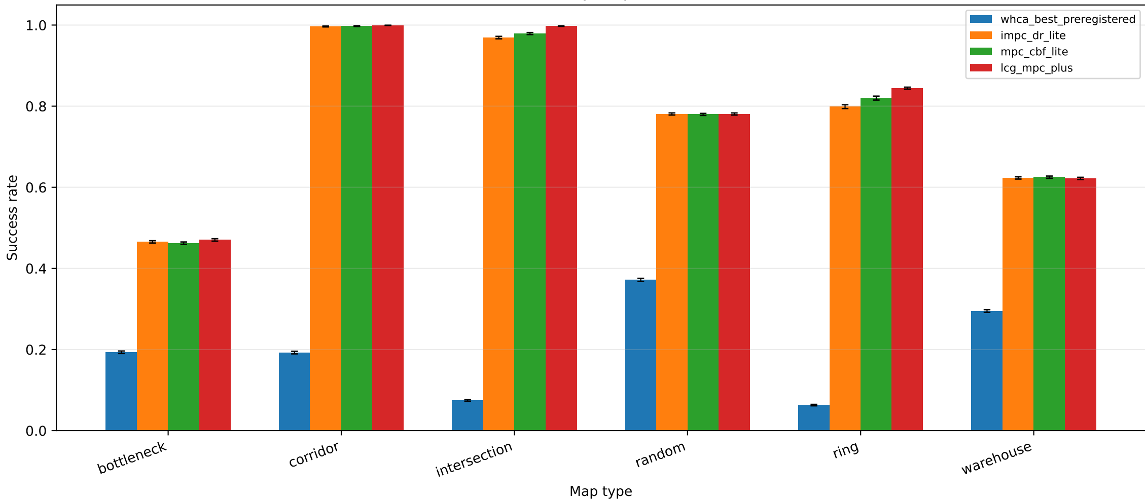
Success rate by map (100 robots)
