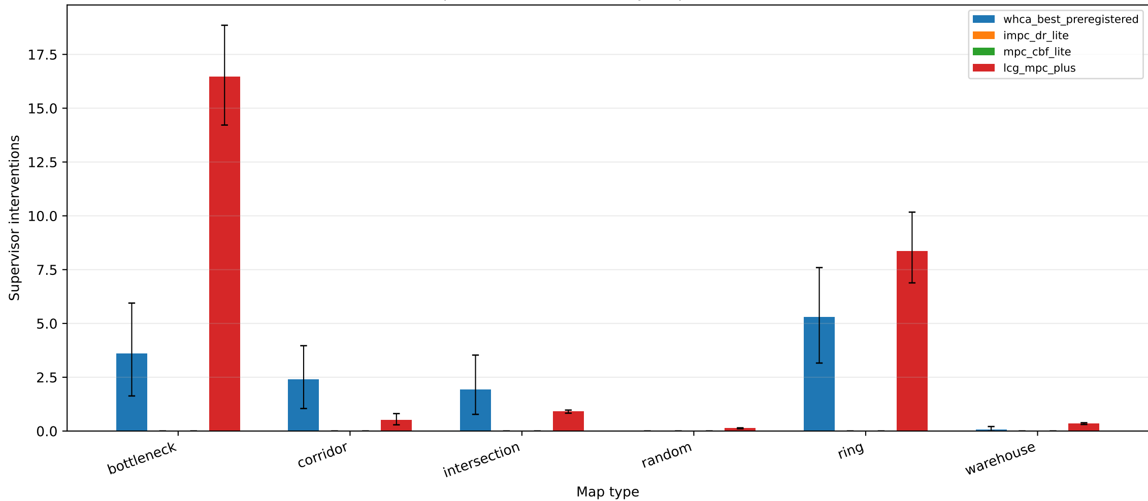
Supervisor interventions by map (100 robots)
