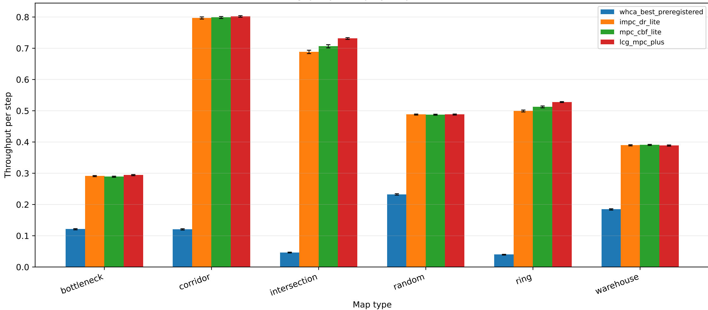
Throughput per step by map (100 robots)
