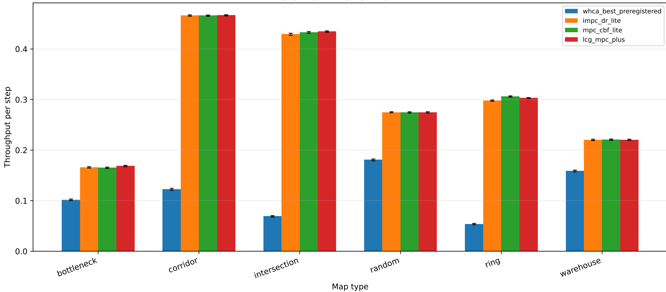
Throughput per step by map (56 robots)
