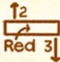
Style Guides
