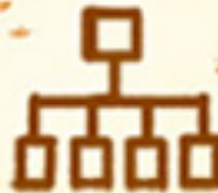
System Maps
