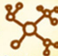
Concept Maps
