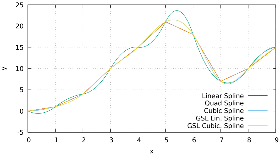
Spline of Random Points
