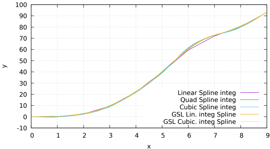
Integration Spline of Random Points
