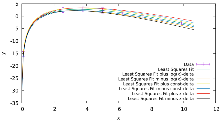
Least Squares Fit to c_1 \cdot \log(x) + c_2 + c_3 \cdot x for Data
