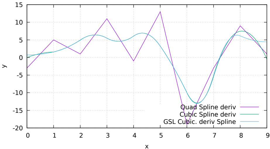
Derivative Spline of Random Points
