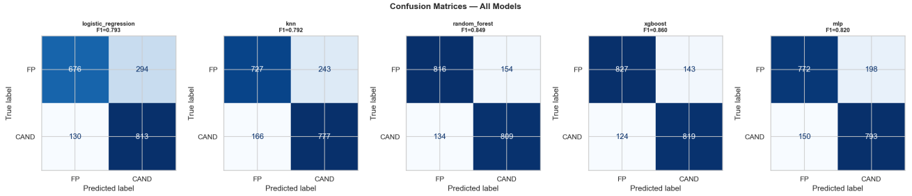
Fig. 7: Confusion matrices on the test set. XGBoost has both fewer false negatives and fewer false positives than the four other families. The F_1 score is annotated above each panel.
