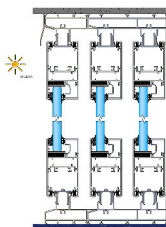
Corte Vertical
