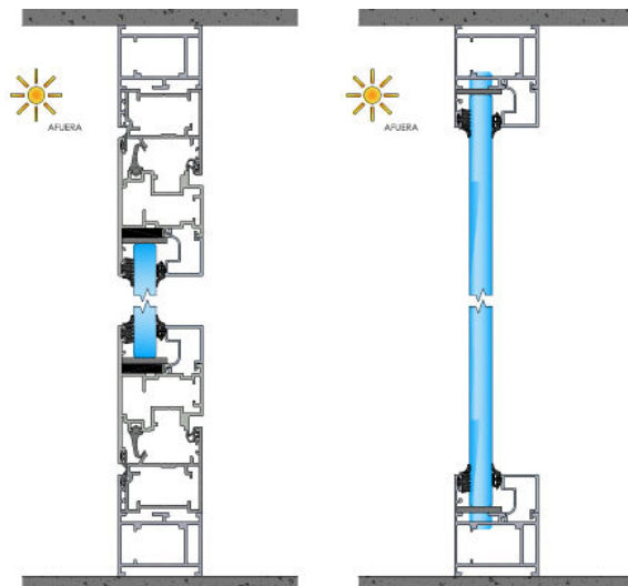
Corte Vertical
