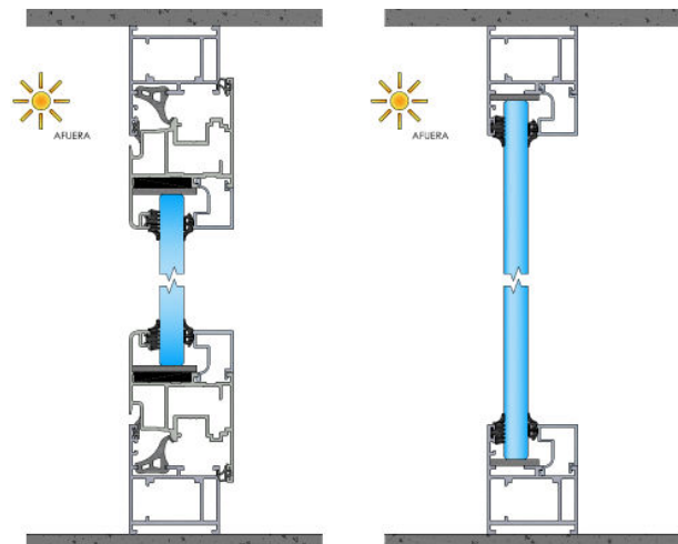
Corte Vertical
