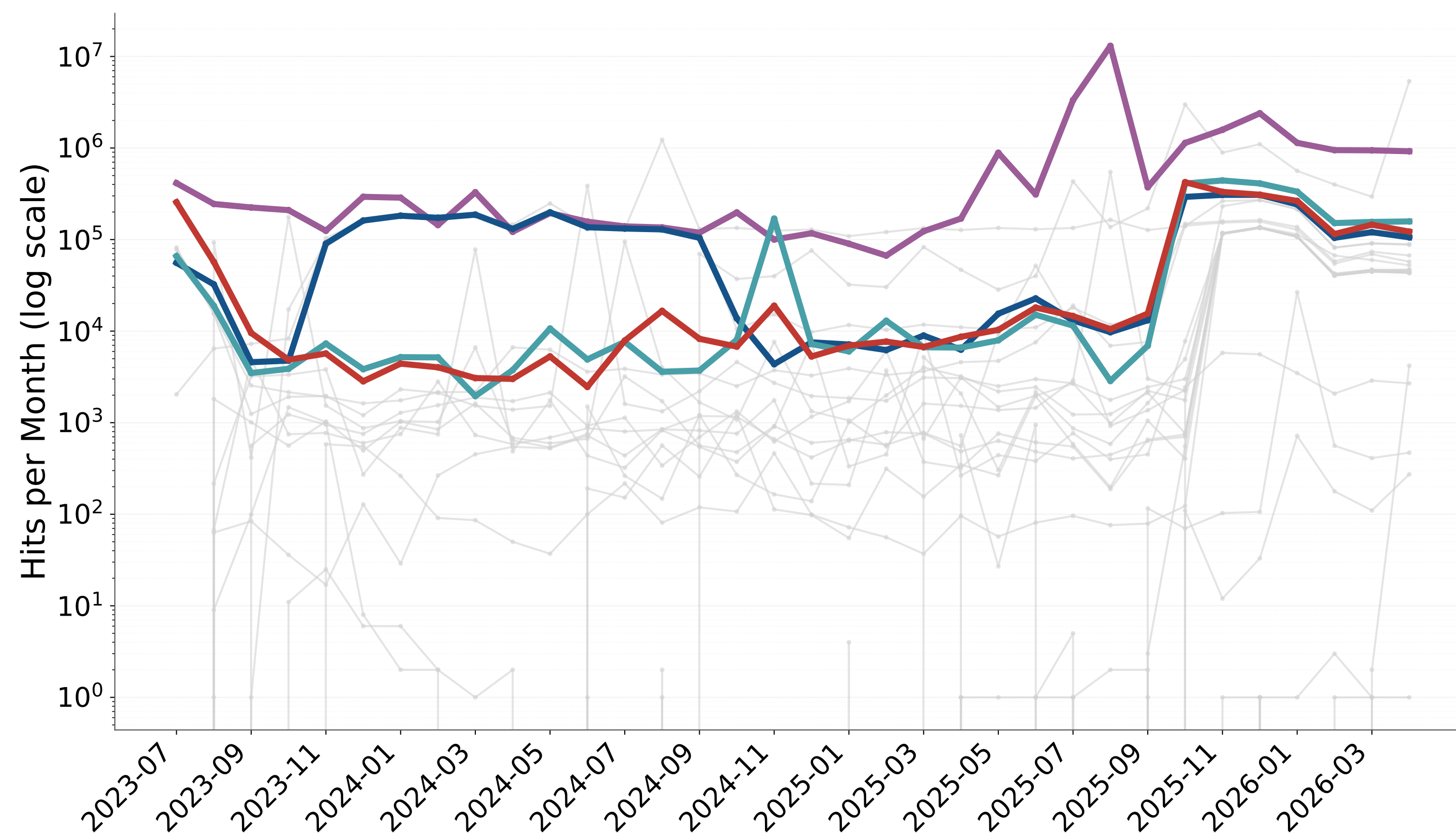
Monthly Total Requests (Aggregated Main Tools) - Unfiltered
