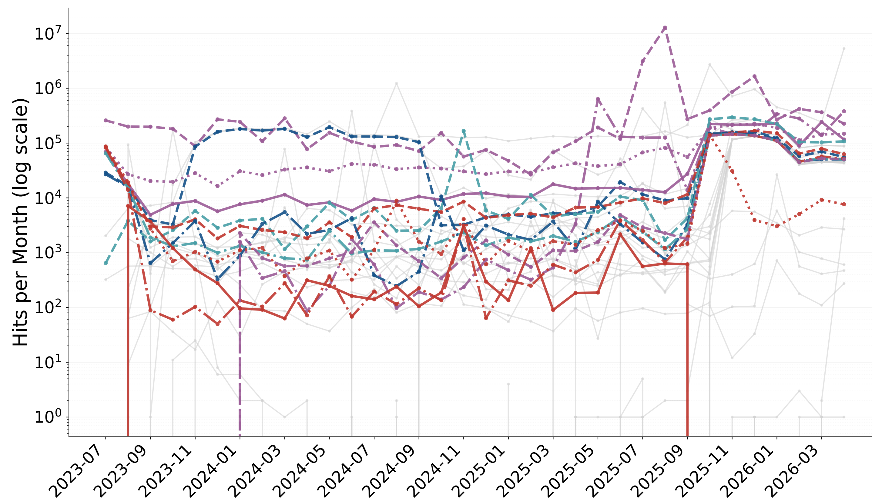
Monthly Total Requests (Individual Components) - Unfiltered
