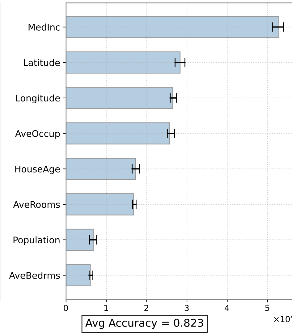
4 bins
