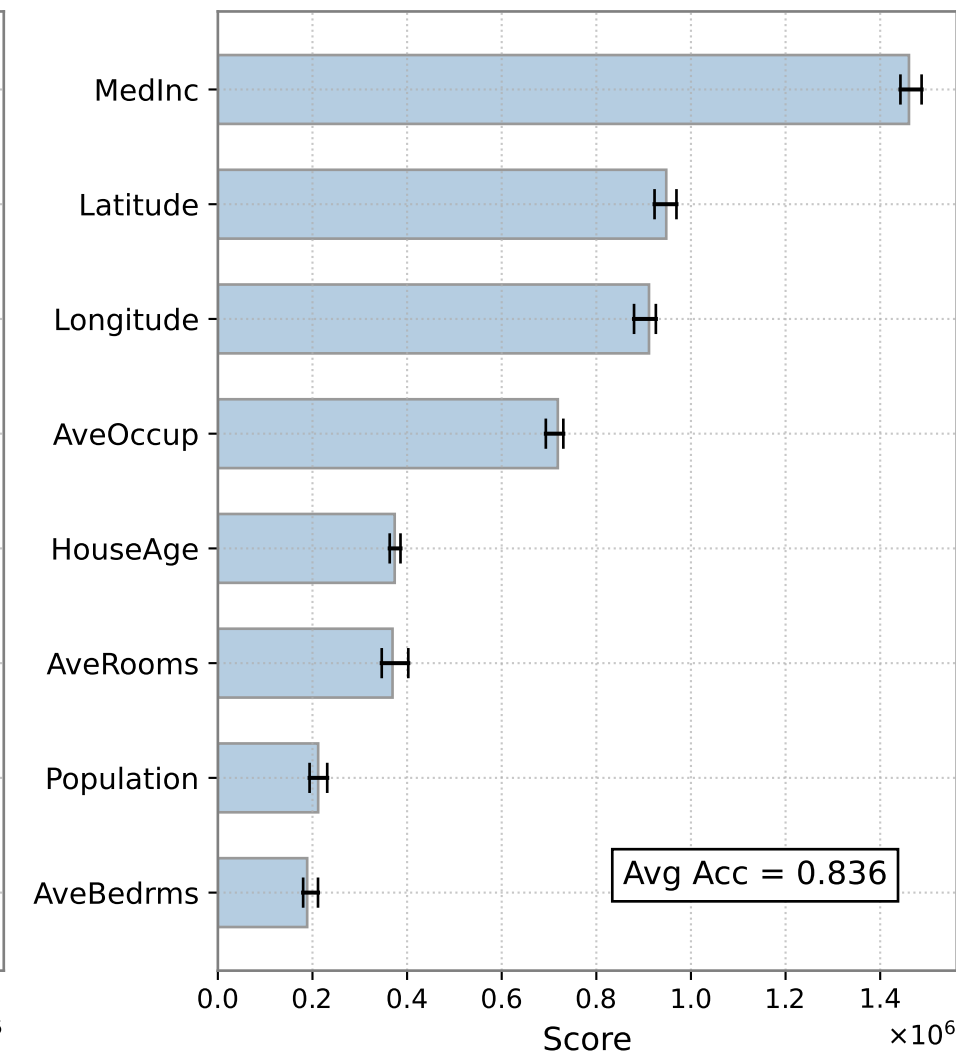
6 bins
