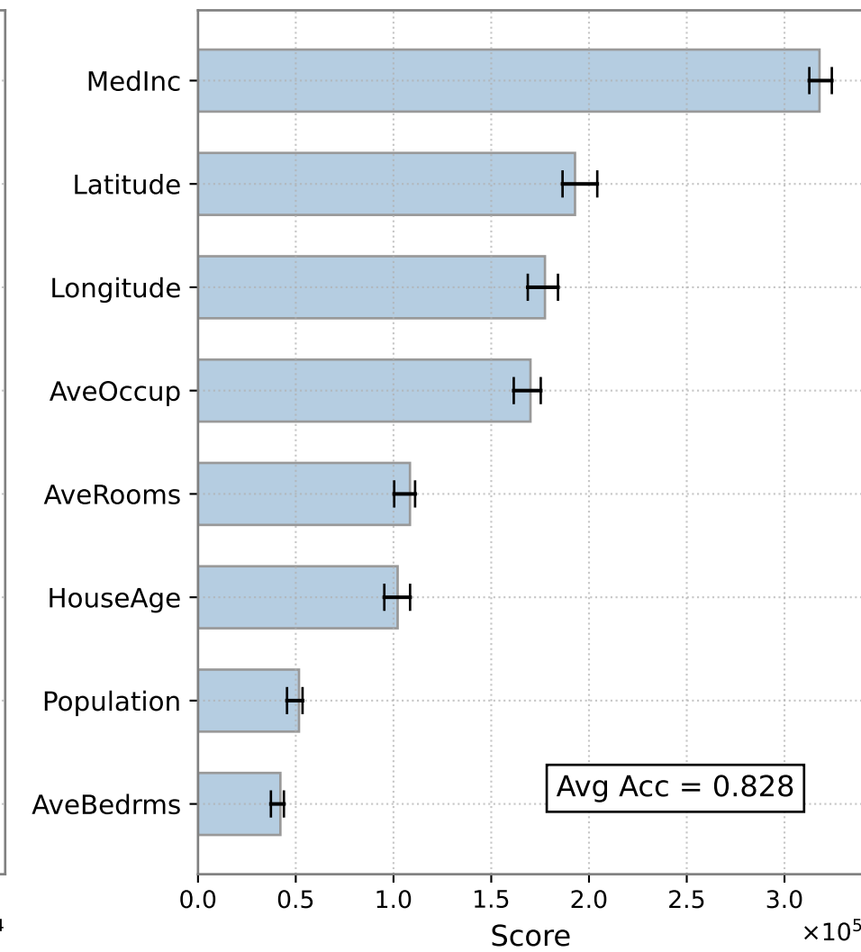
5 bins
