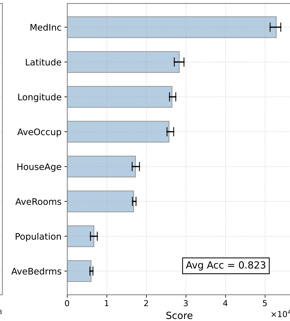
4 bins
