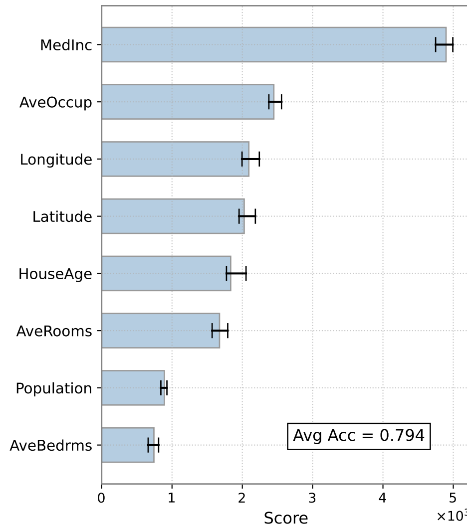
3 bins
