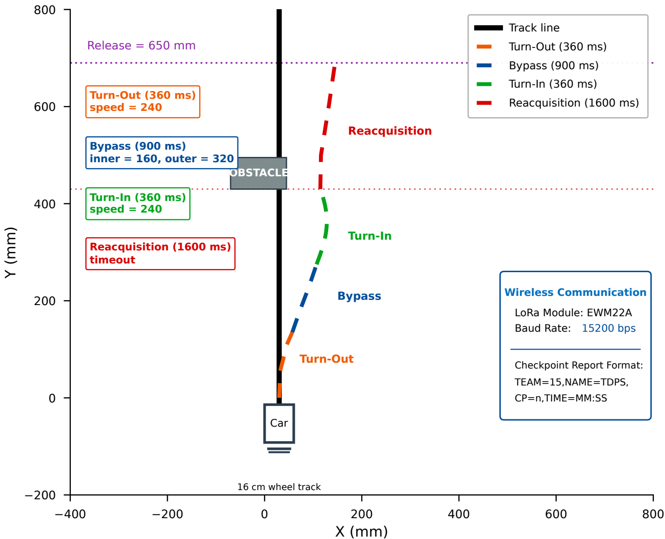
Fig. 7. Open-loop avoidance maneuver trajectory with four phases (simulated).
