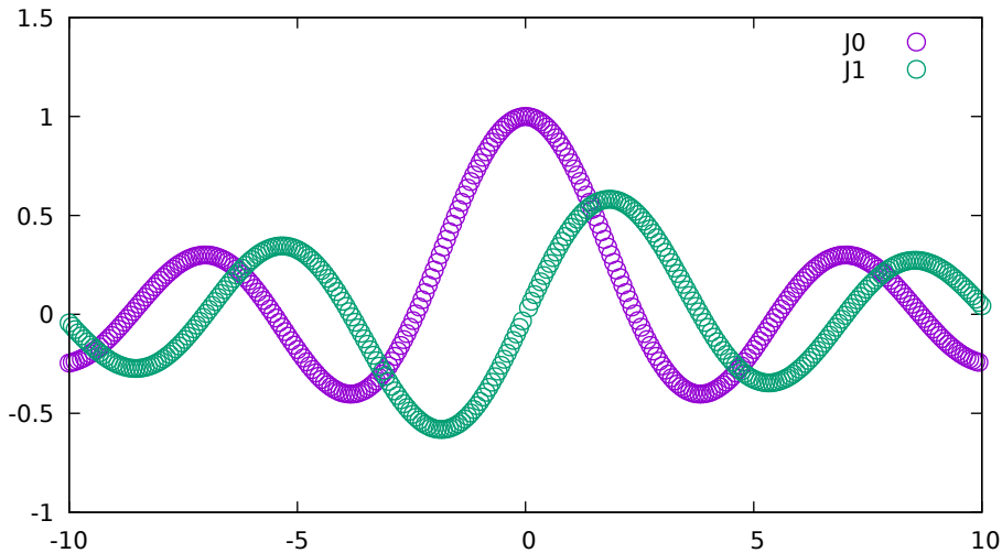
Bessel Functions
