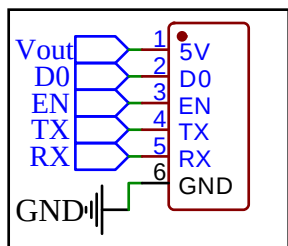
CONECTOR
