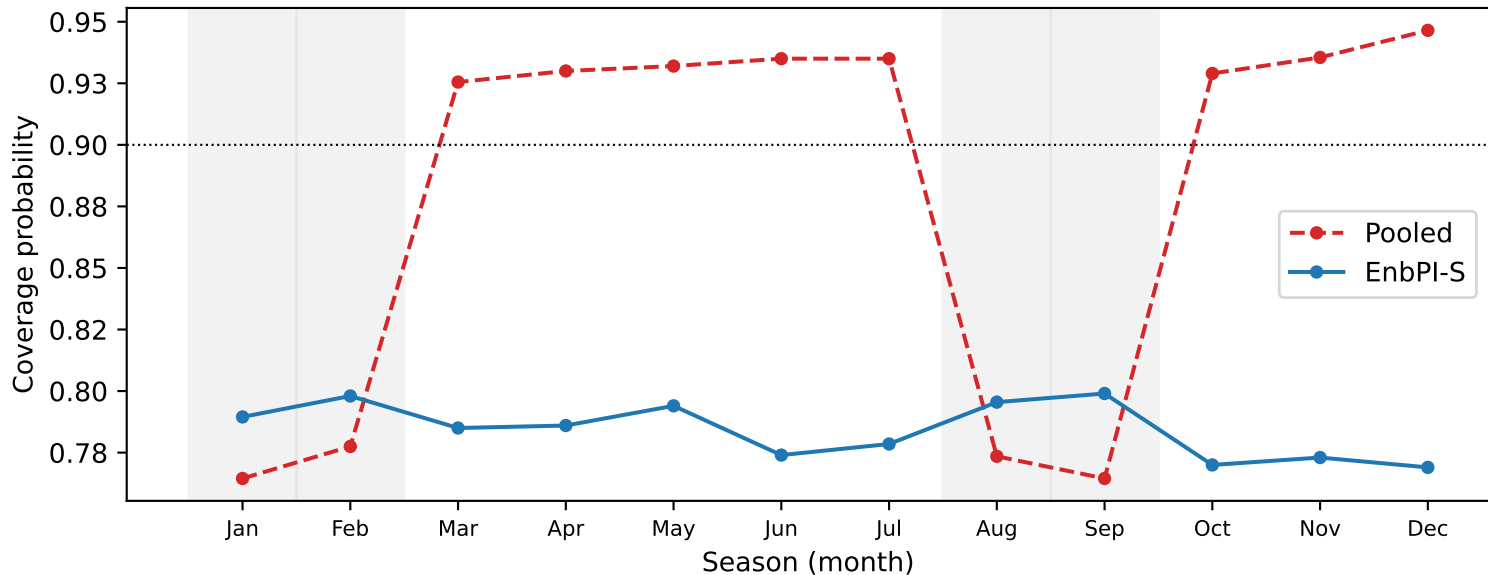
Per-season coverage ( T = 240 , \alpha = 0.10 )
