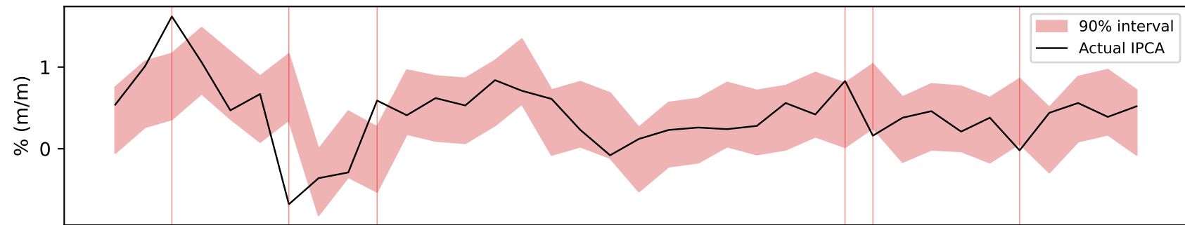
Pooled EnbPI
