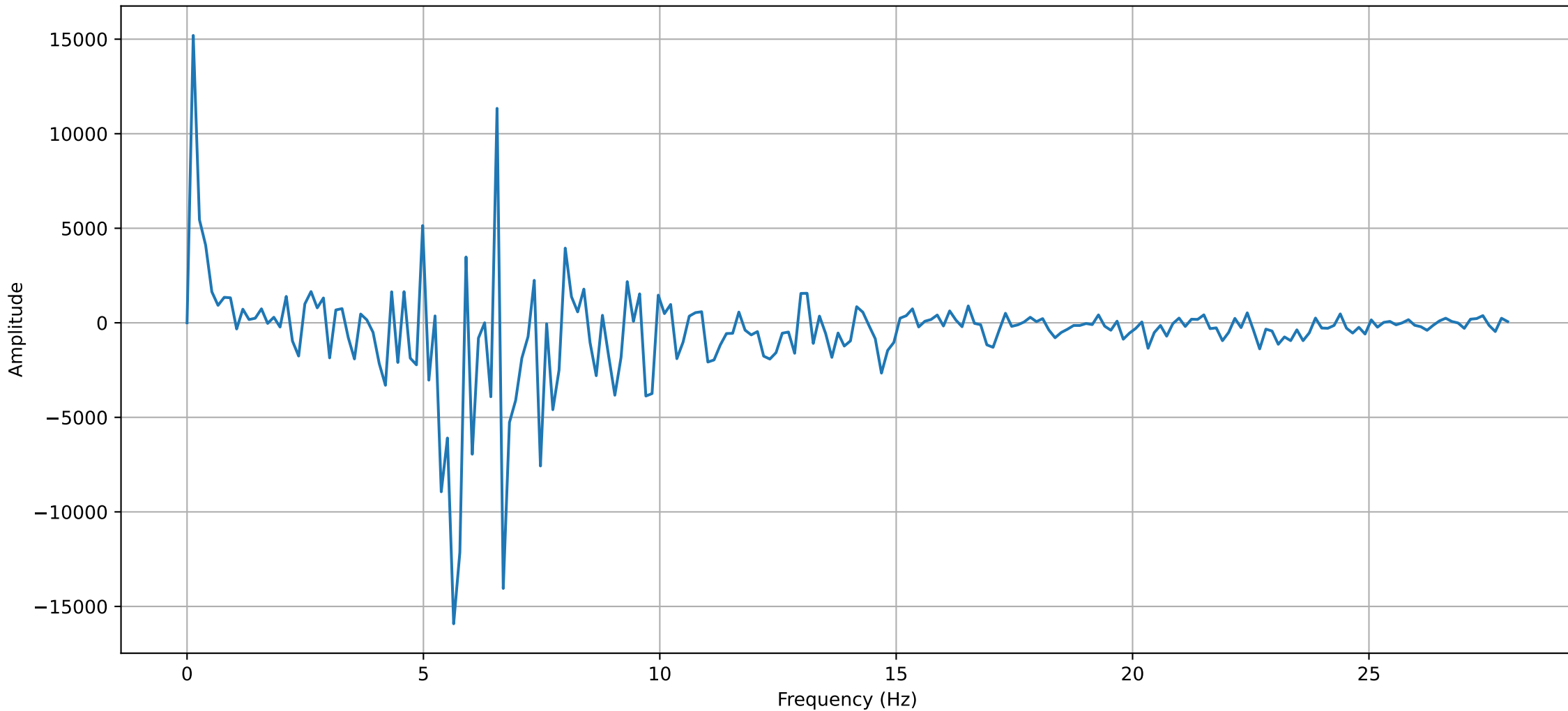
Frequency spectrum of the Pressure oscillation (30mm 90° 3.0)
