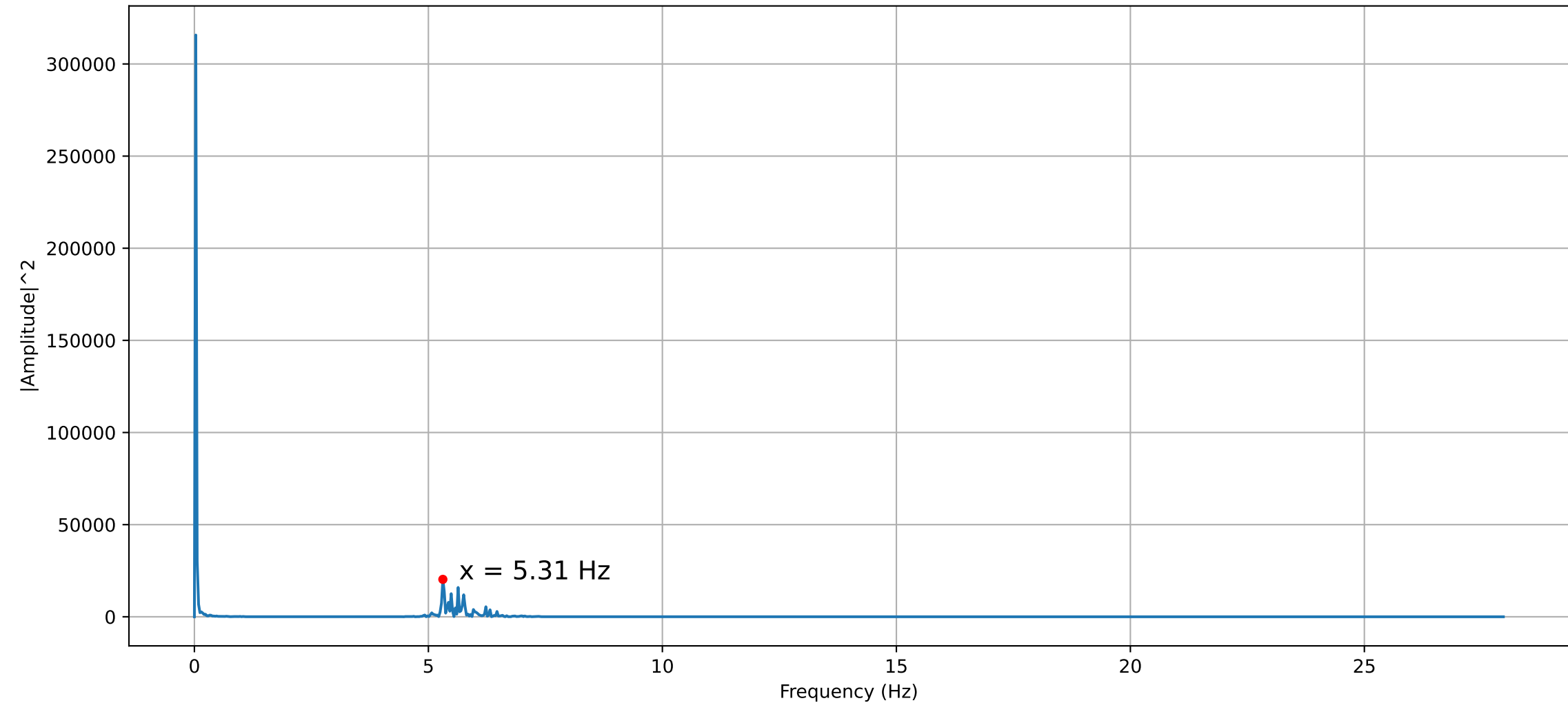
Frequency Power Spectrum of Pressure Oscillation (20mm 90° 1.0)
