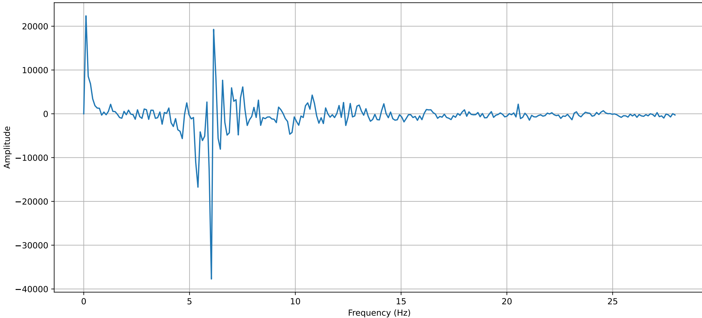
Frequency spectrum of the Pressure oscillation (30mm 90° 2.0)
