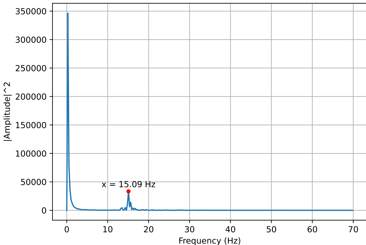
Frequency Power Spectrum of Pressure Oscillation (30mm Vertical 2.0)
