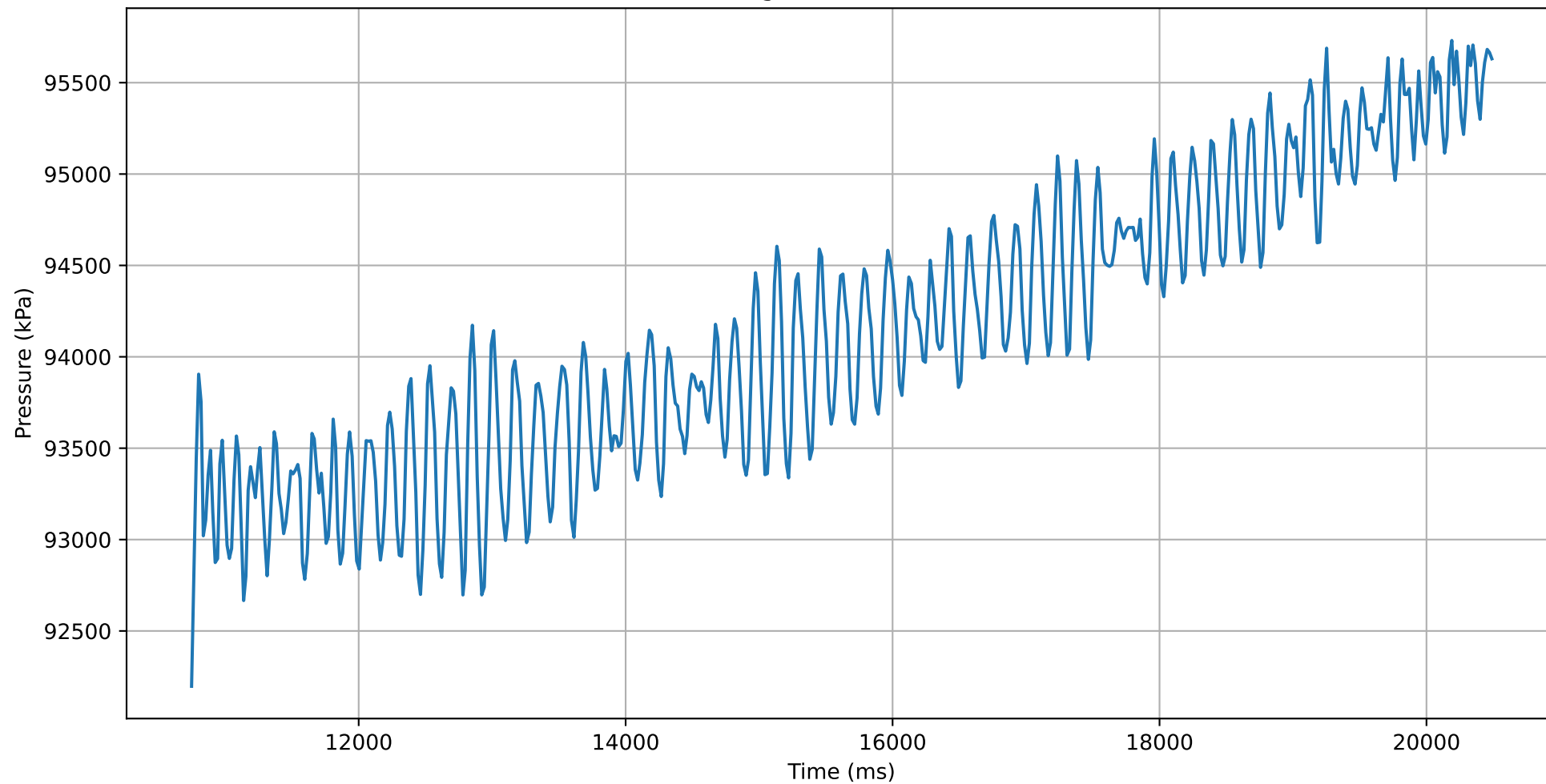
Pressure change in time (30mm 70° 1.0)
