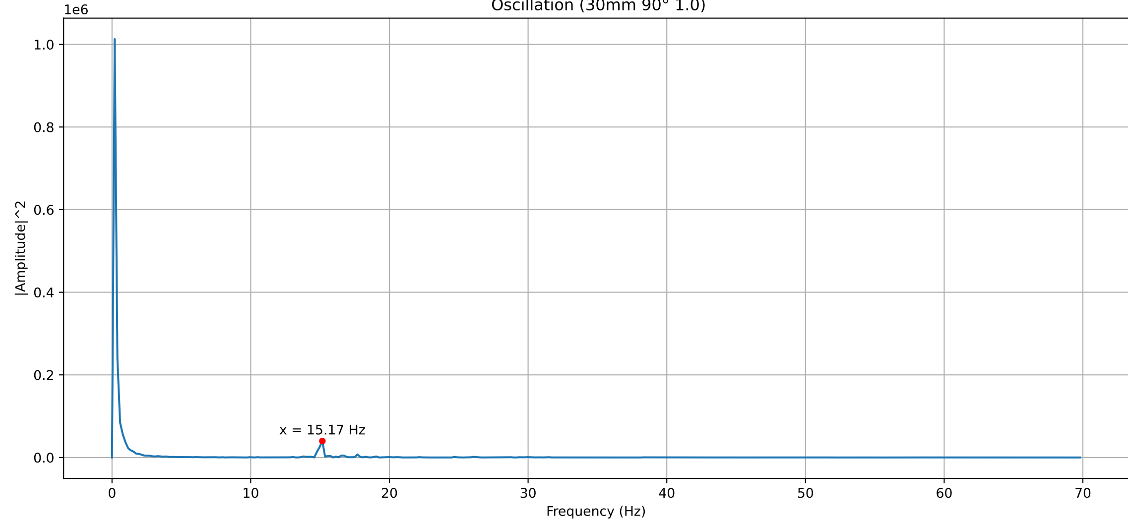
Frequency Power Spectrum of Pressure Oscillation (30mm 90° 1.0)
