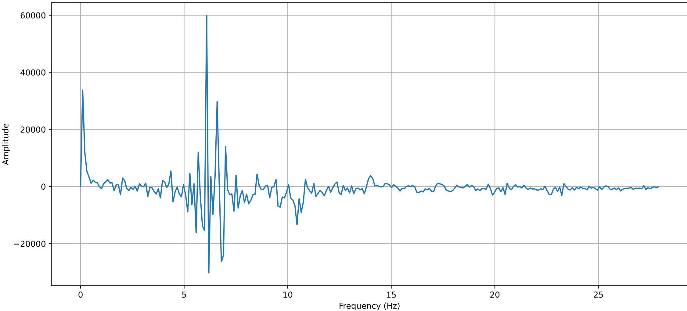
Frequency spectrum of the Pressure oscillation (30mm 70° 1.0)
