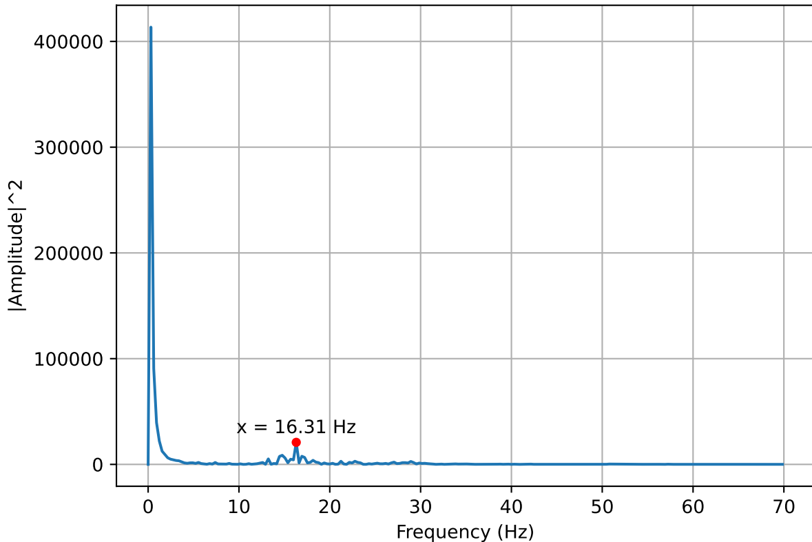
Frequency Power Spectrum of Pressure Oscillation (30mm 60° 1.0)
