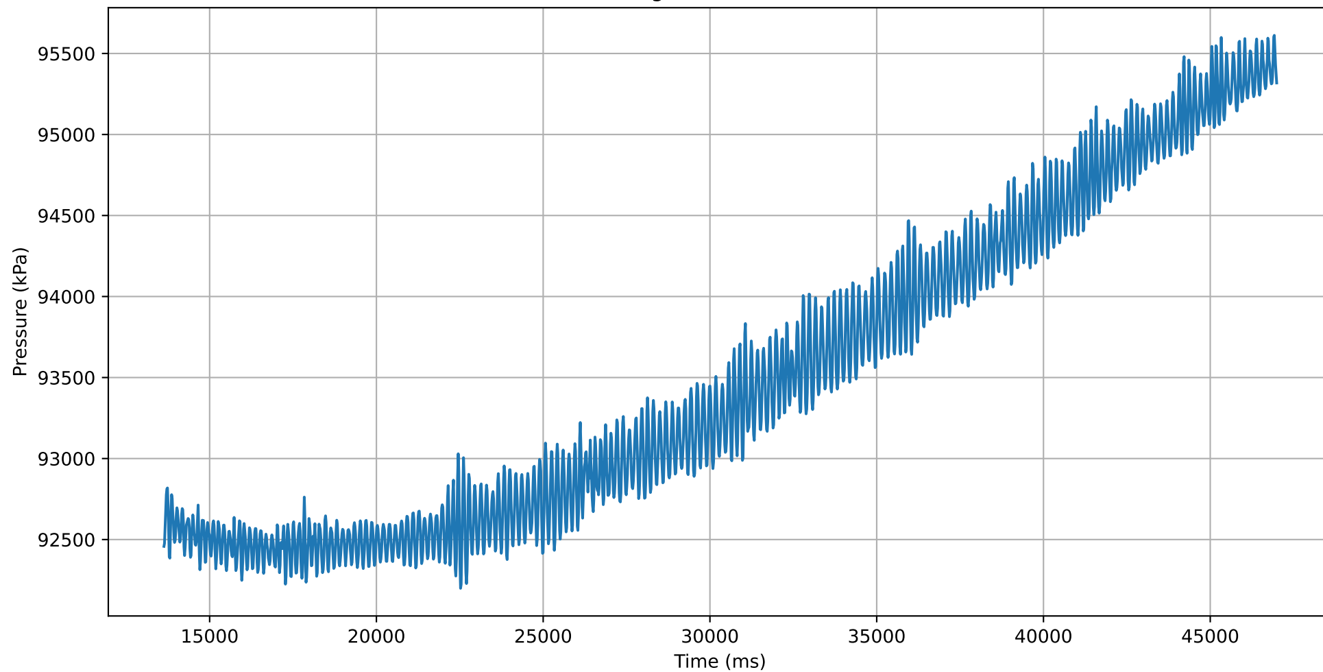
Pressure change in time (20mm 90° 1.0)
