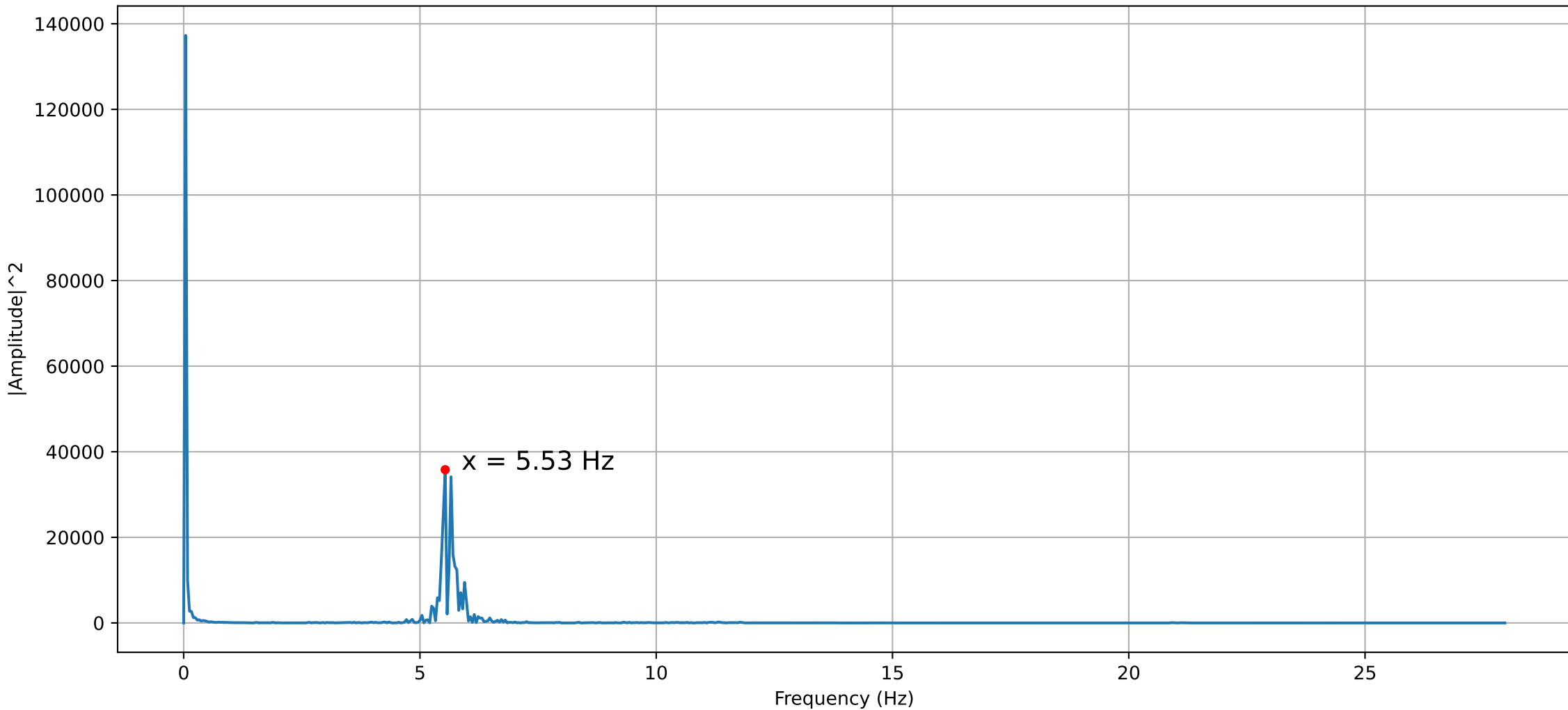
Frequency Power Spectrum of Pressure Oscillation (20mm 70° 1.0)
