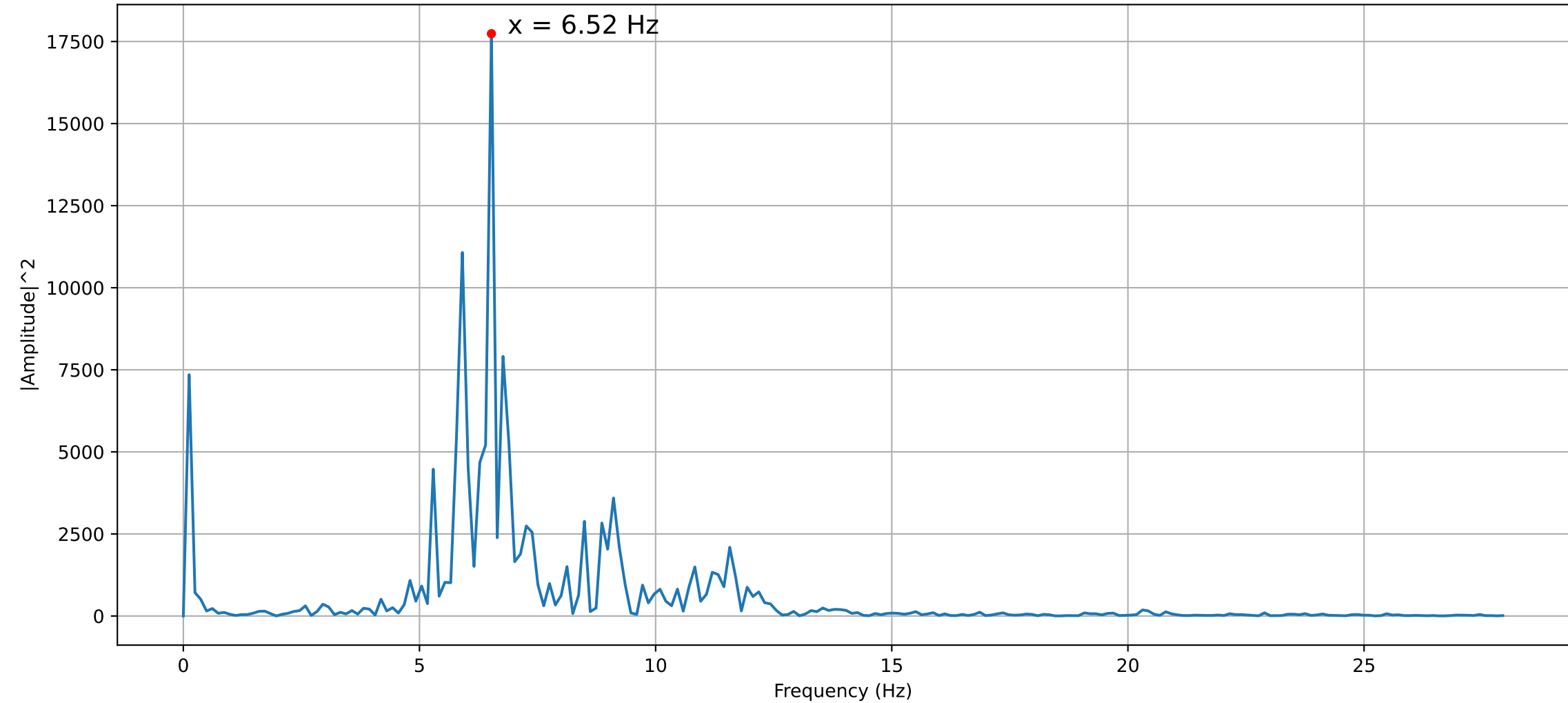
Frequency Power Spectrum of Pressure Oscillation (30mm 60° 1.0)
