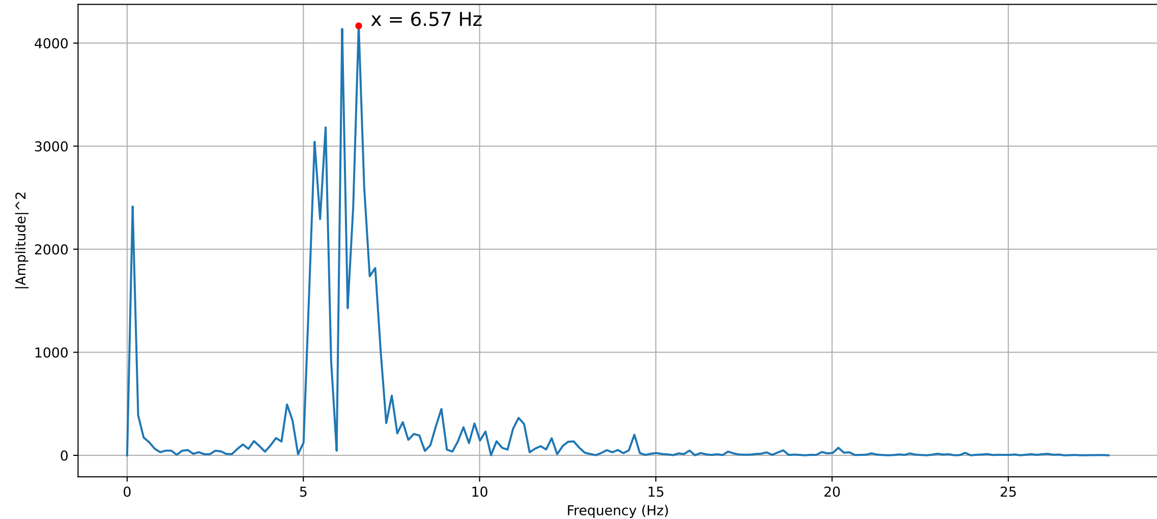
Frequency Power Spectrum of Pressure Oscillation (30mm 90° 4.0)
