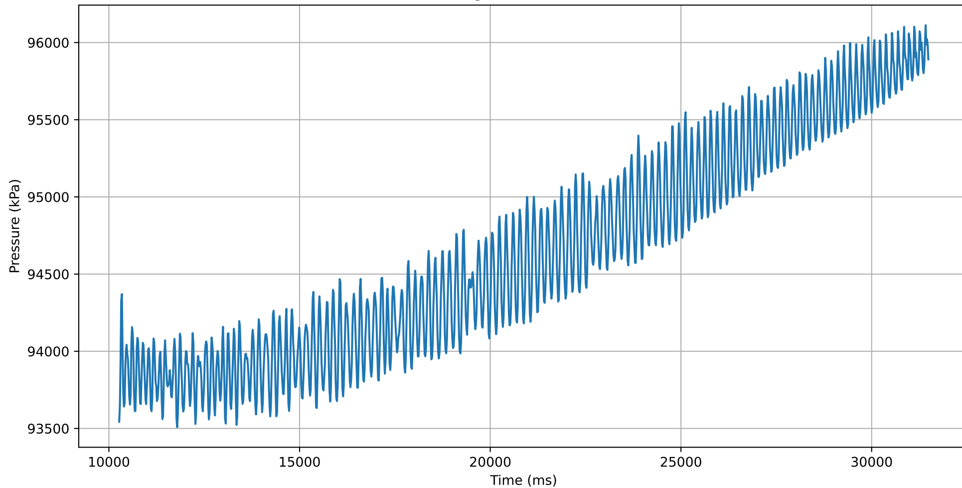
Pressure change in time (20mm 45° 1.0)
