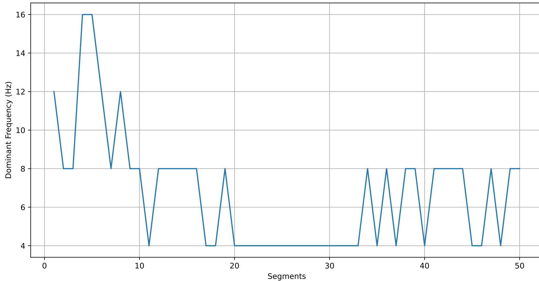
Dominant Frequencies in the Segments (30mm 90° 1.0)
