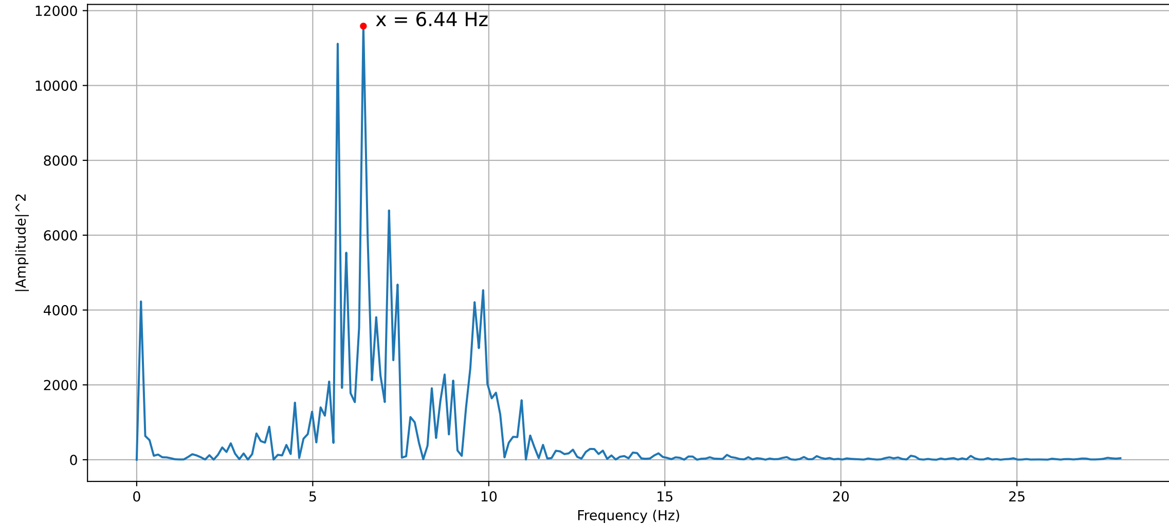
Frequency Power Spectrum of Pressure Oscillation (30mm 45° 1.0)
