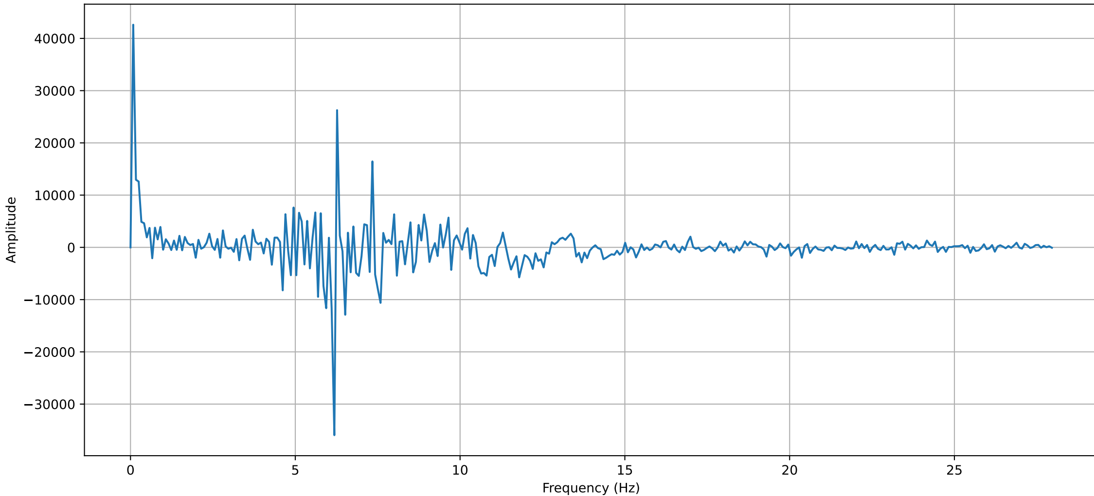
Frequency spectrum of the Pressure oscillation (30mm 90° 1.1)
