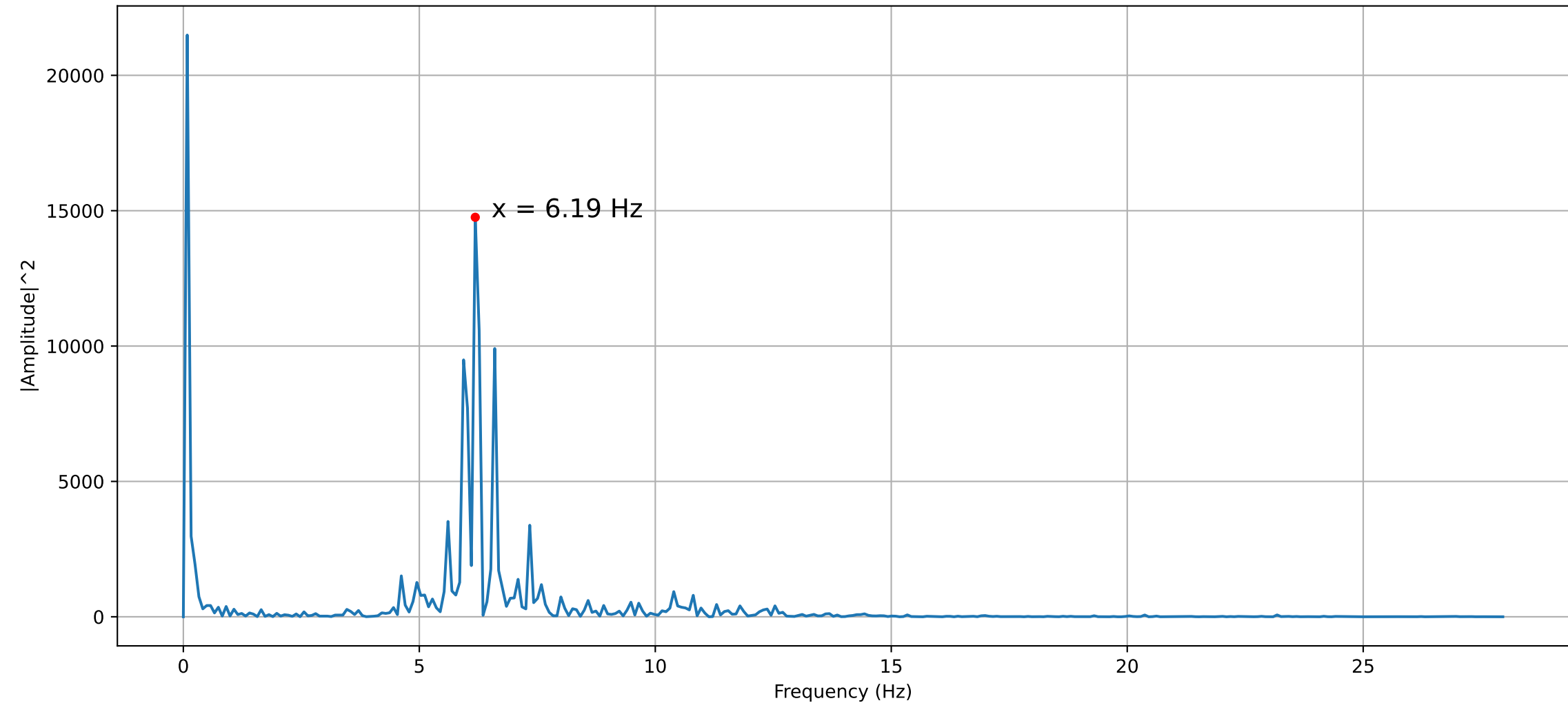
Frequency Power Spectrum of Pressure Oscillation (30mm 90° 1.1)
