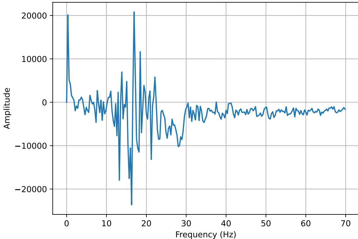
Frequency spectrum of the Pressure oscillation (30mm 60° 1.0)
