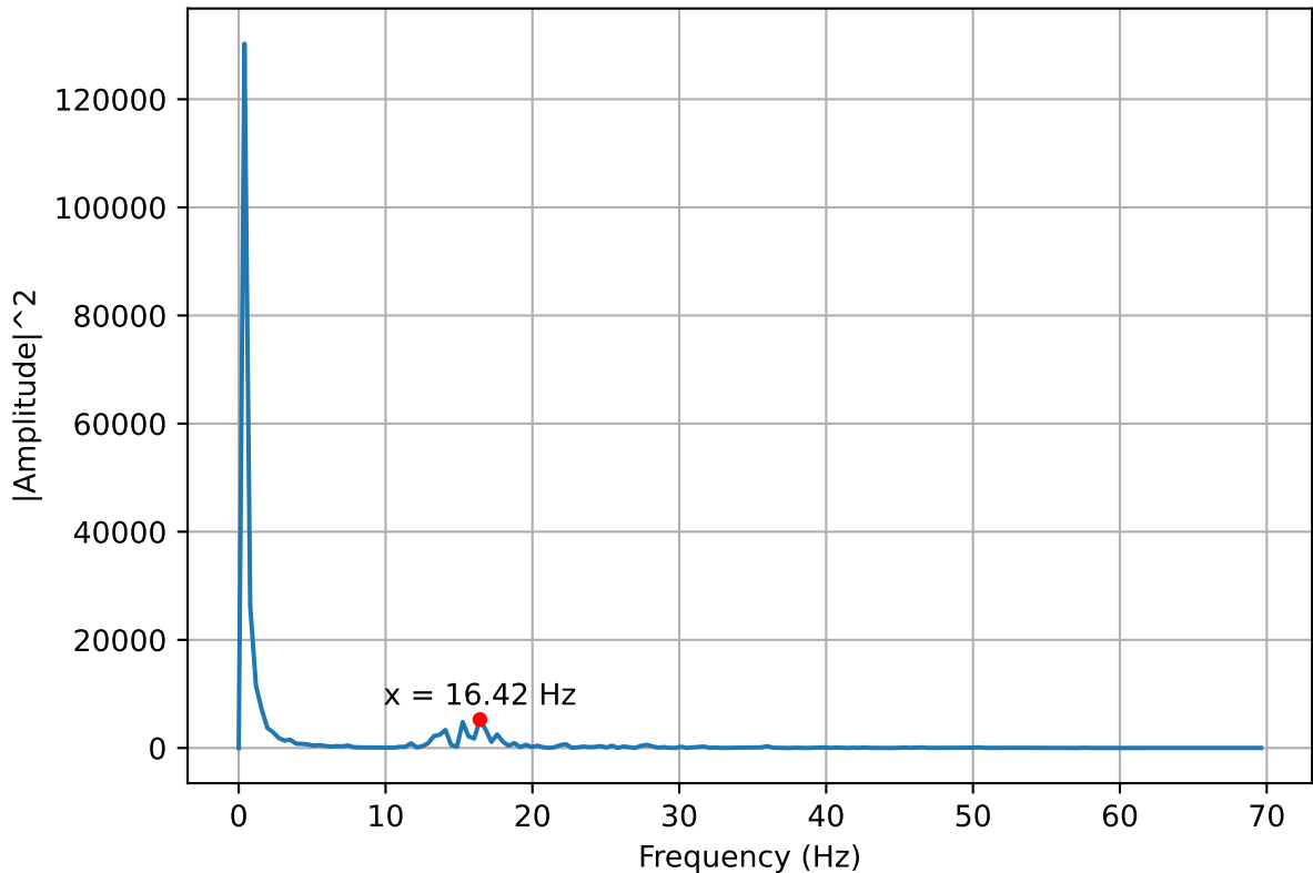
Frequency Power Spectrum of Pressure Oscillation (30mm Vertical 4.0)
