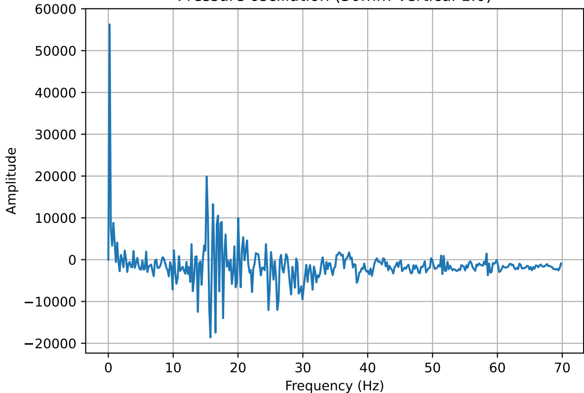
Frequency spectrum of the Pressure oscillation (30mm Vertical 1.0)
