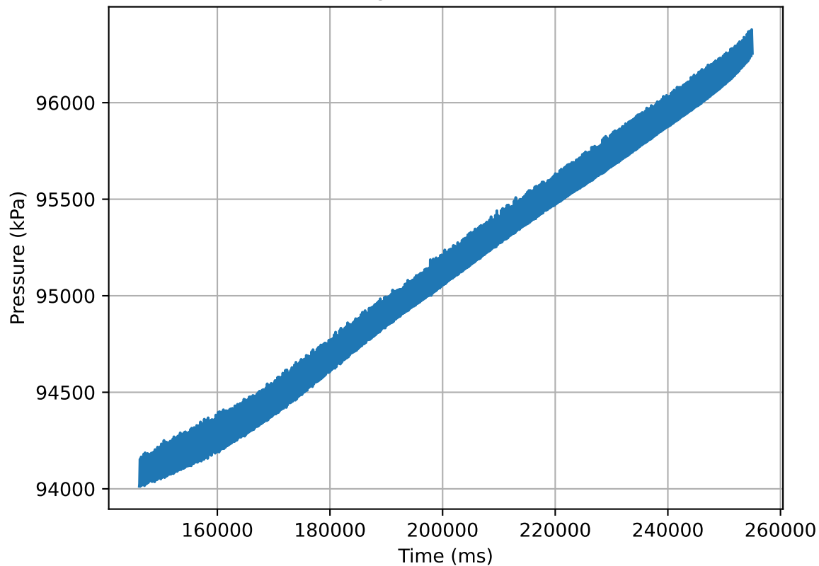
Pressure change in time (10mm 45° 1.0)
