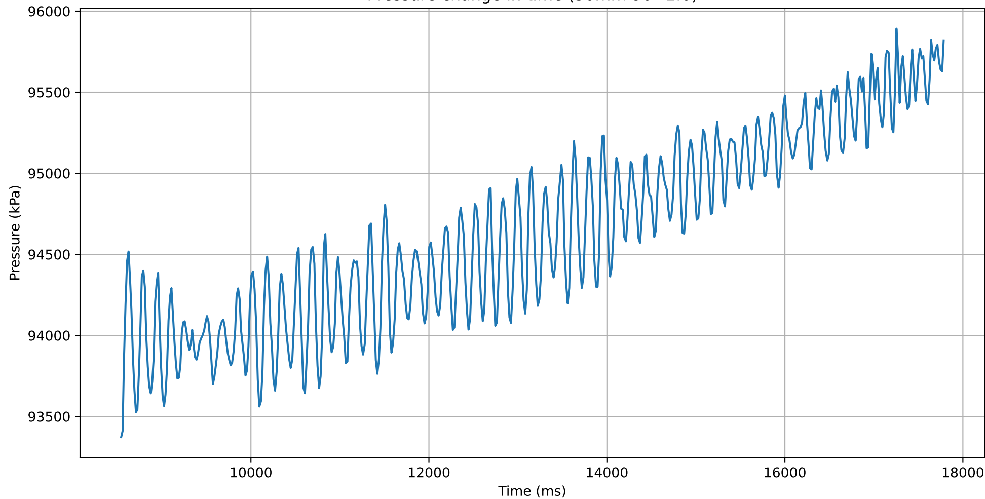
Pressure change in time (30mm 90° 2.0)
