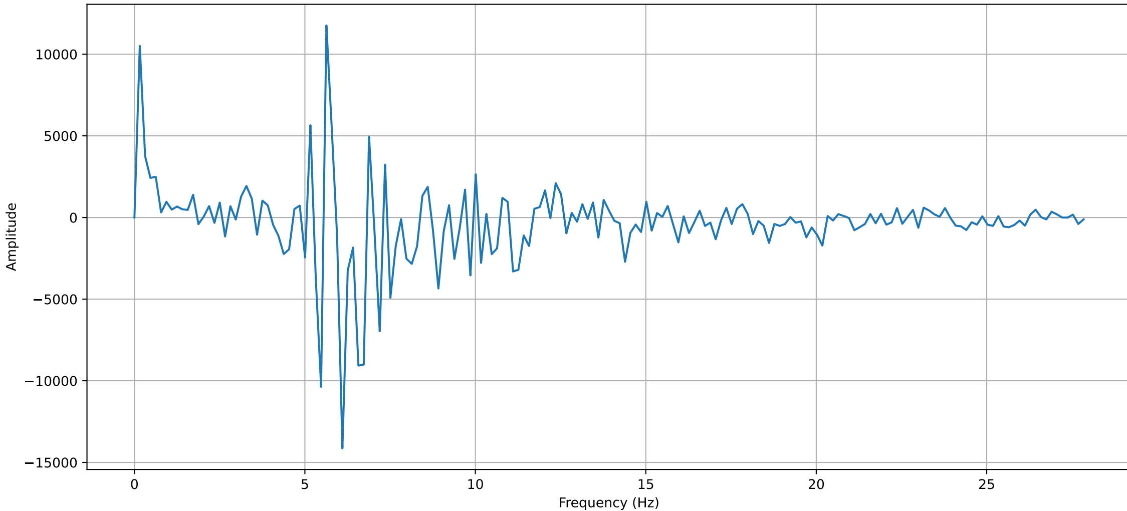
Frequency spectrum of the Pressure oscillation (30mm 90° 4.0)
