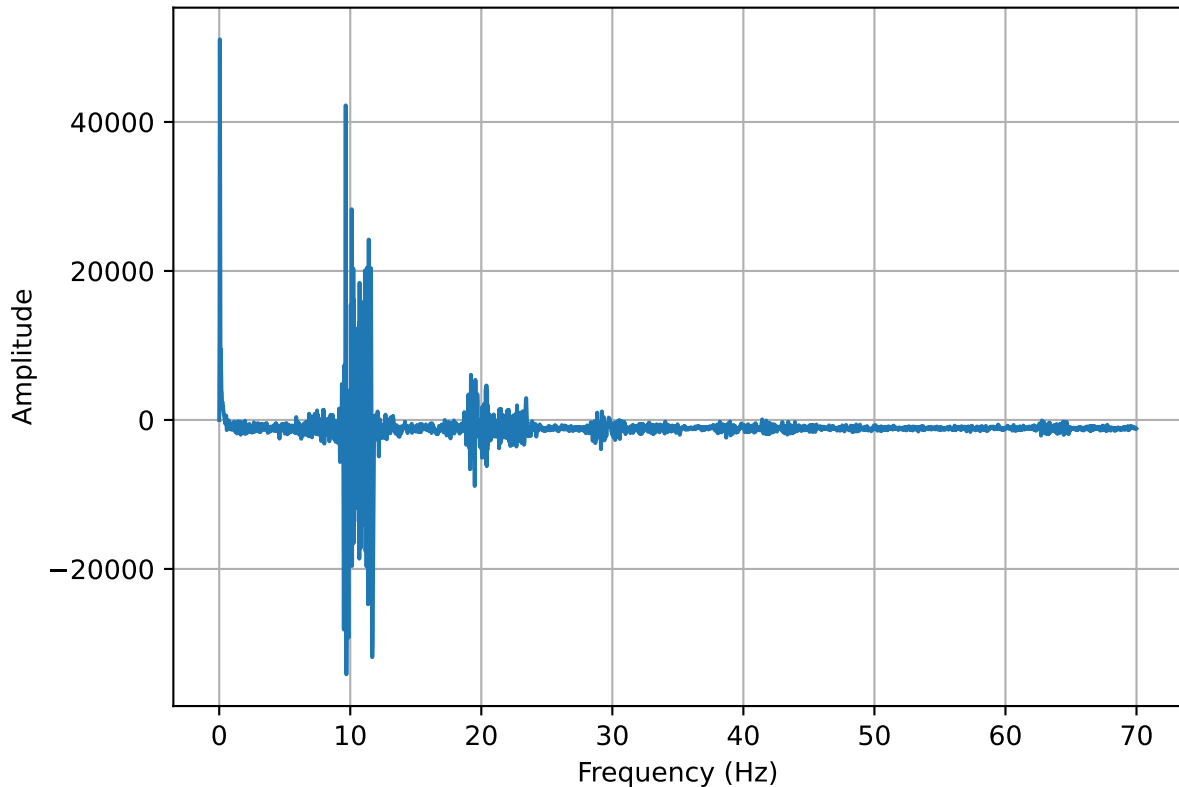
Frequency spectrum of the Pressure oscillation (10mm 45° 1.0)
