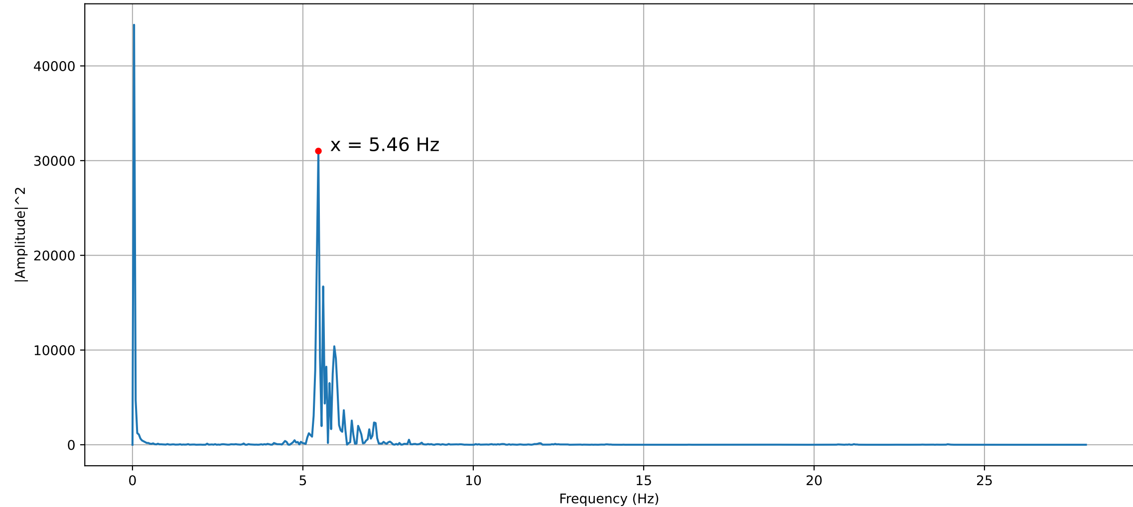
Frequency Power Spectrum of Pressure Oscillation (20mm 45° 1.0)
