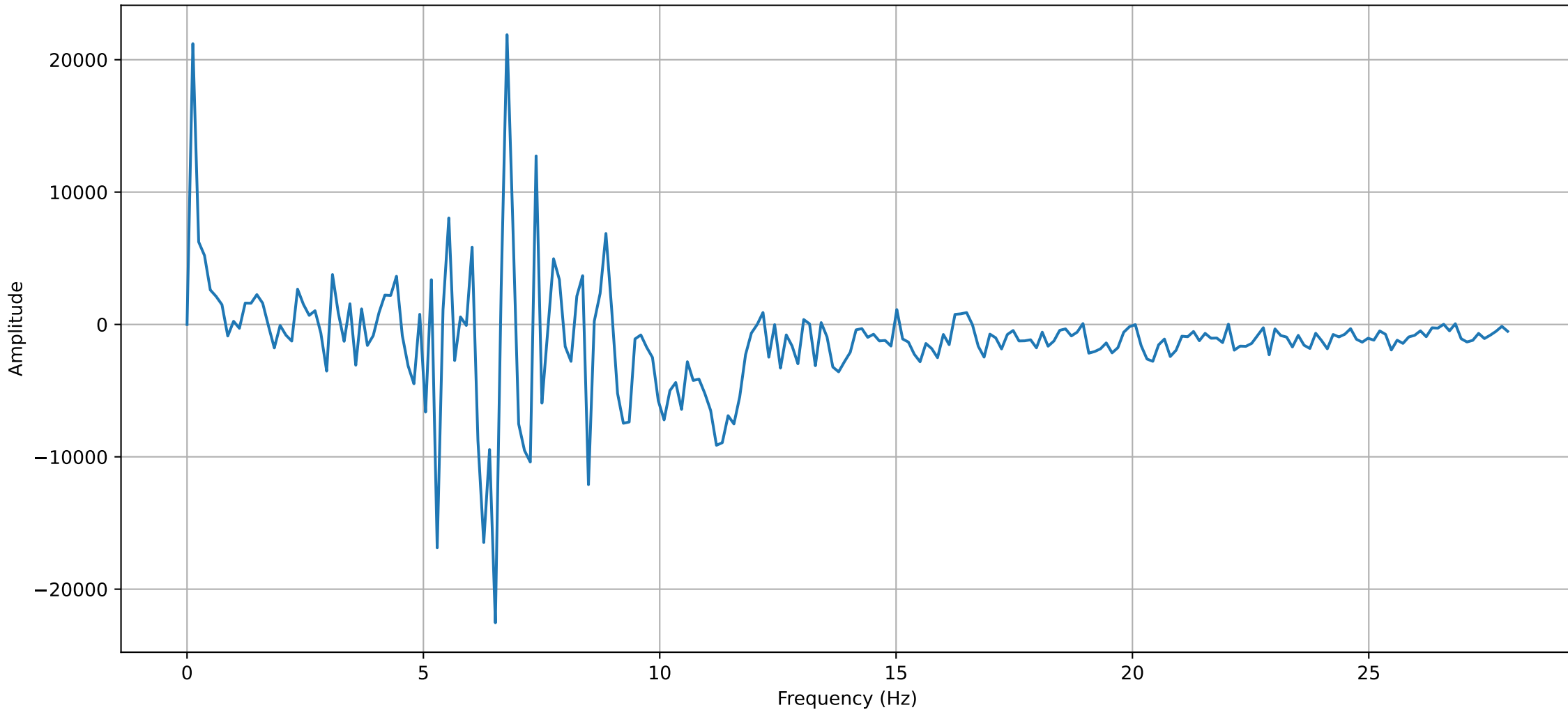
Frequency spectrum of the Pressure oscillation (30mm 60° 1.0)
