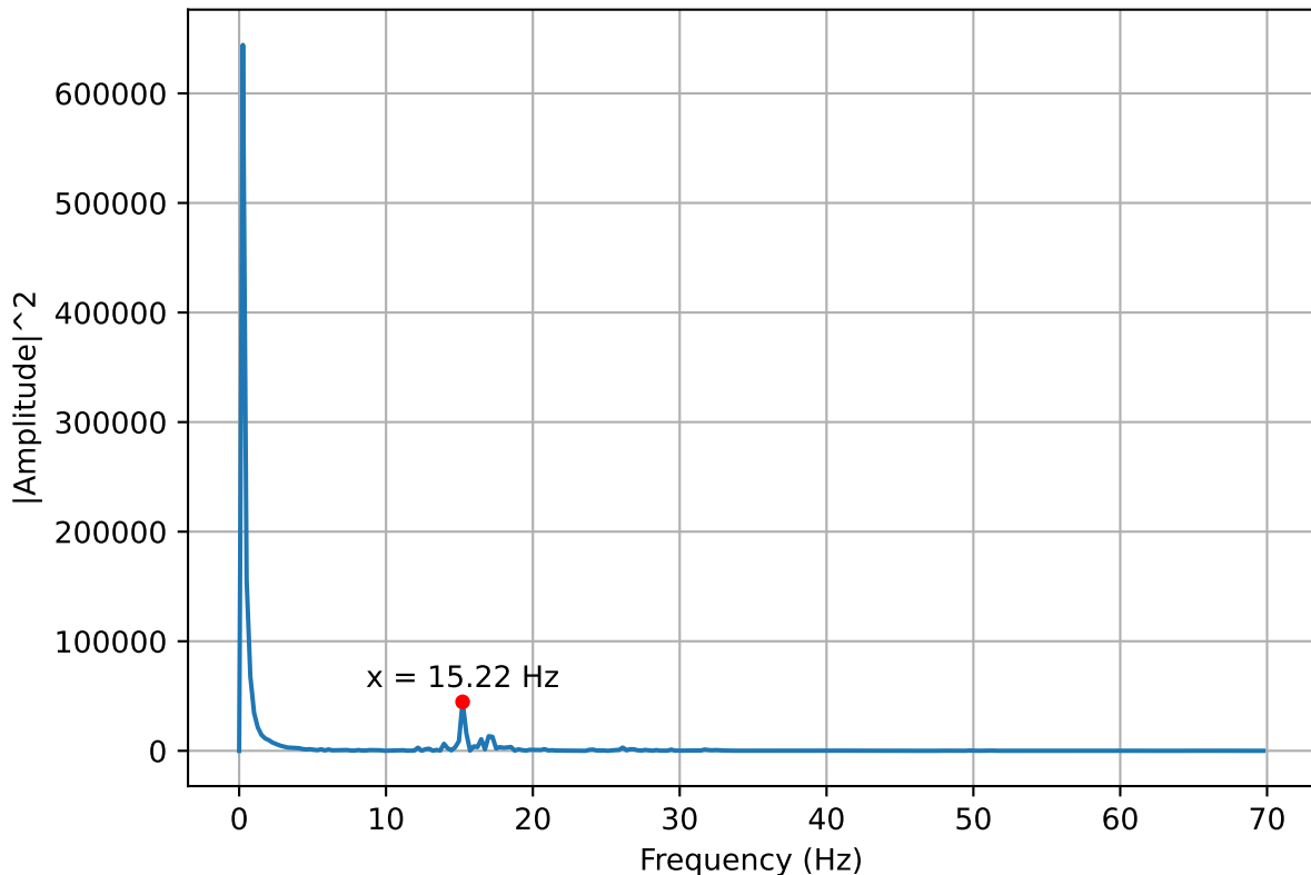
Frequency Power Spectrum of Pressure Oscillation (30mm 70° 1.0)
