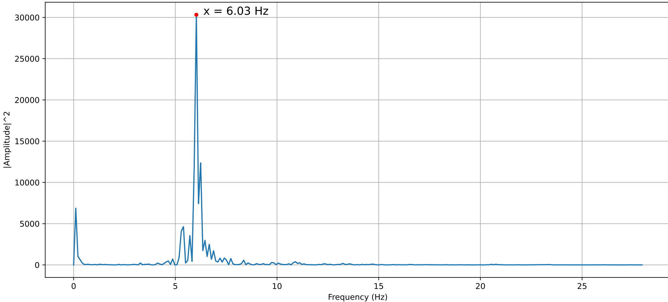
Frequency Power Spectrum of Pressure Oscillation (30mm 90° 2.0)
