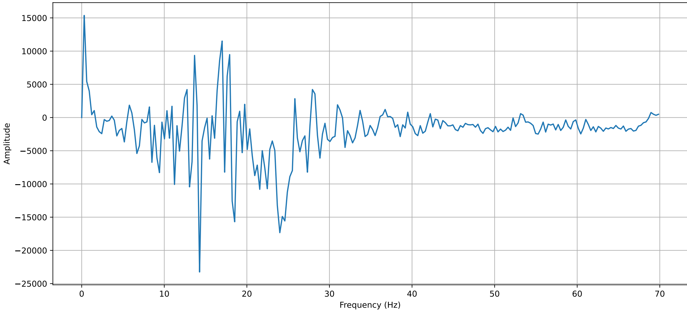
Frequency spectrum of the Pressure oscillation (30mm 45° 1.0)
