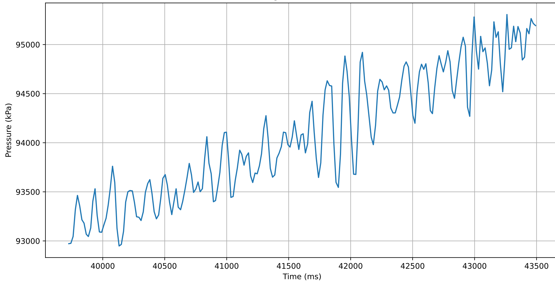
Pressure change in time (40mm 90° 1.0)
