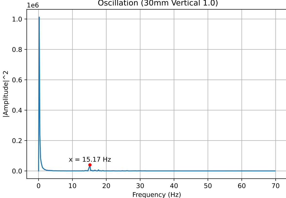
Frequency Power Spectrum of Pressure Oscillation (30mm Vertical 1.0)
