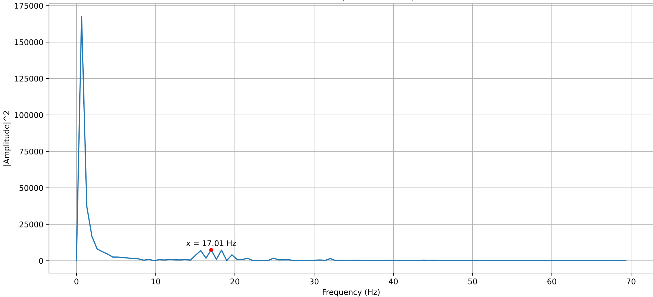
Frequency Power Spectrum of Pressure Oscillation (40mm 90° 1.0)
