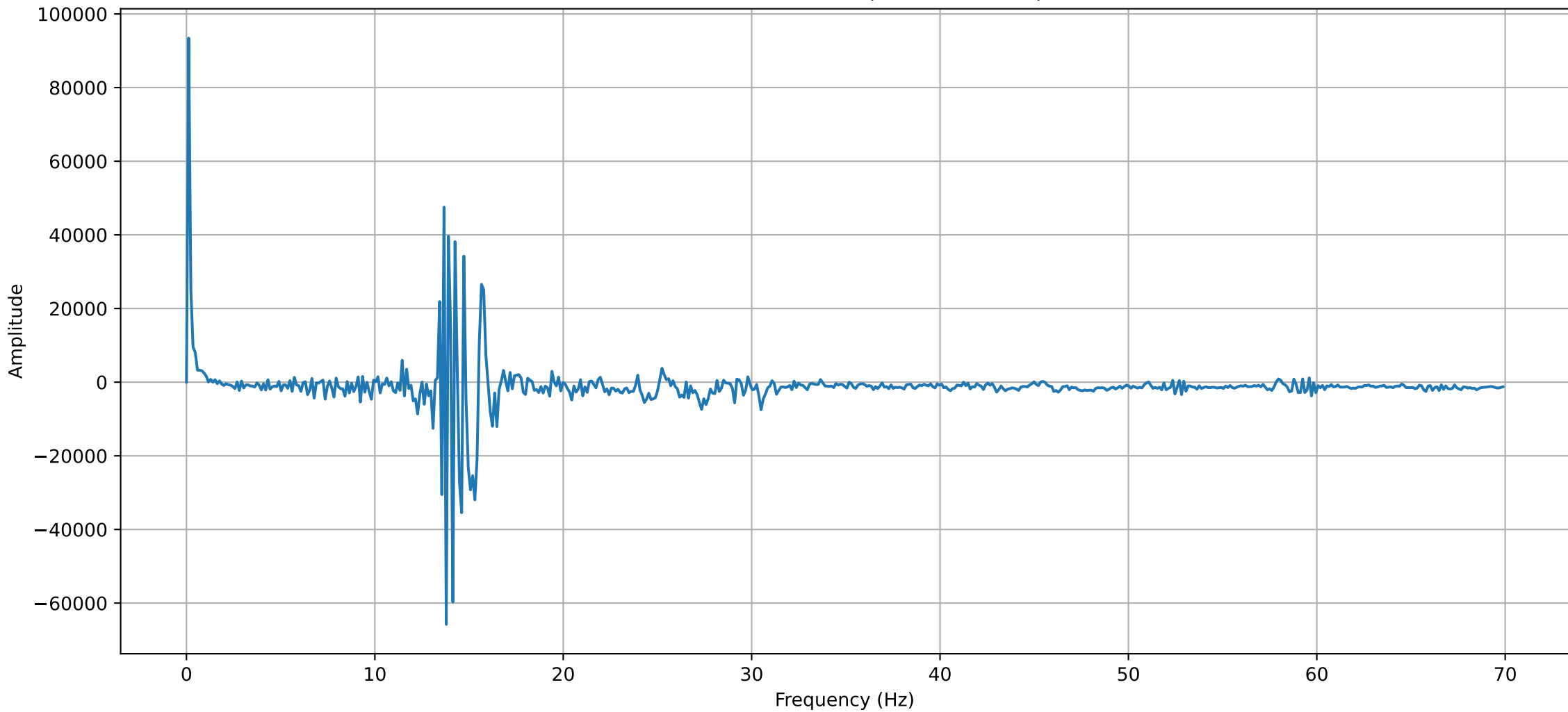
Frequency spectrum of the Pressure oscillation (20mm 60° 1.0)
