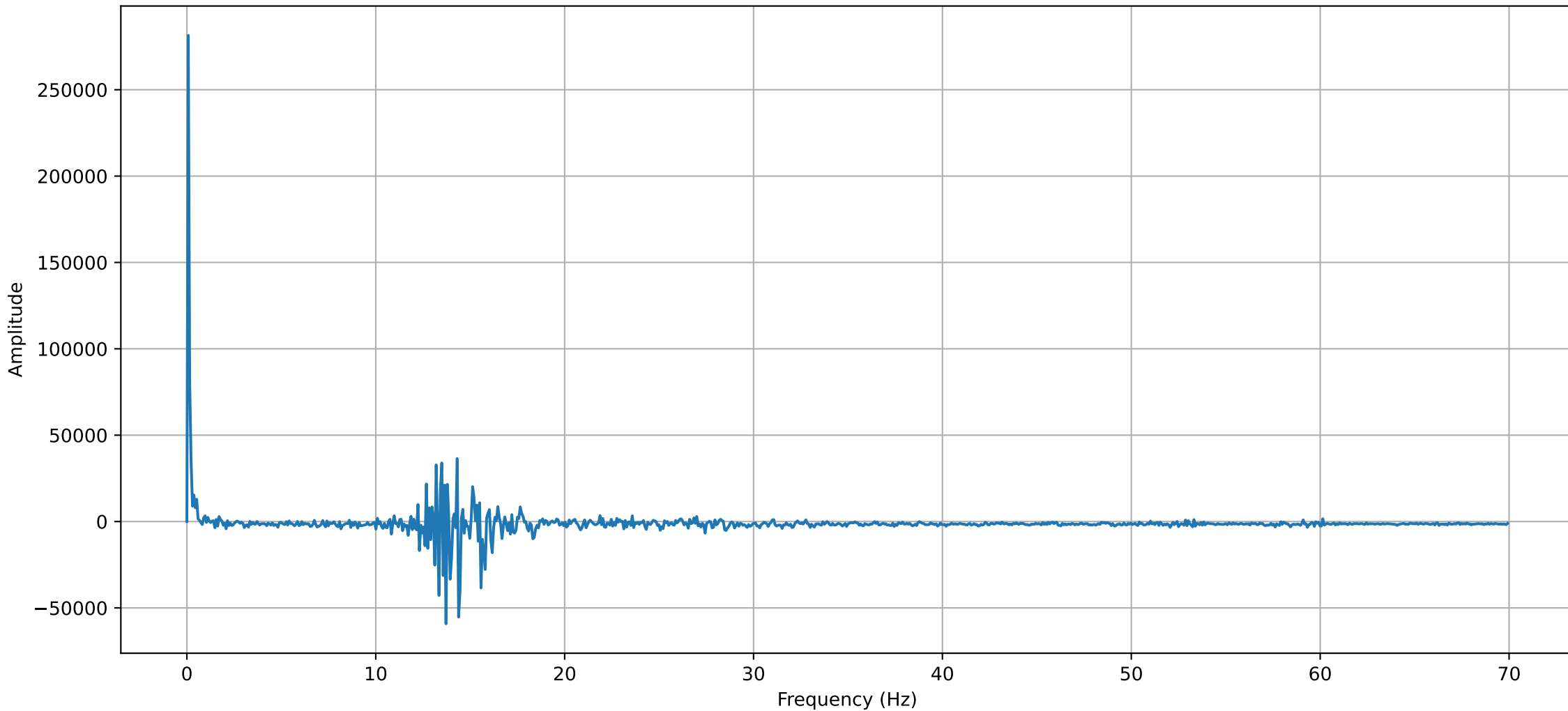
Frequency spectrum of the Pressure oscillation (20mm 90° 1.0)
