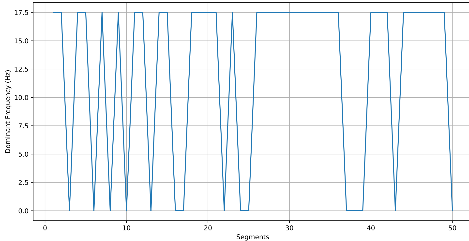
Dominant Frequencies in the Segments (30mm Vertical 3.0)
