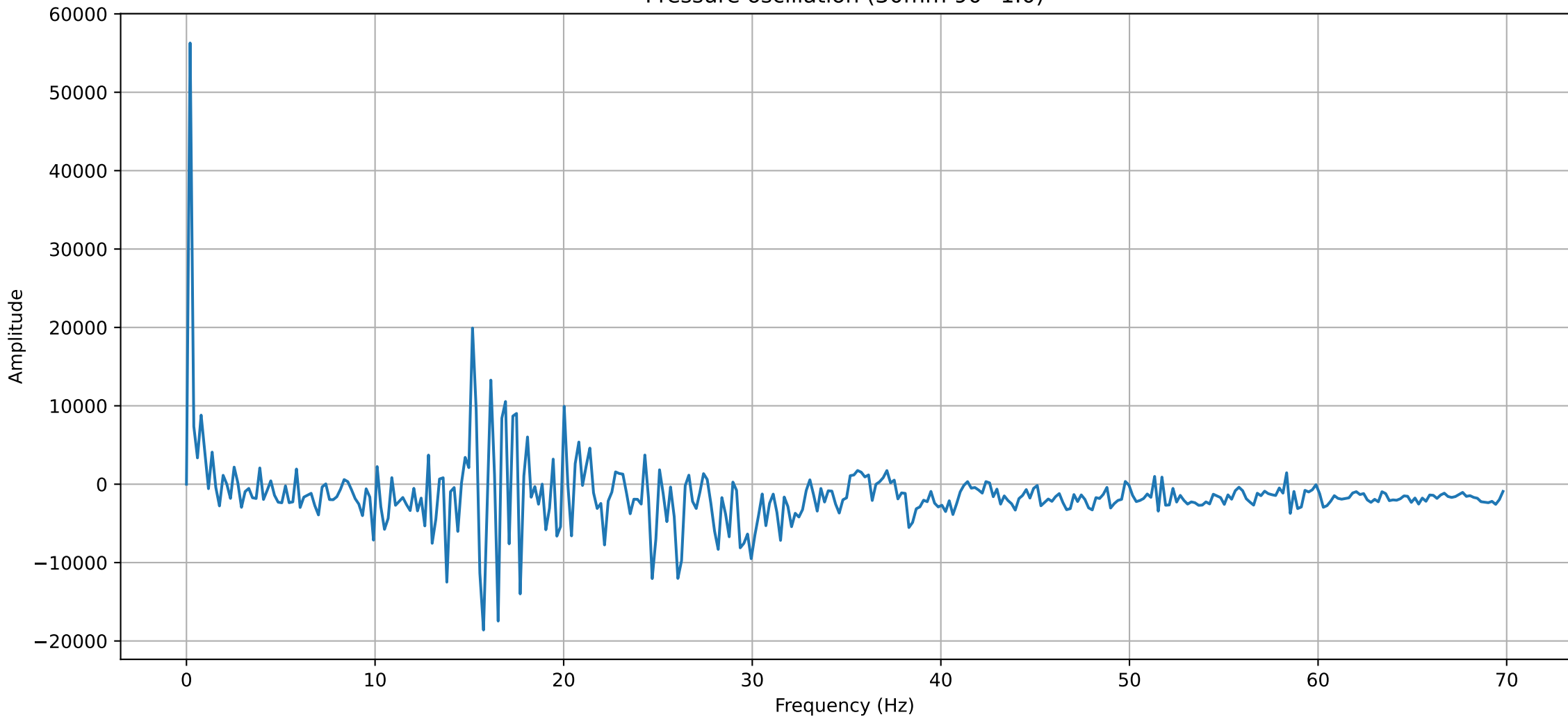
Frequency spectrum of the Pressure oscillation (30mm 90° 1.0)
