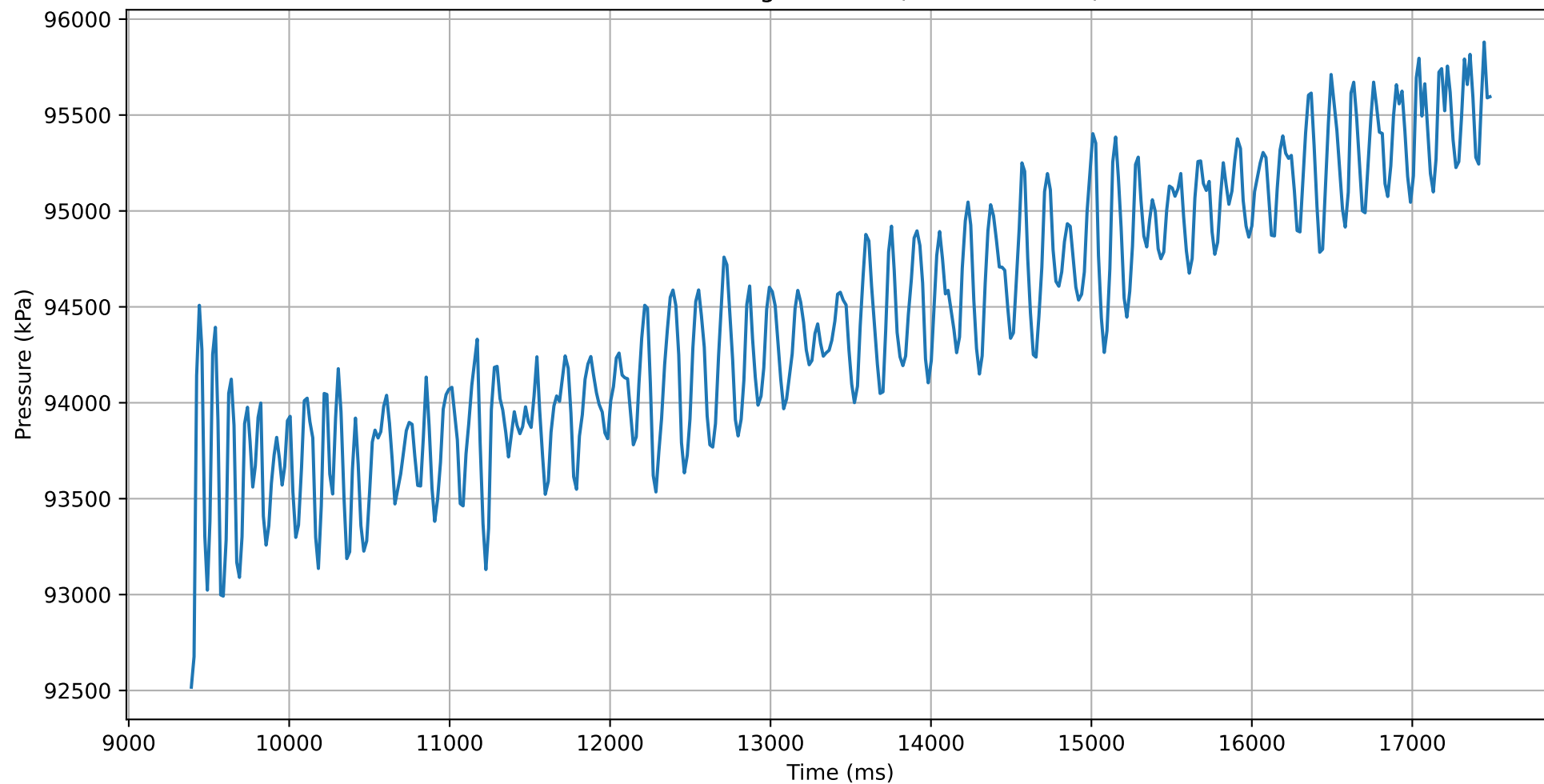
Pressure change in time (30mm 45° 1.0)
