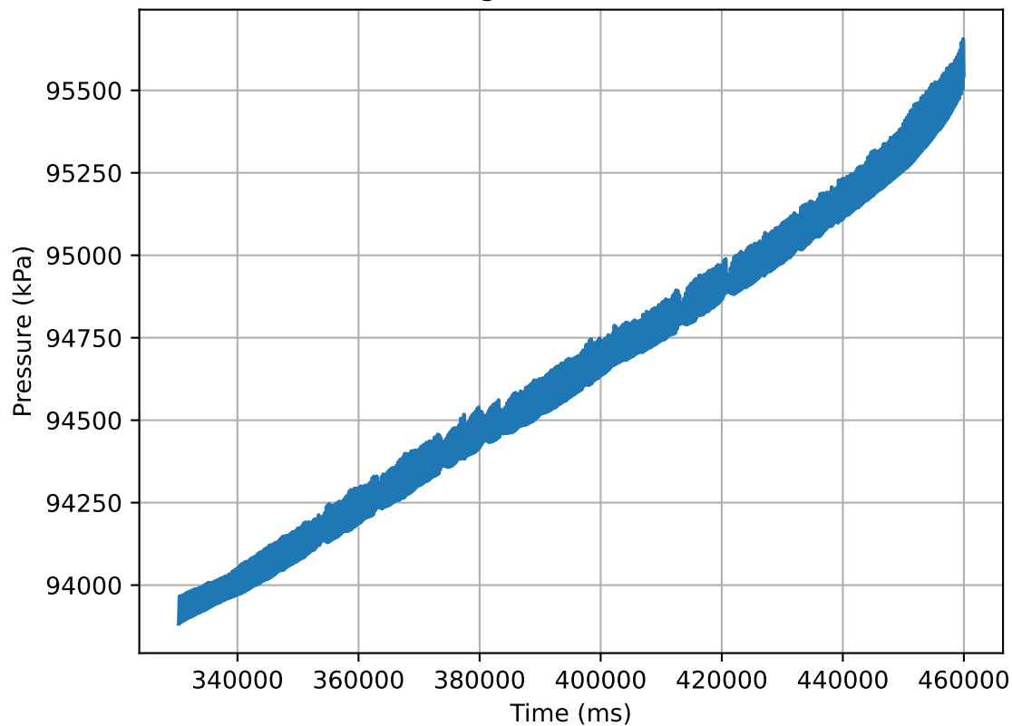
Pressure change in time (10mm 90° 1.0)
