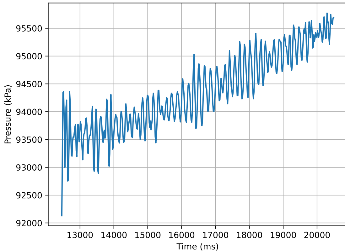
Pressure change in time (30mm 60° 1.0)
