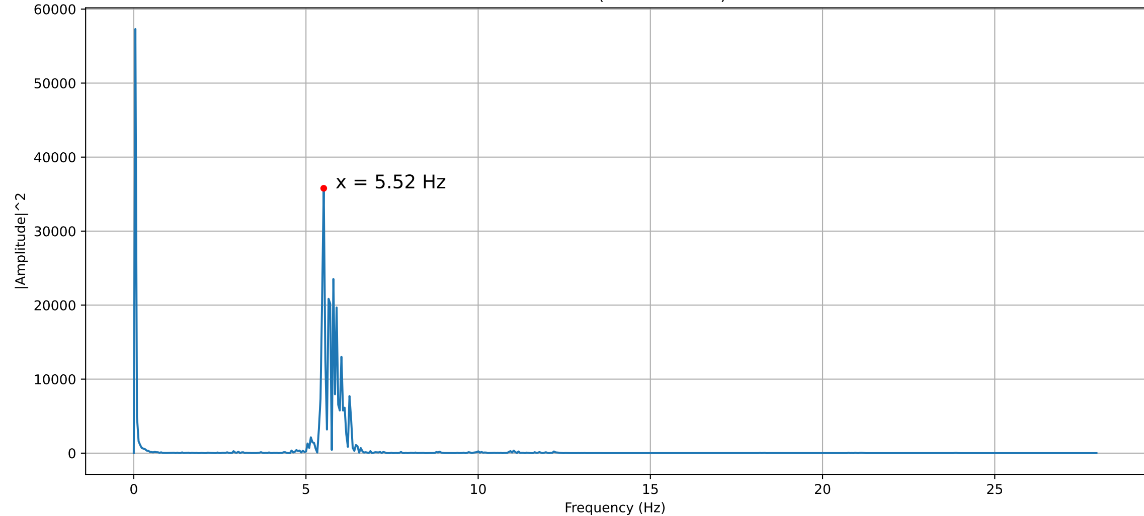
Frequency Power Spectrum of Pressure Oscillation (20mm 60° 1.0)
