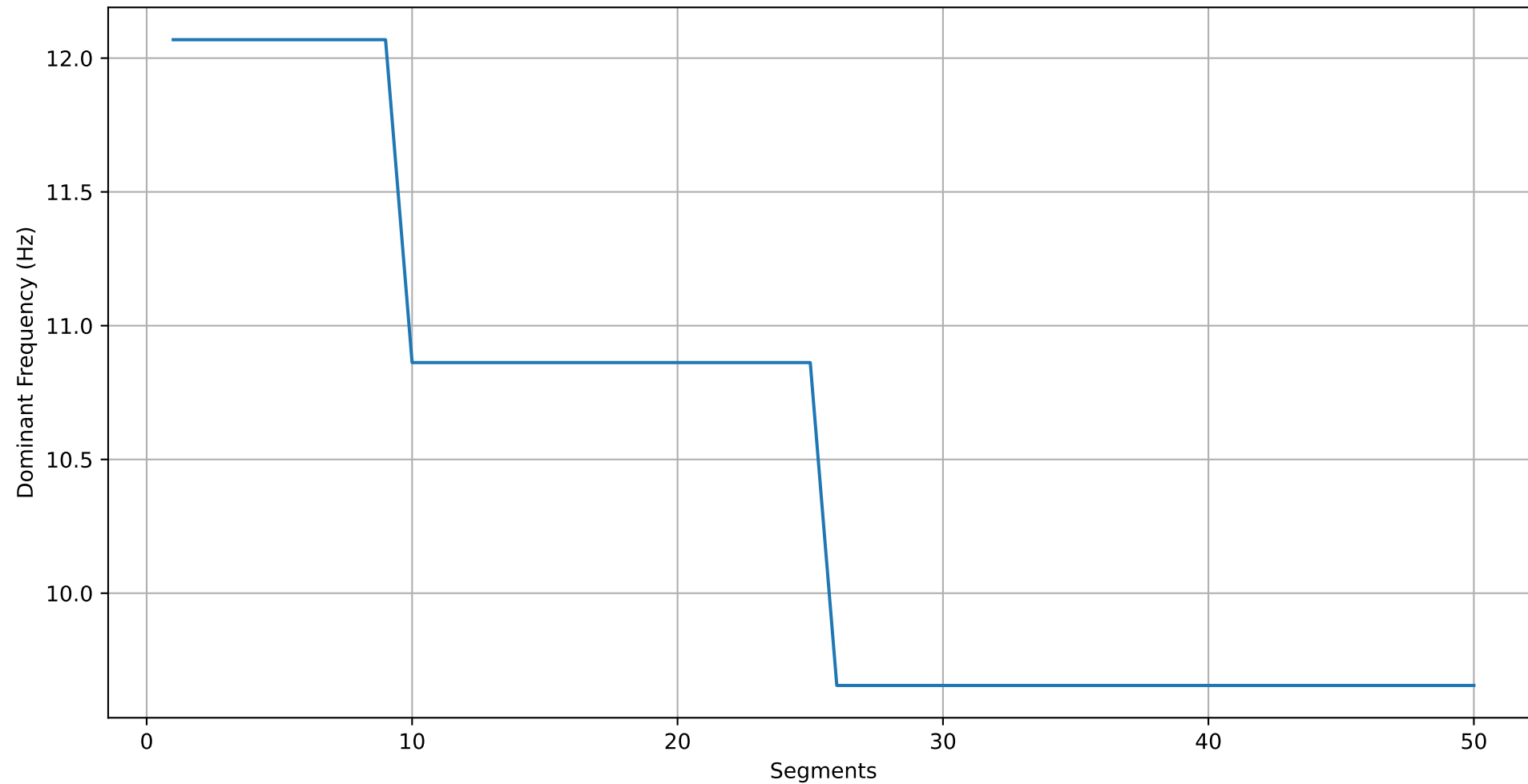
Dominant Frequencies in the Segments (10mm 45° 1.0)
