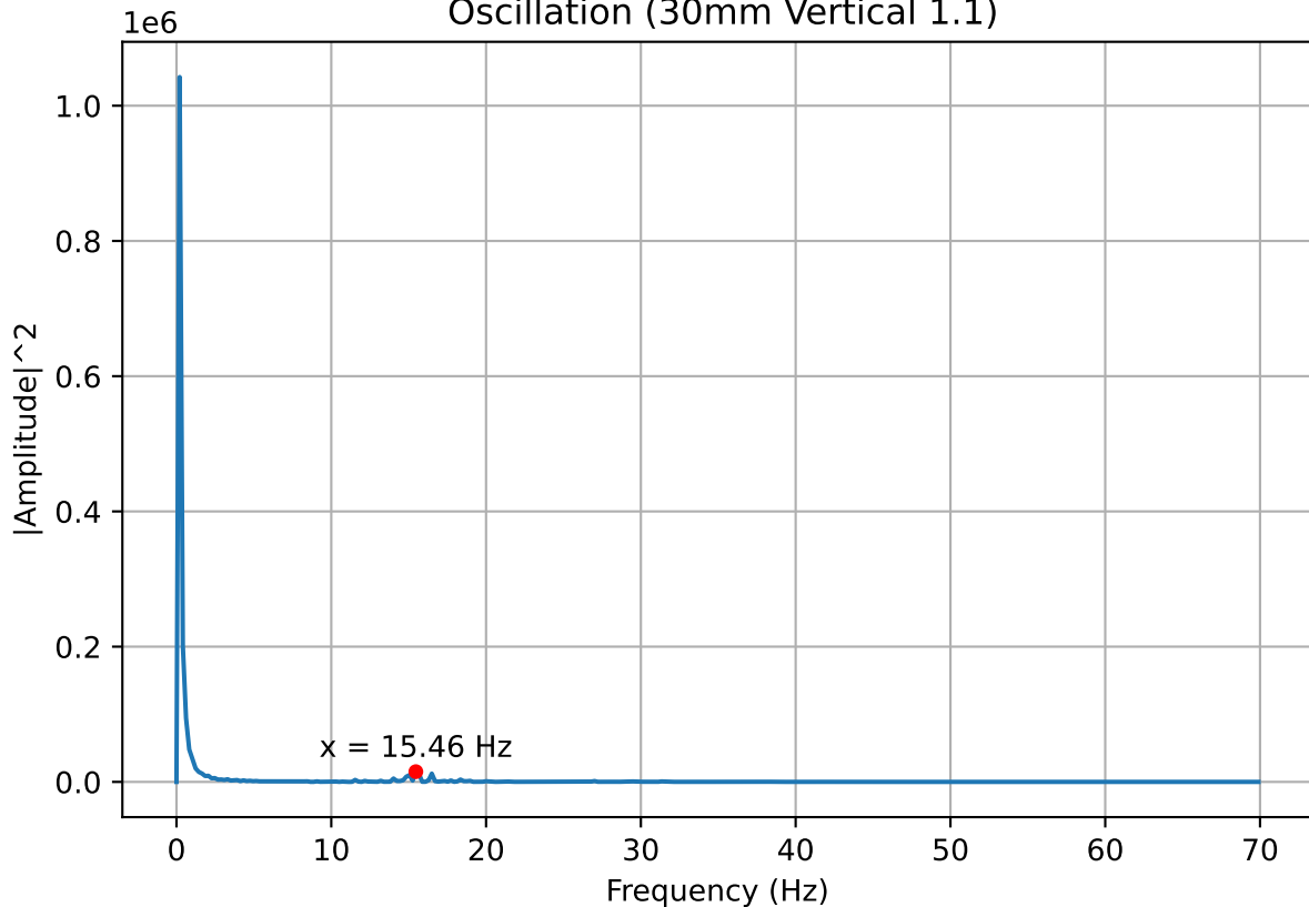
Frequency Power Spectrum of Pressure Oscillation (30mm Vertical 1.1)
