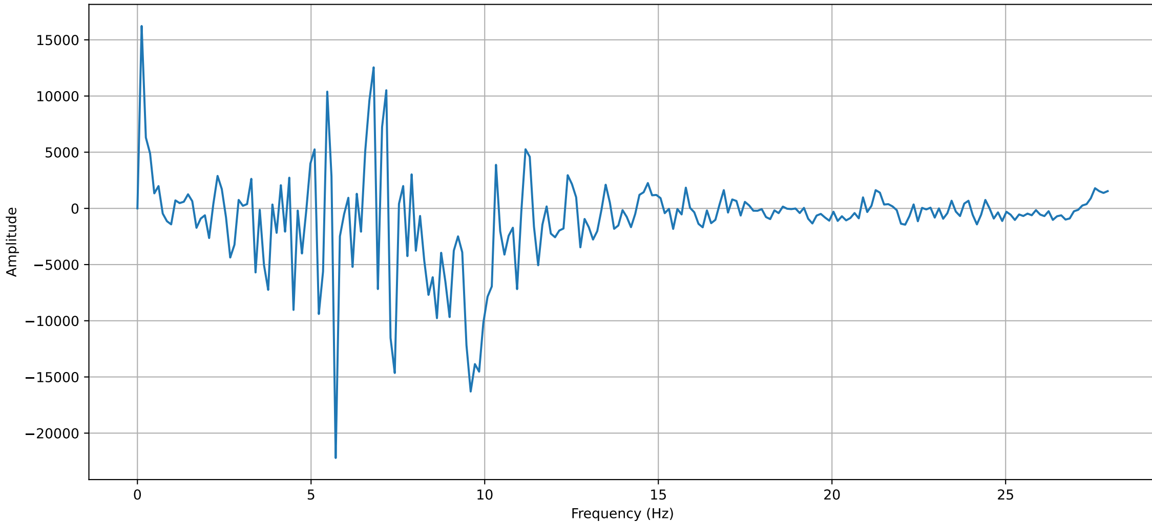
Frequency spectrum of the Pressure oscillation (30mm 45° 1.0)
