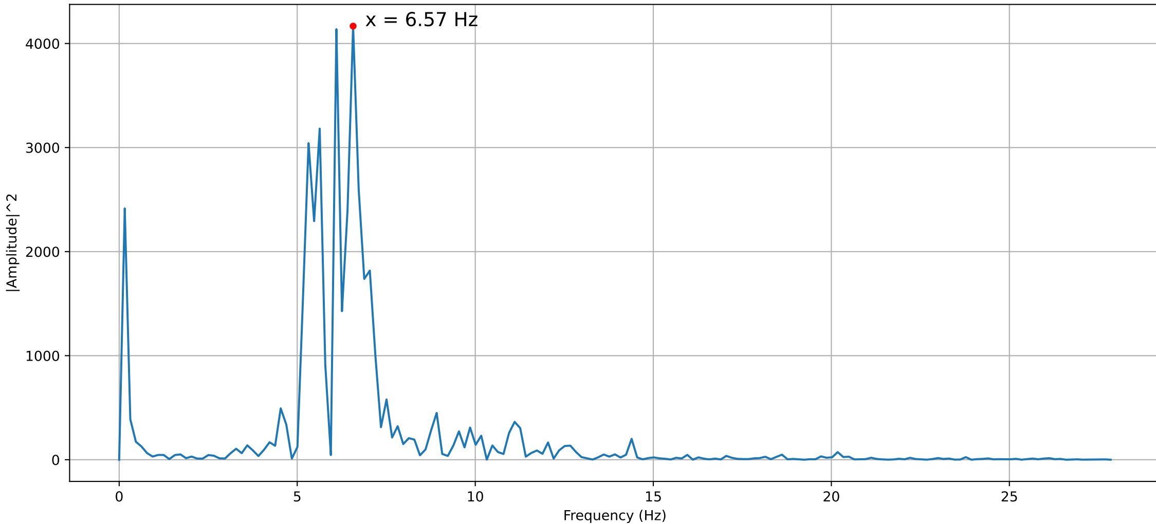
Frequency Power Spectrum of Pressure Oscillation (30mm 90° 4.0)
