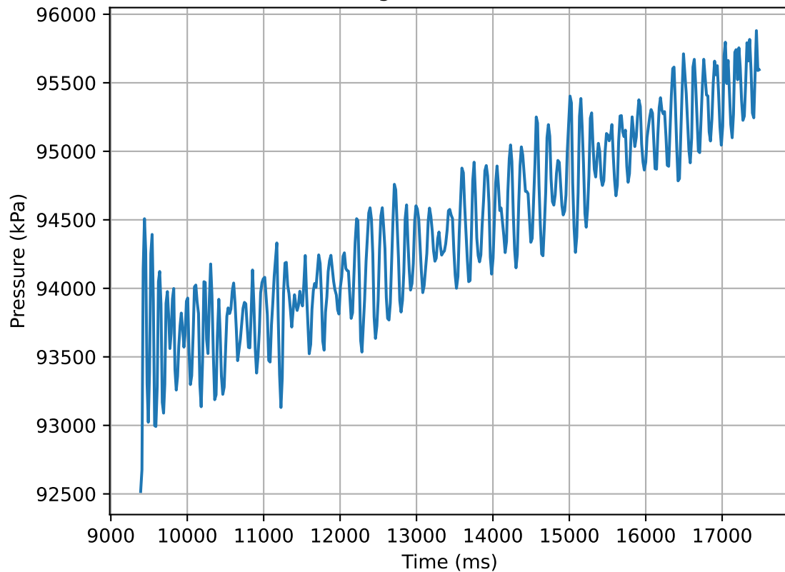
Pressure change in time (30mm 45° 1.0)
