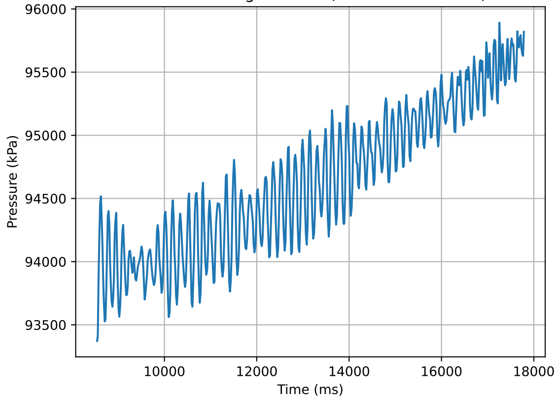
Pressure change in time (30mm Vertical 2.0)
