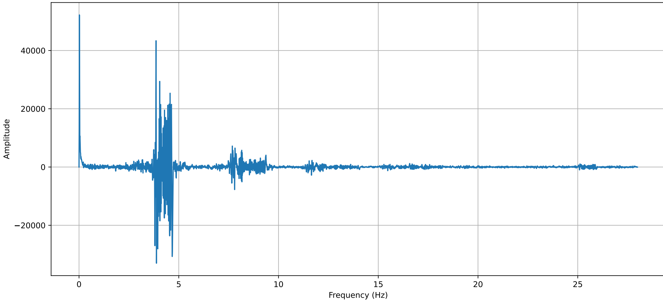
Frequency spectrum of the Pressure oscillation (10mm 45° 1.0)
