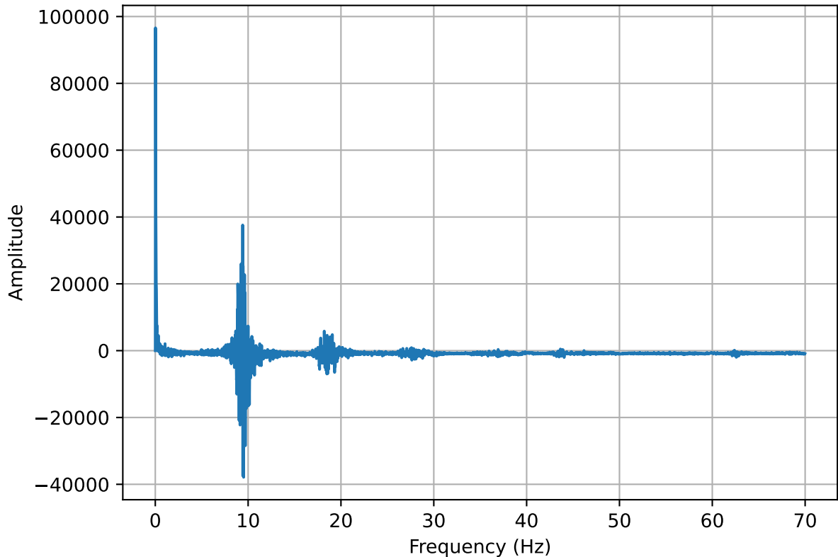
Frequency spectrum of the Pressure oscillation (10mm 90° 1.0)
