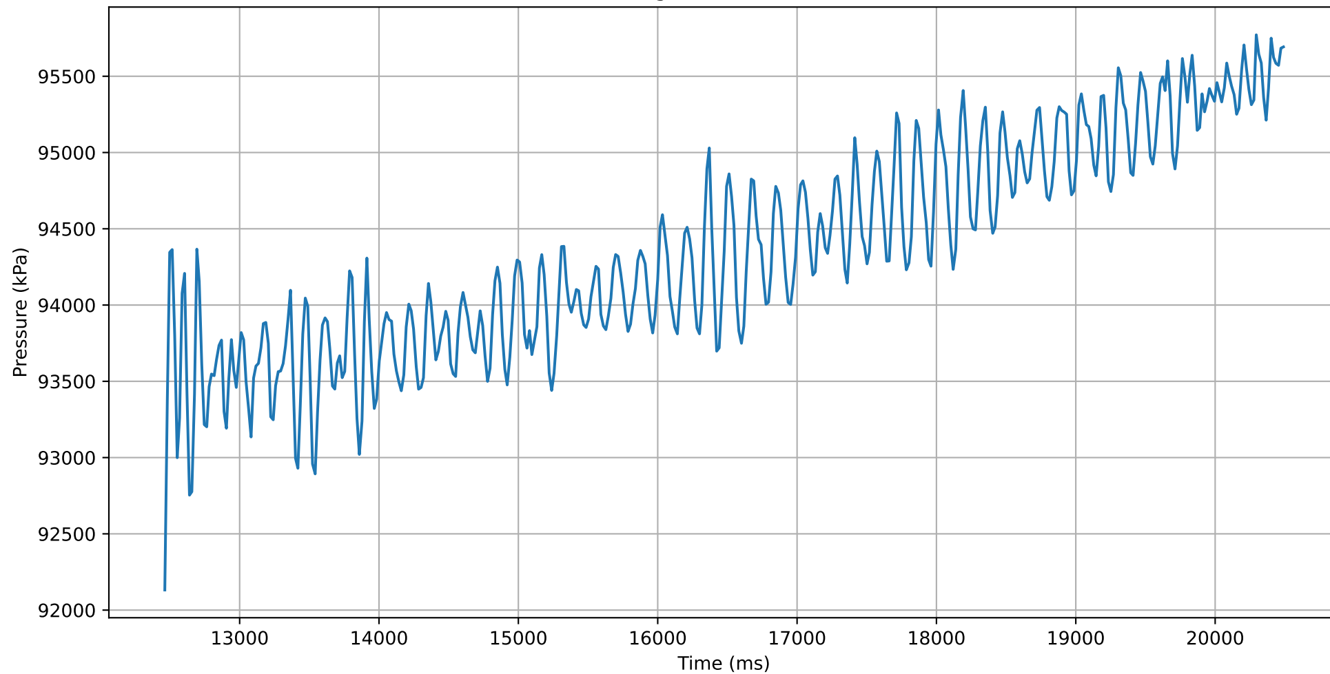
Pressure change in time (30mm 60° 1.0)
