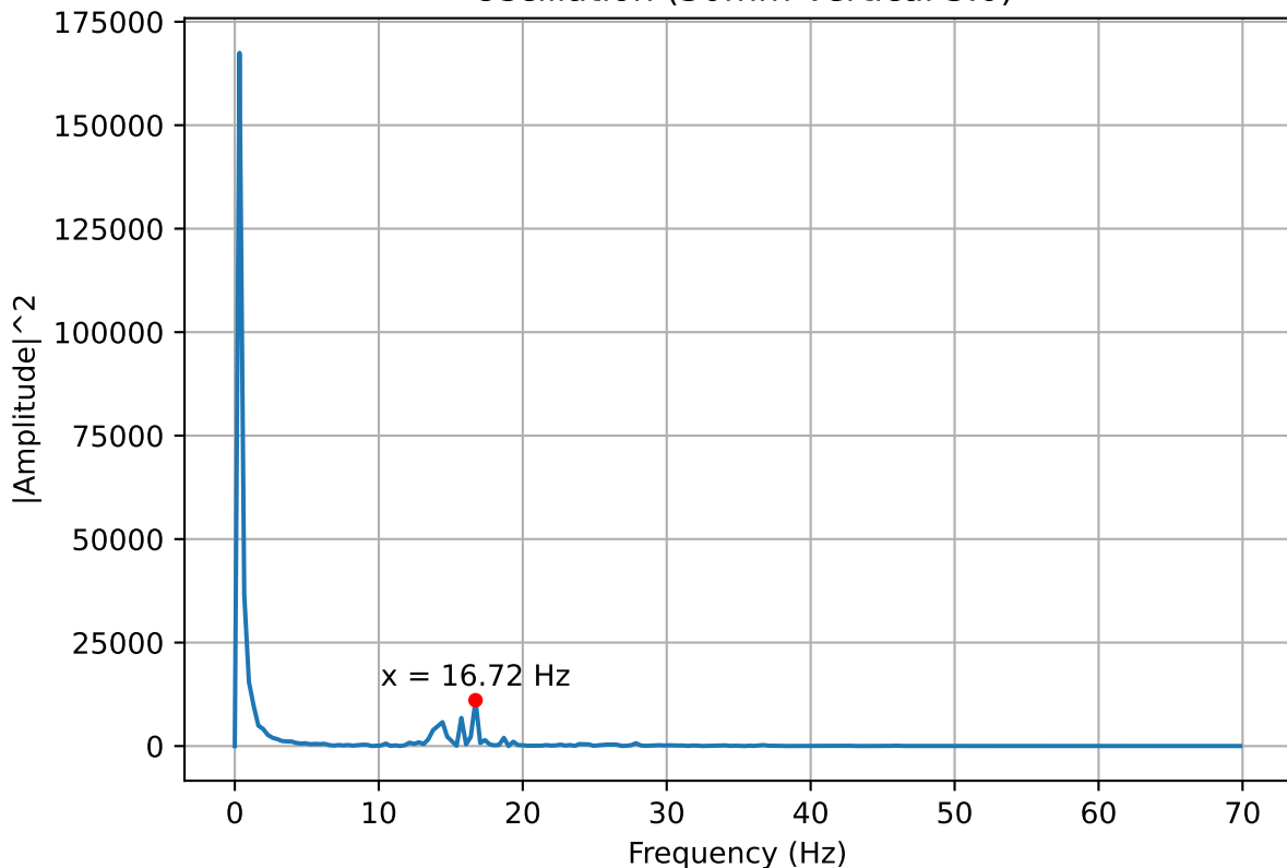
Frequency Power Spectrum of Pressure Oscillation (30mm Vertical 3.0)
