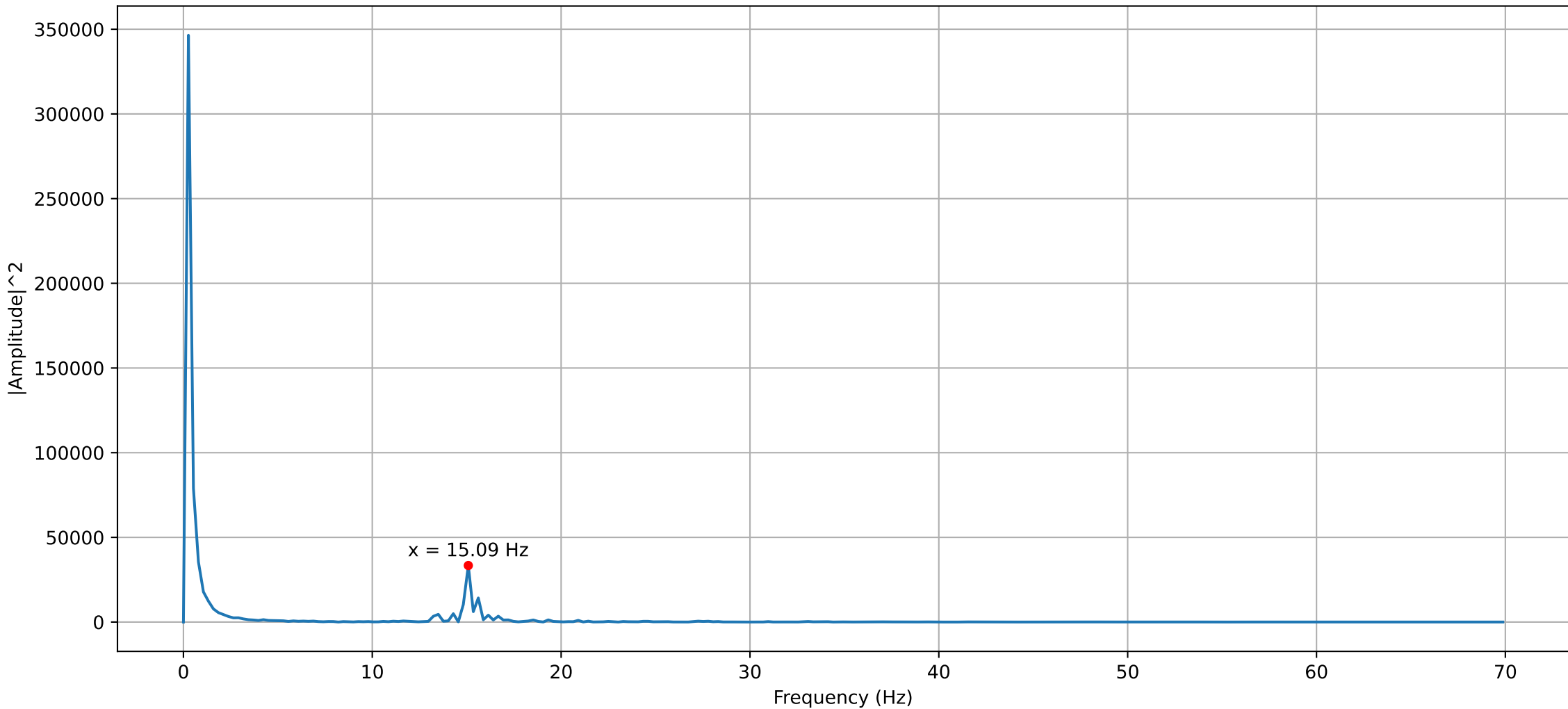
Frequency Power Spectrum of Pressure Oscillation (30mm 90° 2.0)
