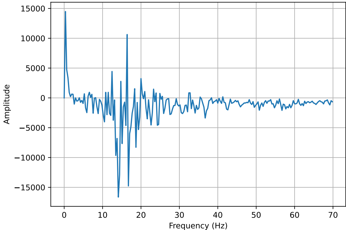
Frequency spectrum of the Pressure oscillation (30mm Vertical 3.0)
