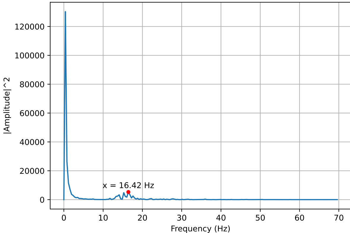
Frequency Power Spectrum of Pressure Oscillation (30mm 90° 4.0)
