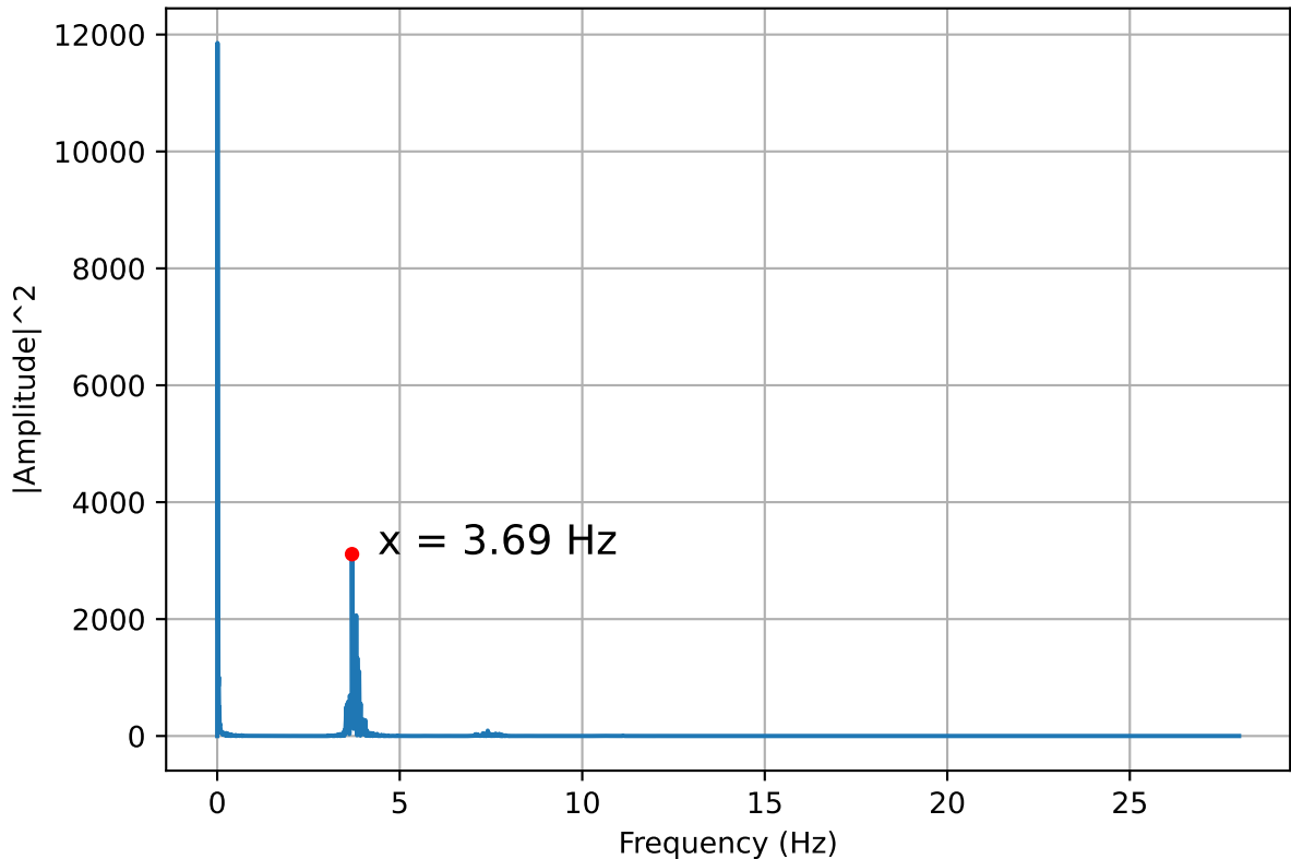
Frequency Power Spectrum of Pressure Oscillation (10mm 90° 1.0)
