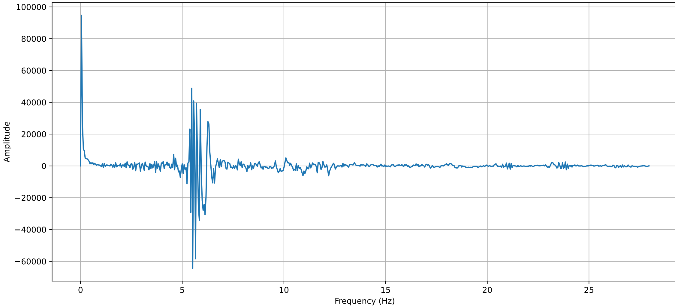
Frequency spectrum of the Pressure oscillation (20mm 60° 1.0)
