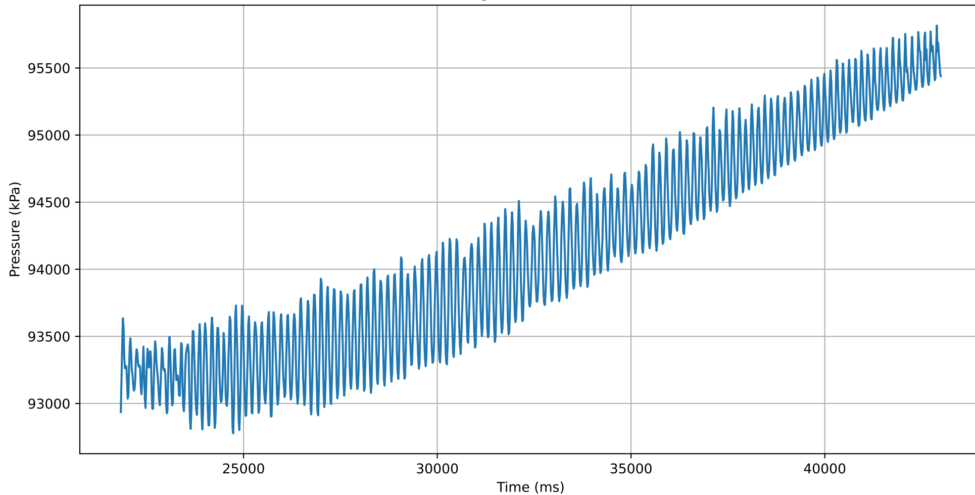
Pressure change in time (20mm 60° 1.0)
