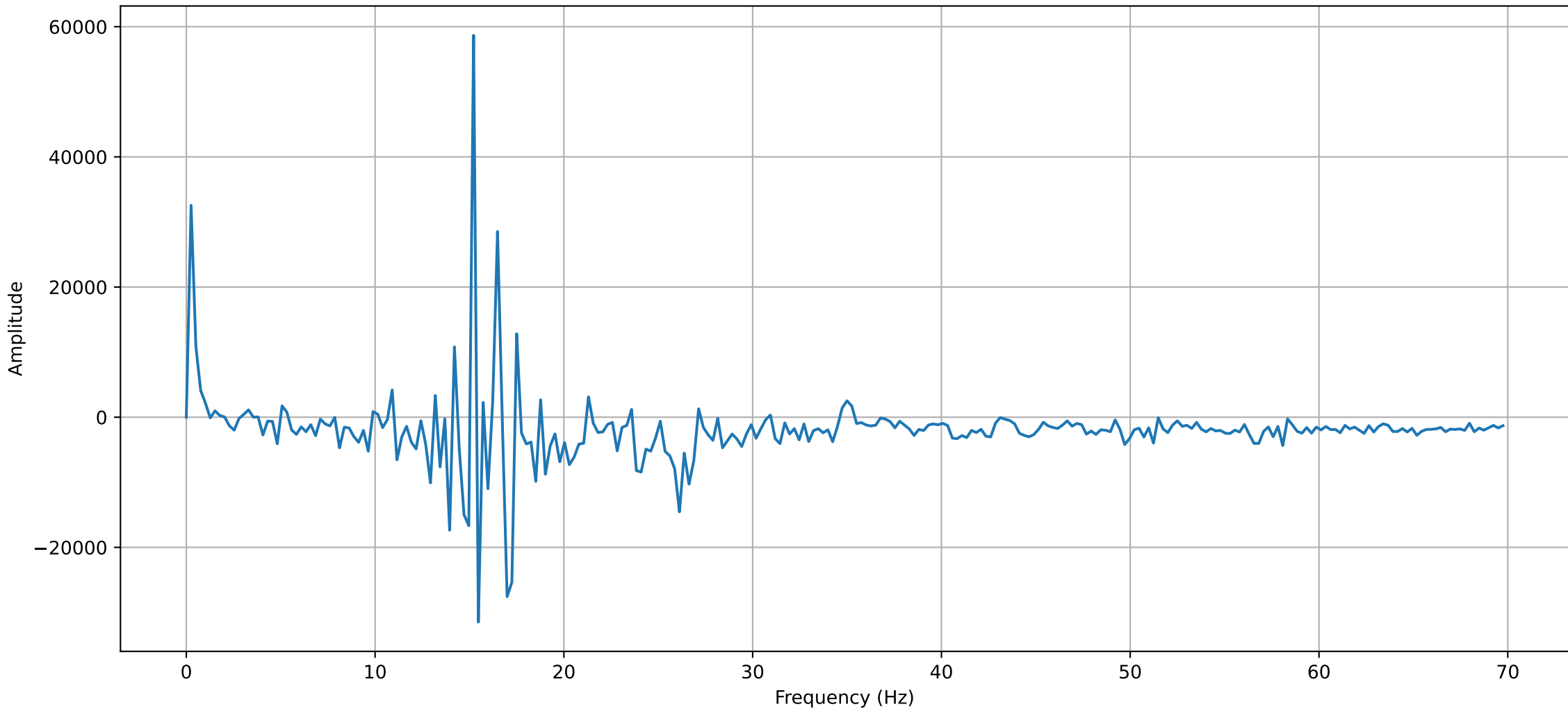
Frequency spectrum of the Pressure oscillation (30mm 70° 1.0)
