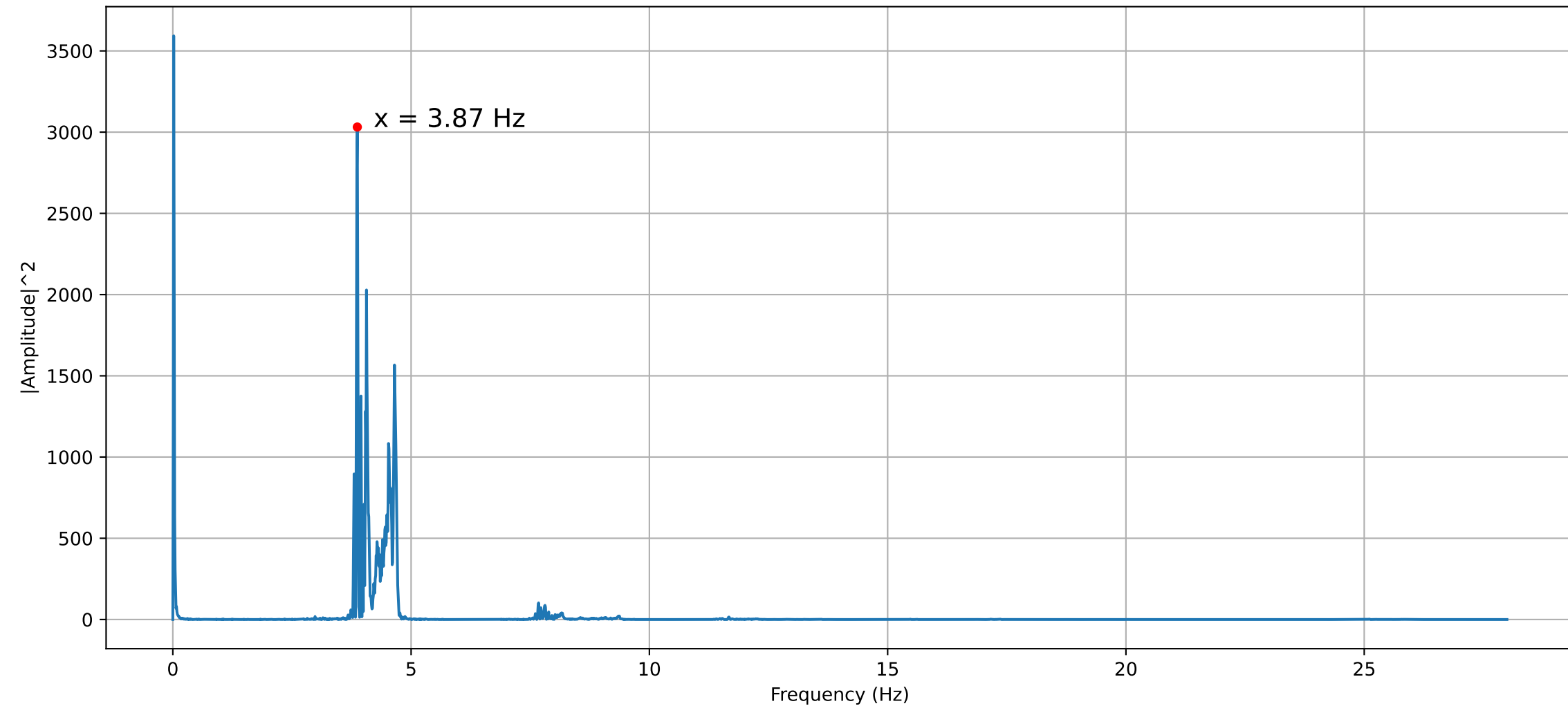
Frequency Power Spectrum of Pressure Oscillation (10mm 45° 1.0)
