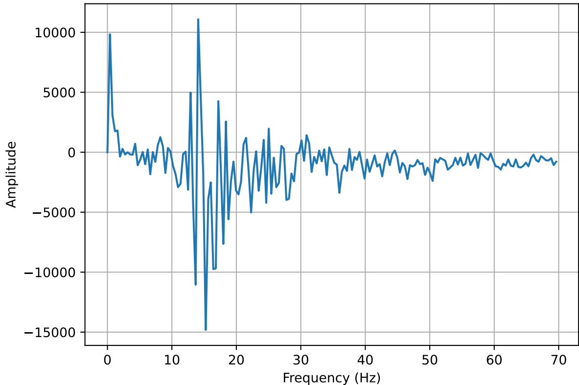
Frequency spectrum of the Pressure oscillation (30mm Vertical 4.0)
