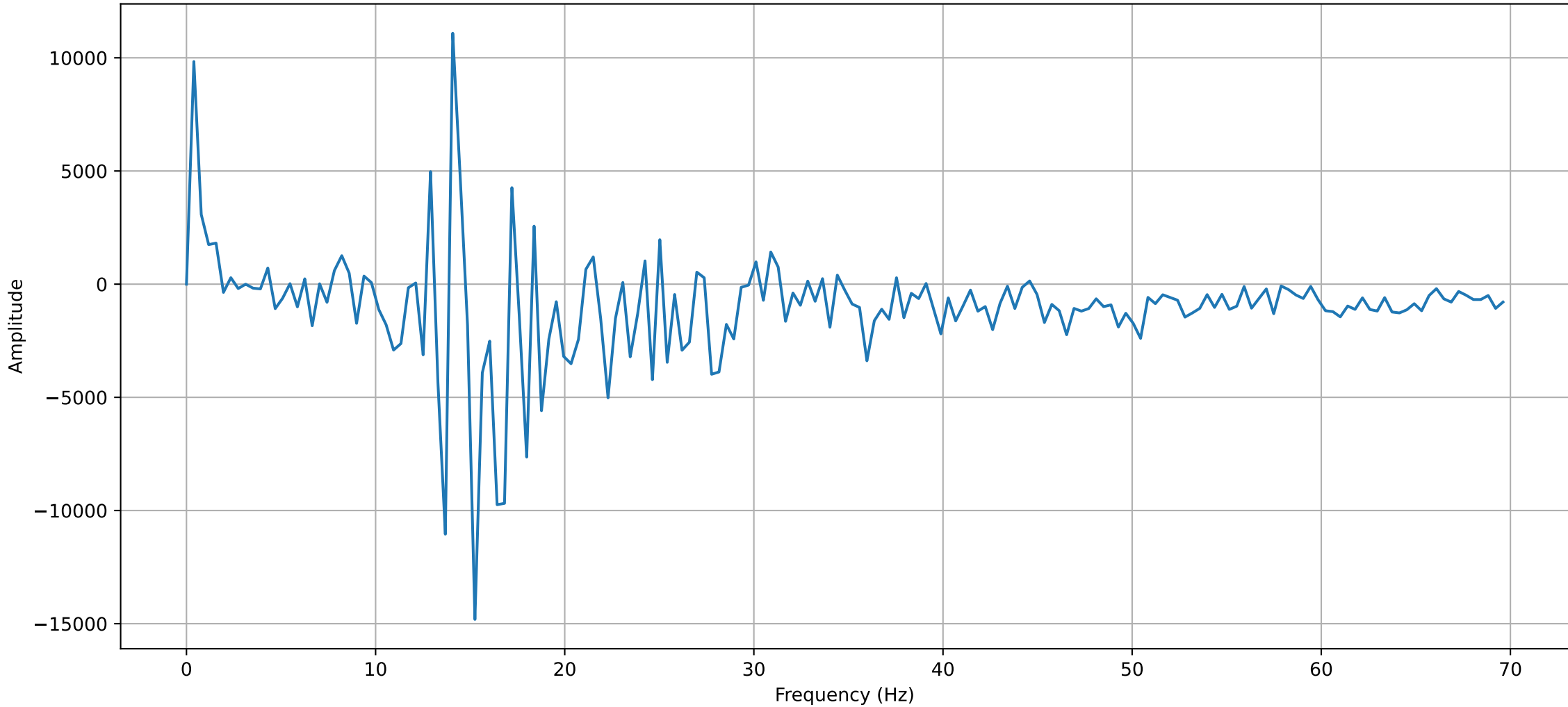
Frequency spectrum of the Pressure oscillation (30mm 90° 4.0)
