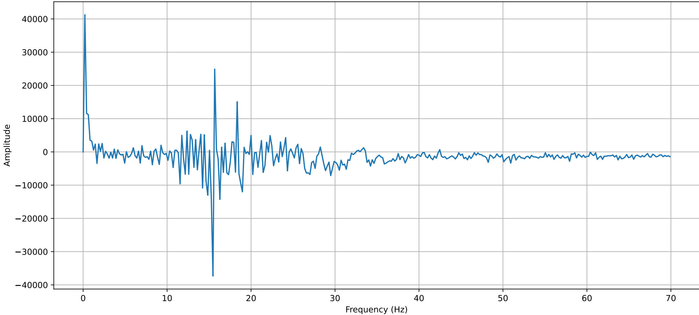
Frequency spectrum of the Pressure oscillation (30mm 90° 1.1)
