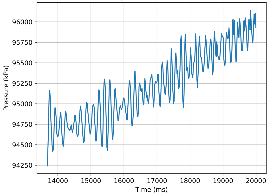
Pressure change in time (30mm Vertical 4.0)
