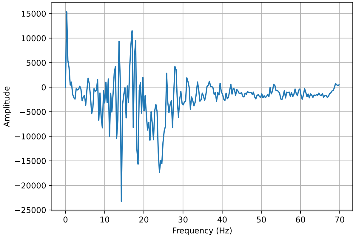
Frequency spectrum of the Pressure oscillation (30mm 45° 1.0)
