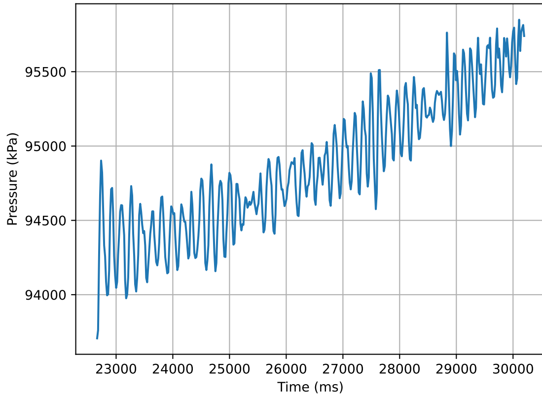
Pressure change in time (30mm Vertical 3.0)
