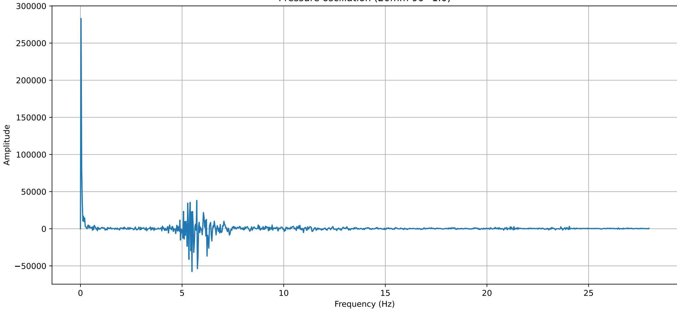
Frequency spectrum of the Pressure oscillation (20mm 90° 1.0)
