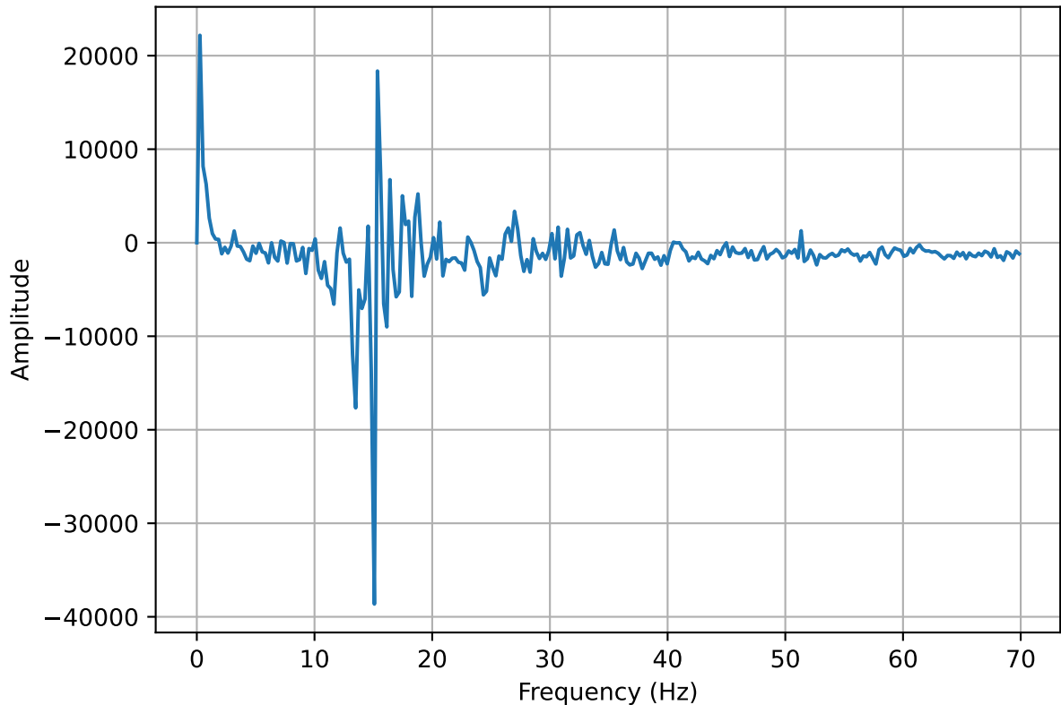
Frequency spectrum of the Pressure oscillation (30mm Vertical 2.0)
