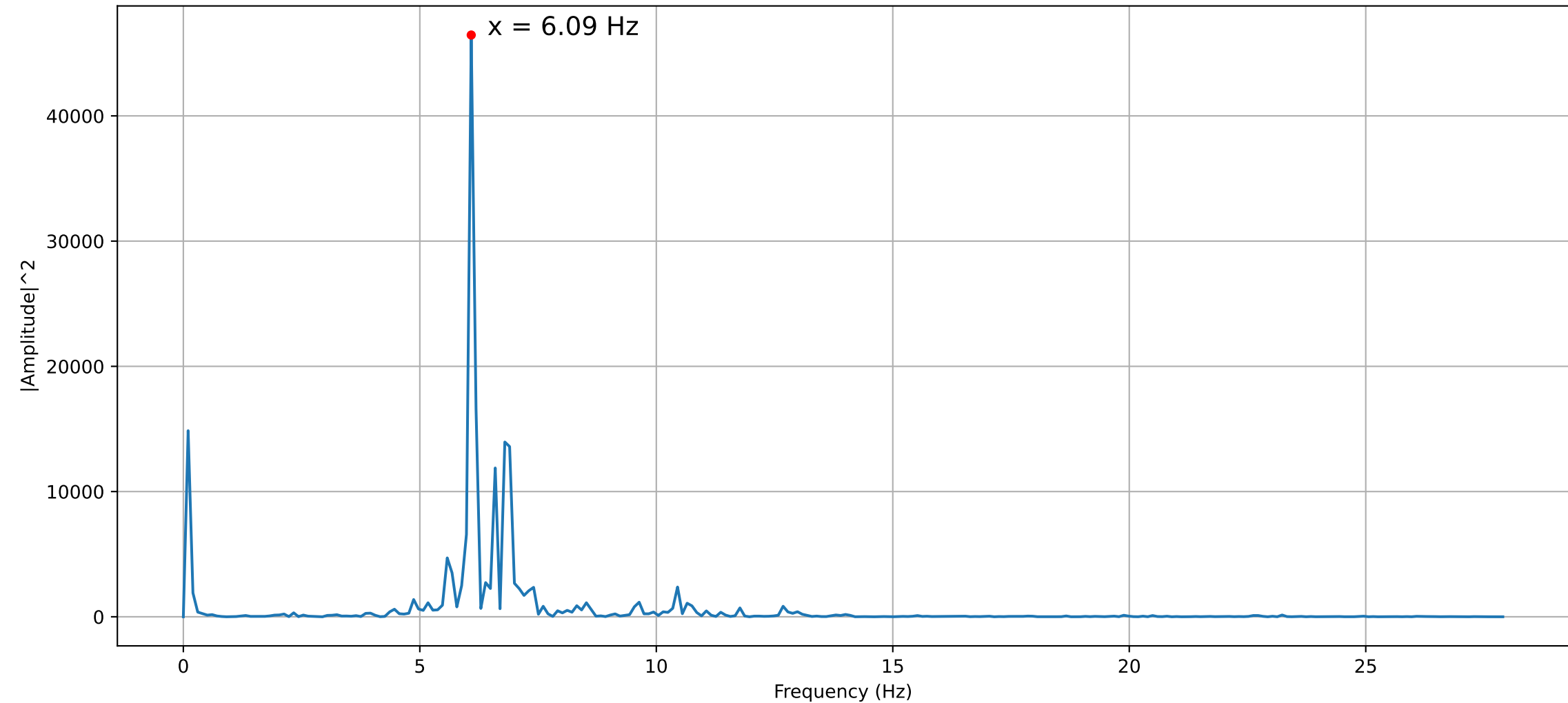
Frequency Power Spectrum of Pressure Oscillation (30mm 70° 1.0)
