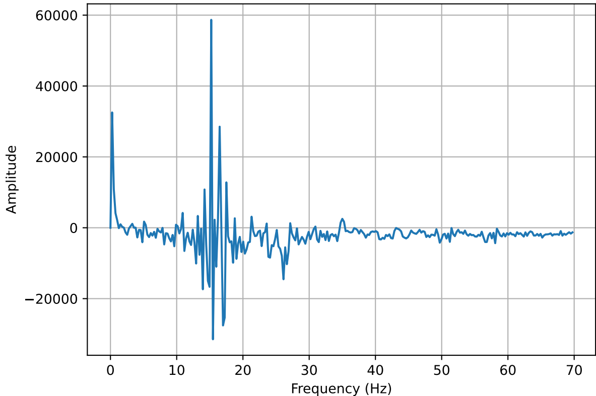
Frequency spectrum of the Pressure oscillation (30mm 70° 1.0)
