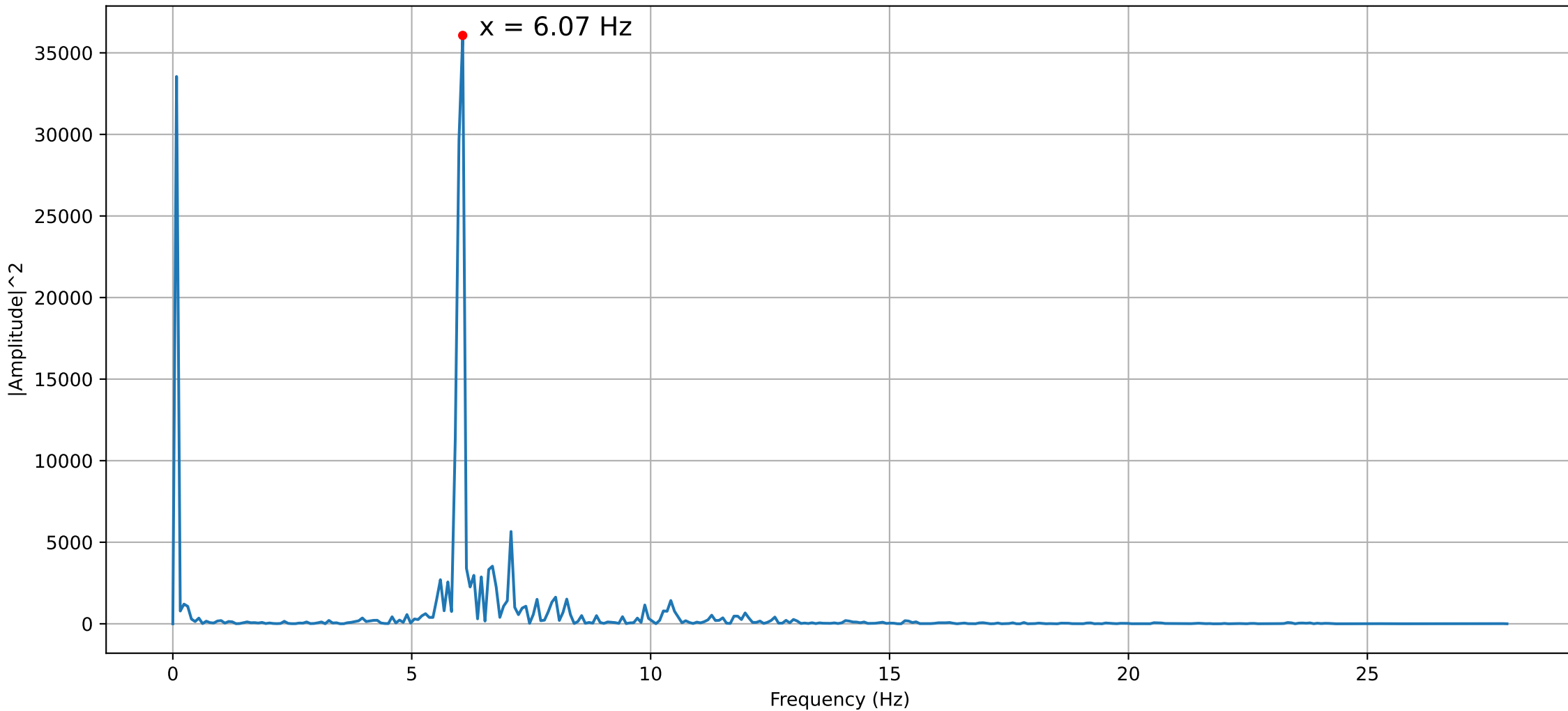
Frequency Power Spectrum of Pressure Oscillation (30mm 90° 1.0)
