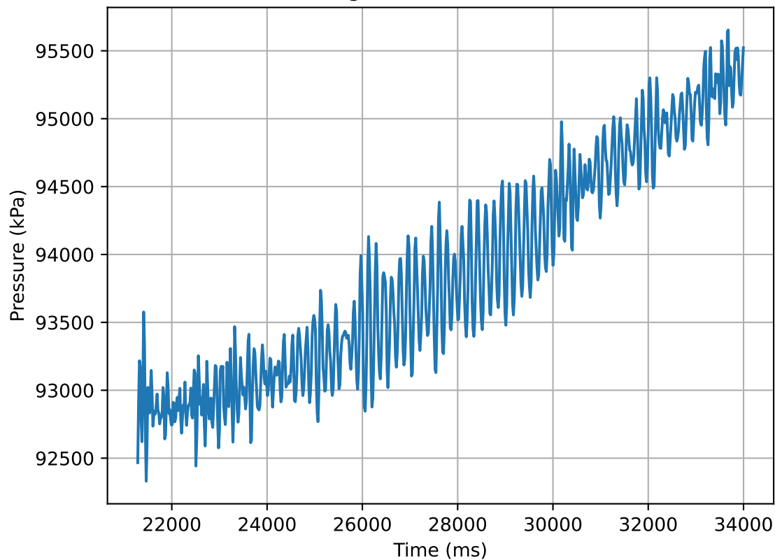
Pressure change in time (30mm Vertical 1.0)
