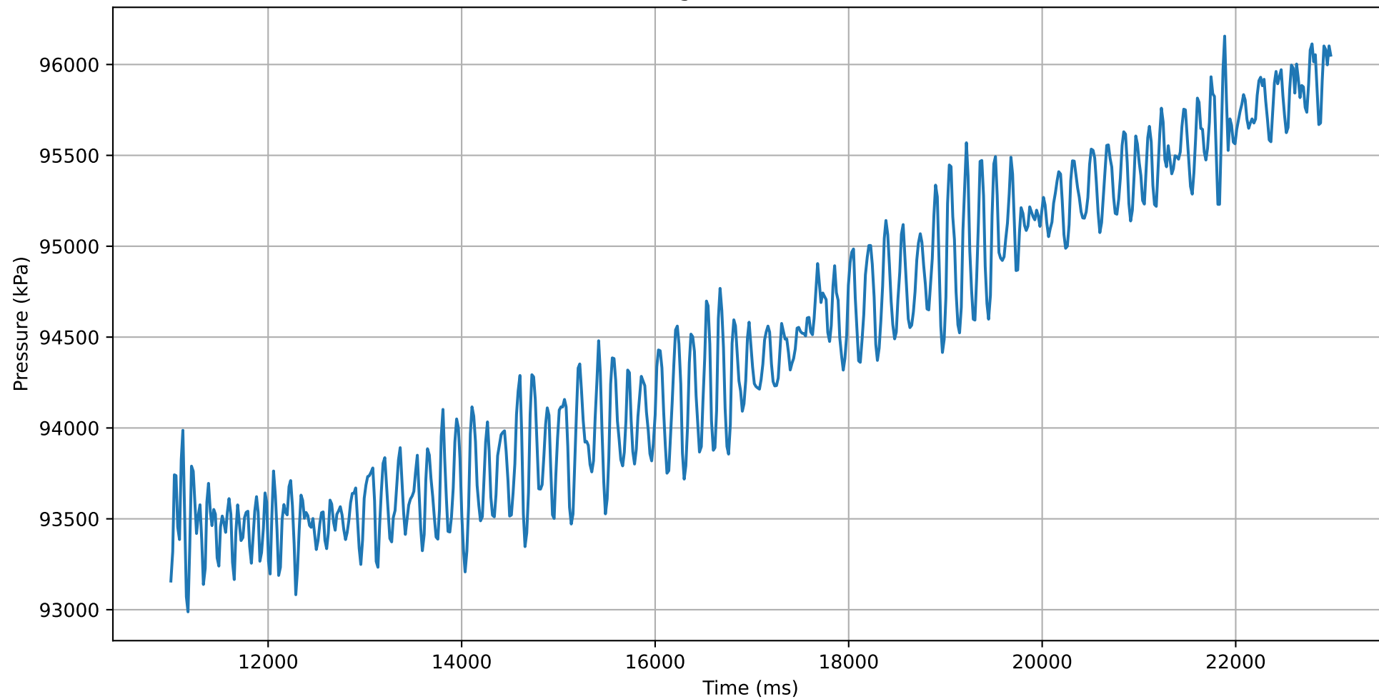
Pressure change in time (30mm 90° 1.1)
