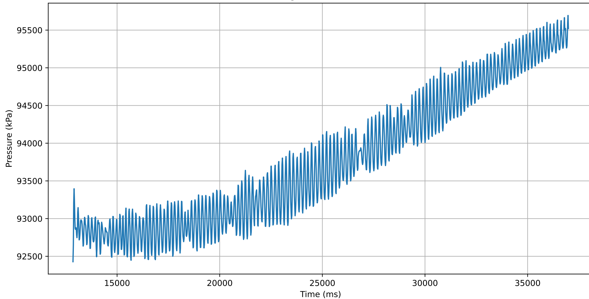
Pressure change in time (20mm 70° 1.0)
