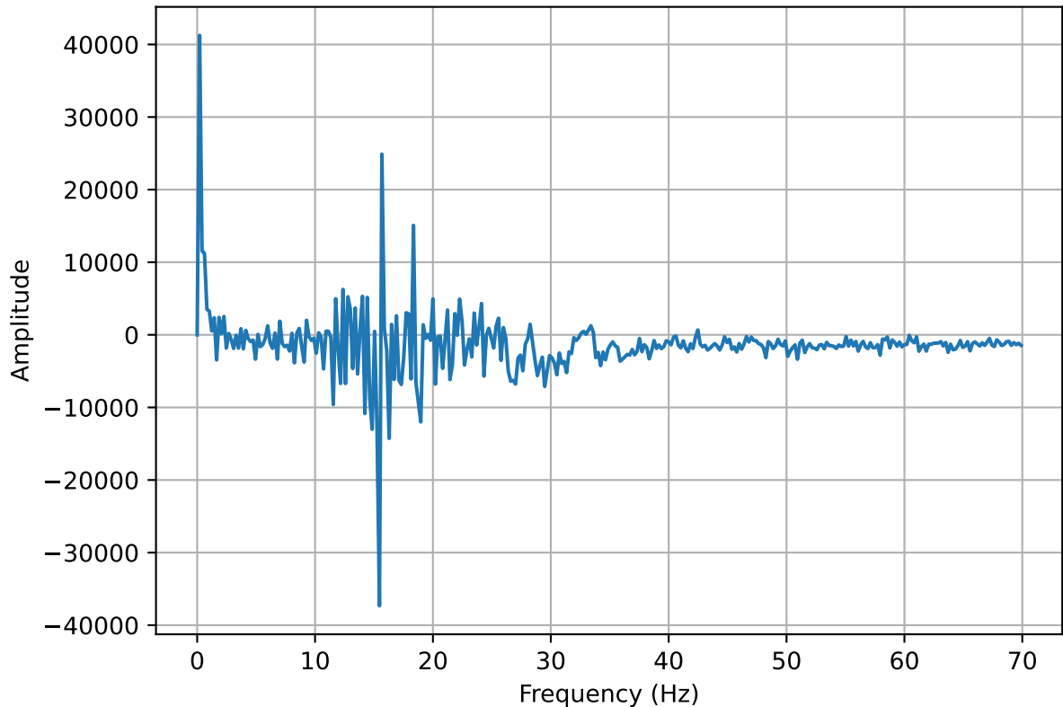
Frequency spectrum of the Pressure oscillation (30mm Vertical 1.1)
