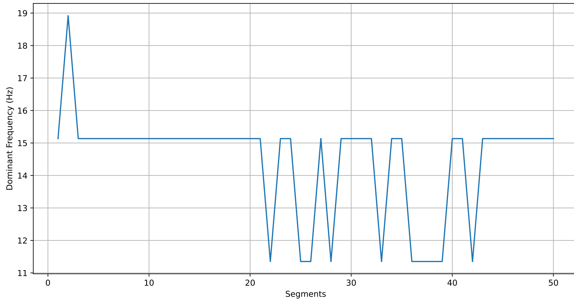
Dominant Frequencies in the Segments (20mm 90° 1.0)
