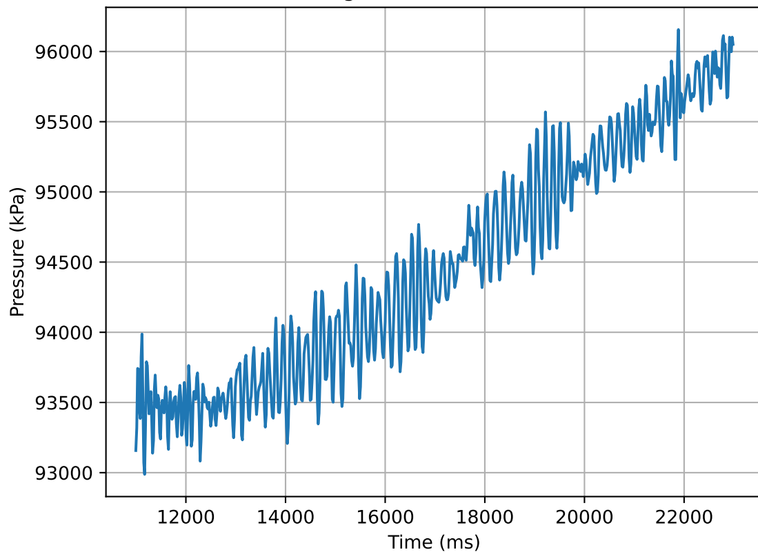
Pressure change in time (30mm Vertical 1.1)
