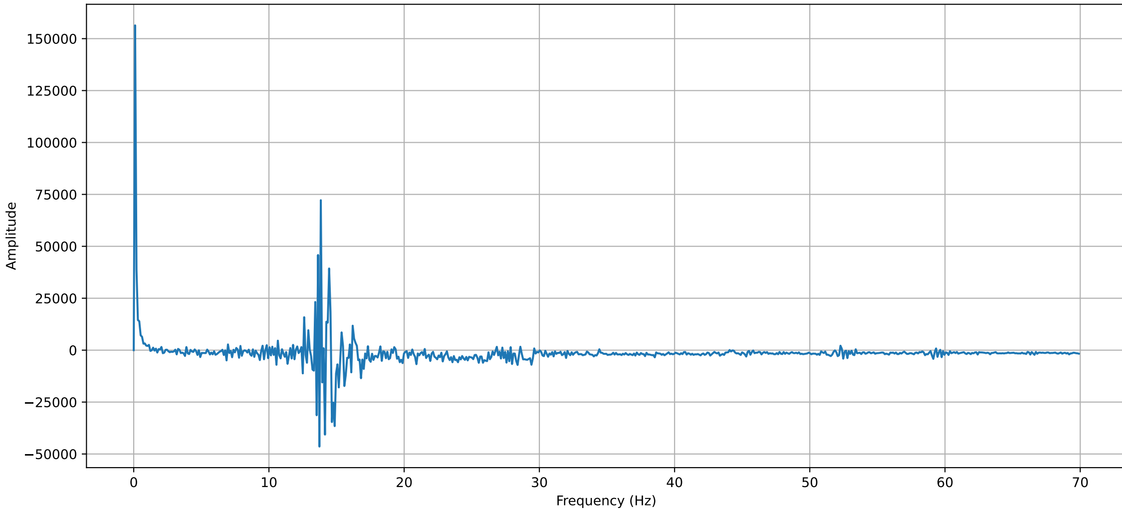
Frequency spectrum of the Pressure oscillation (20mm 70° 1.0)
