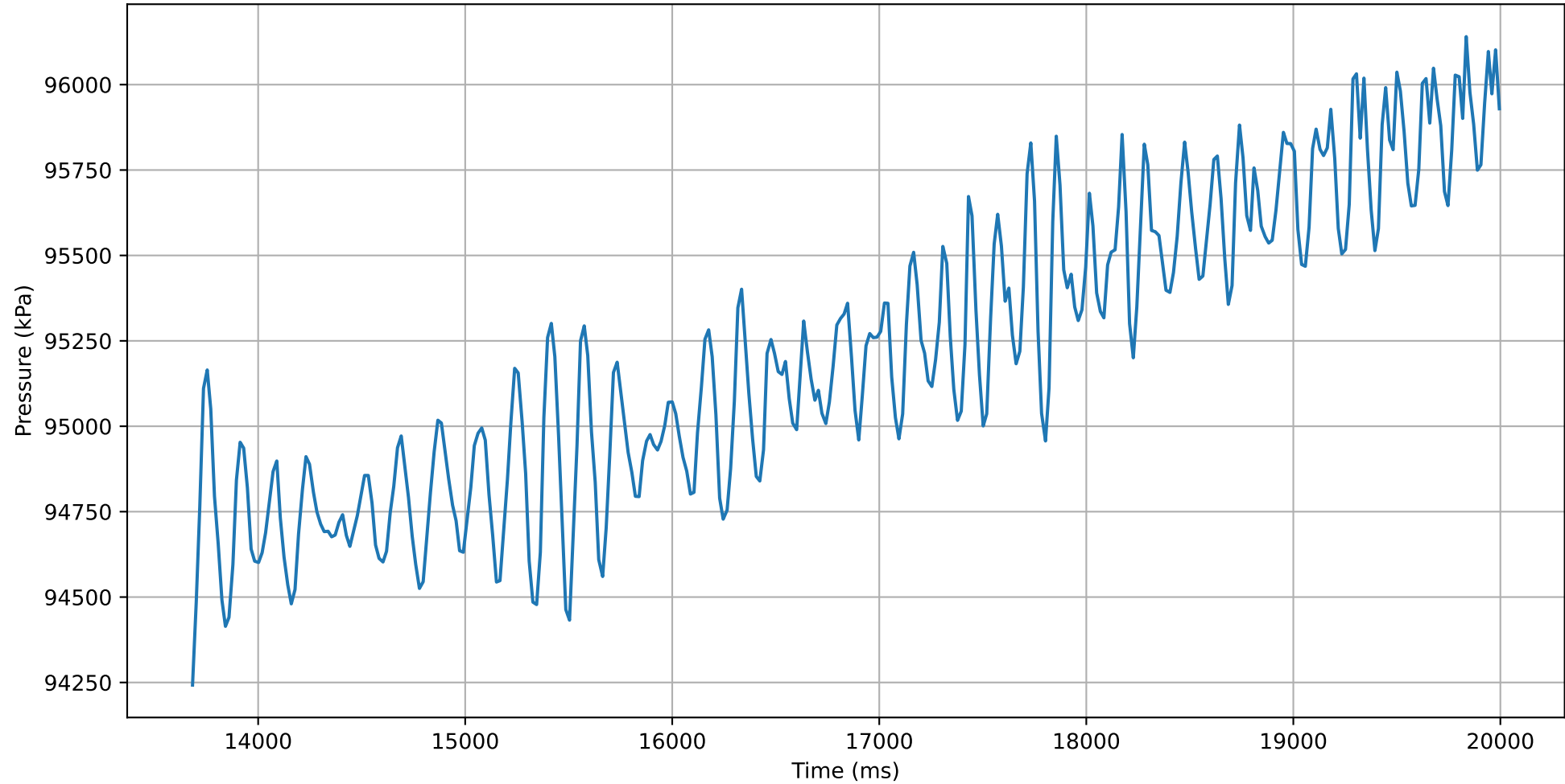
Pressure change in time (30mm 90° 4.0)
