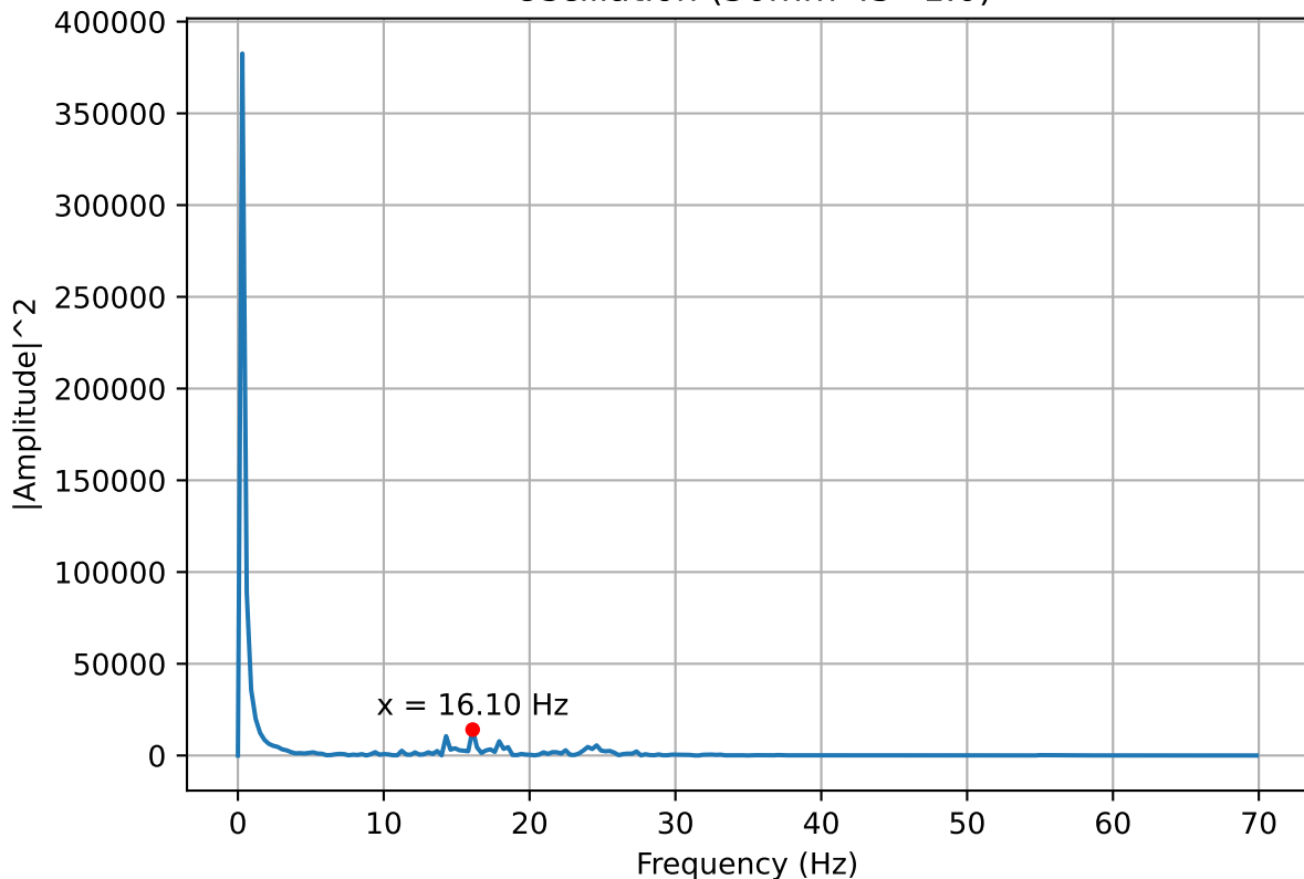
Frequency Power Spectrum of Pressure Oscillation (30mm 45° 1.0)
