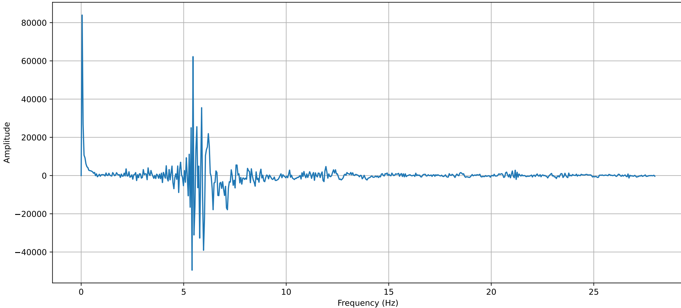
Frequency spectrum of the Pressure oscillation (20mm 45° 1.0)
