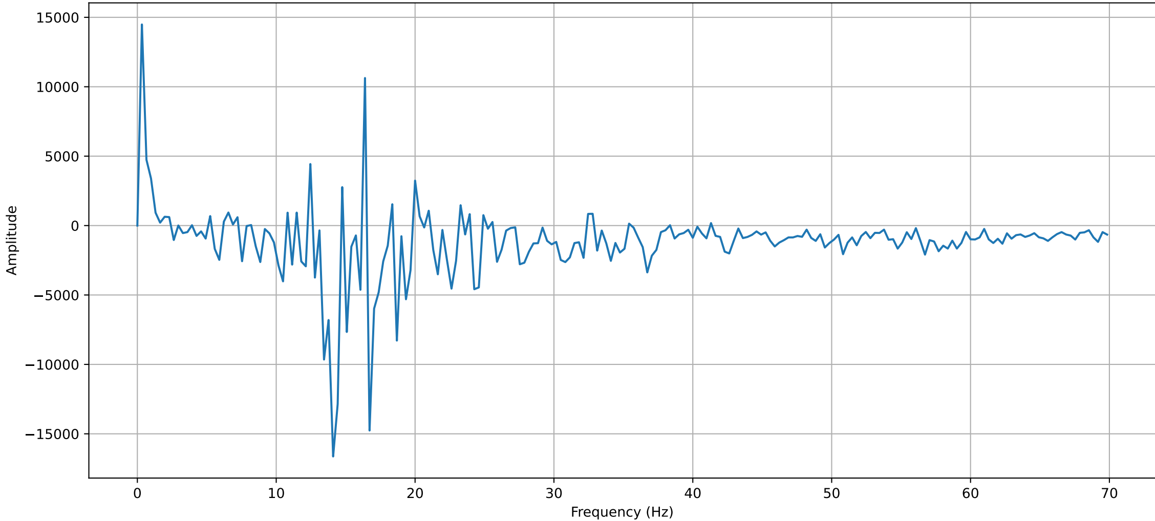
Frequency spectrum of the Pressure oscillation (30mm 90° 3.0)
