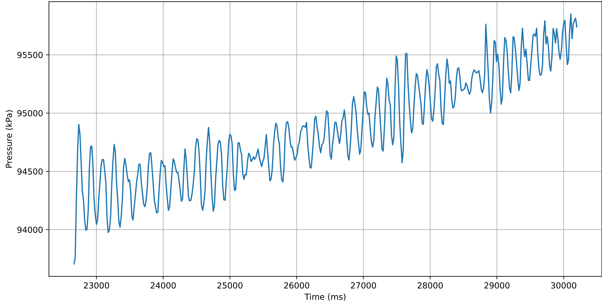
Pressure change in time (30mm 90° 3.0)
