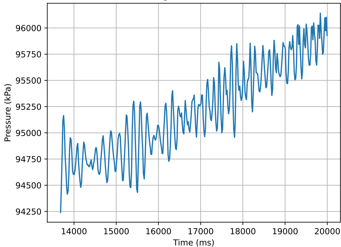
Pressure change in time (30mm 90° 4.0)
