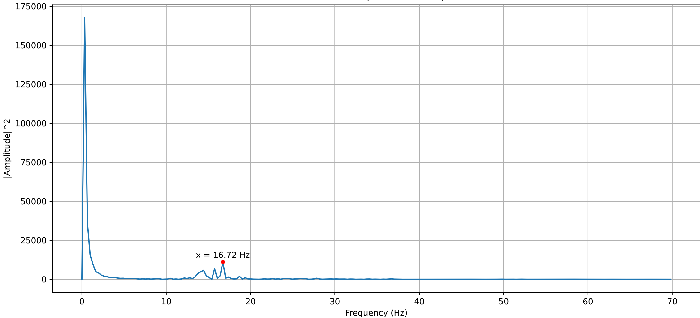
Frequency Power Spectrum of Pressure Oscillation (30mm 90° 3.0)
