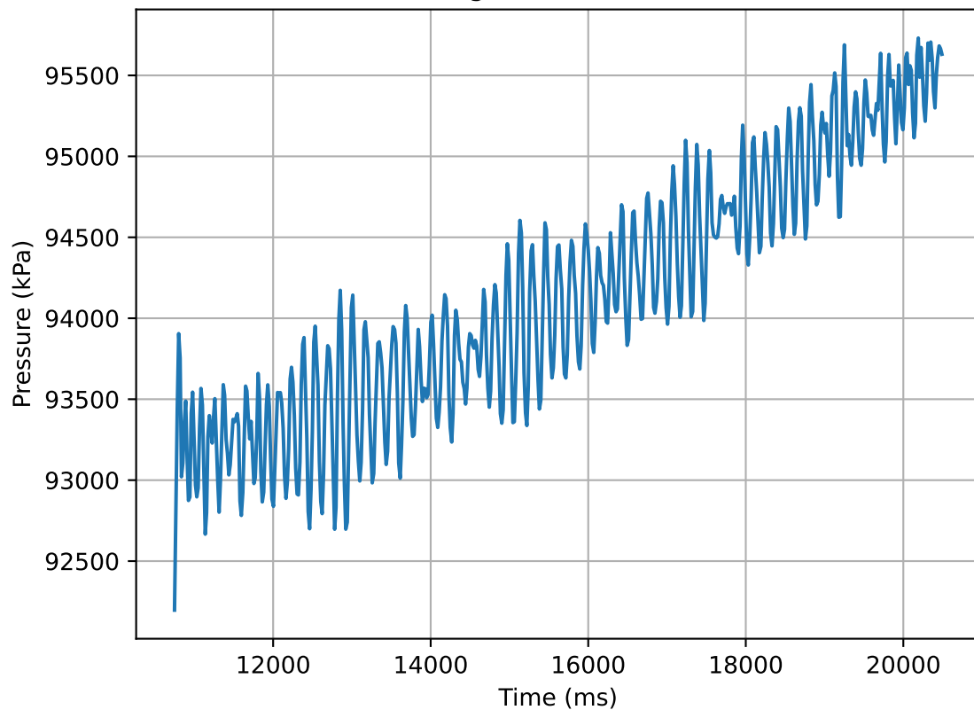
Pressure change in time (30mm 70° 1.0)
