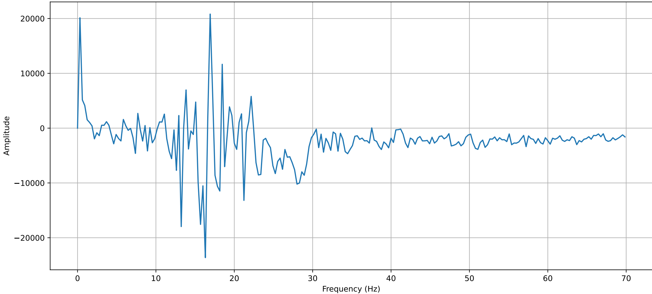
Frequency spectrum of the Pressure oscillation (30mm 60° 1.0)
