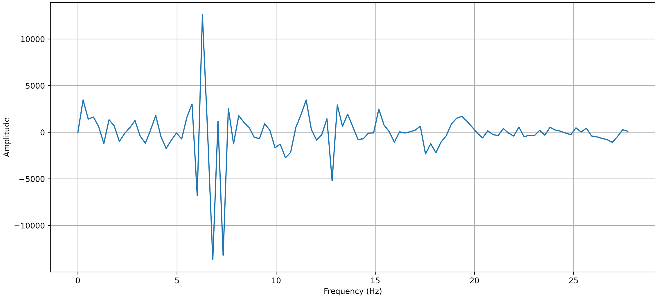
Frequency spectrum of the Pressure oscillation (40mm 90° 1.0)
