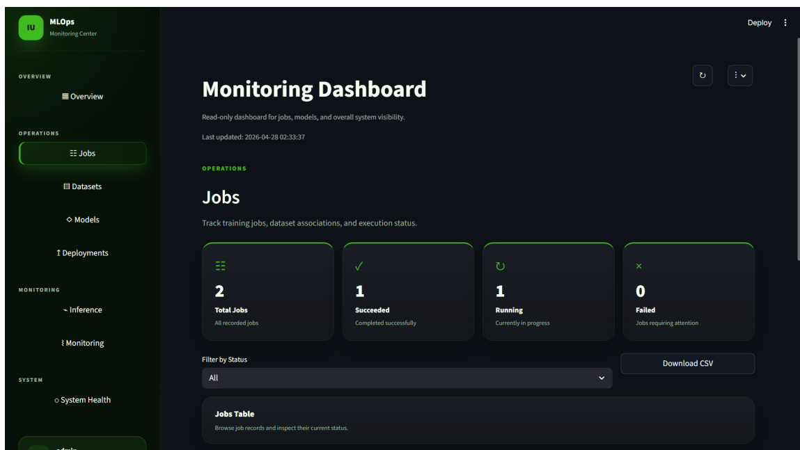
Figure 7: Monitoring Dashboard – Jobs page. Displays all training jobs with their current lifecycle status (total, running, succeeded, failed) and associated dataset metadata.
