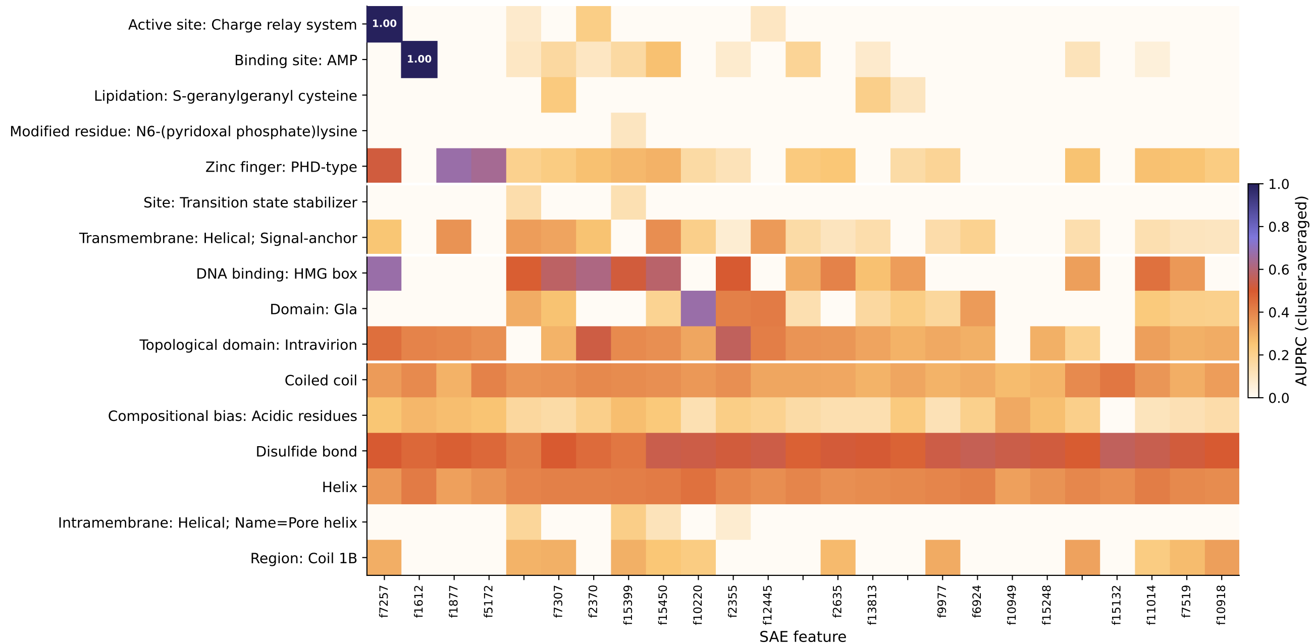
SAE feature × UniProt annotation alignment
