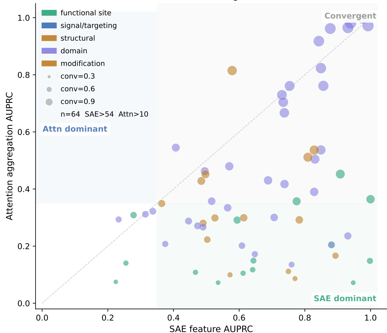
SAE × Attention convergence (64 annotation subtypes) (bubble size = convergence score)
