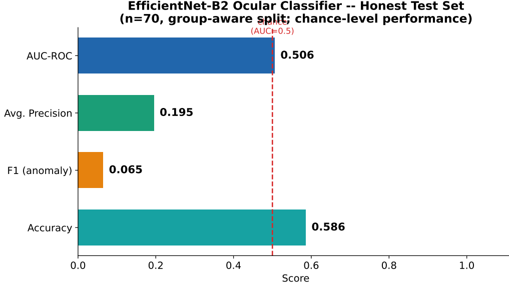
Figure S1: EfficientNet-B2 ocular anomaly classifier: leakage-free test-set metrics ( n = 70 , group-aware split). AUC-ROC = 0.506 sits on the chance line (dashed), with Average Precision = 0.195, F1 (anomaly) = 0.065 and Accuracy = 0.586.
