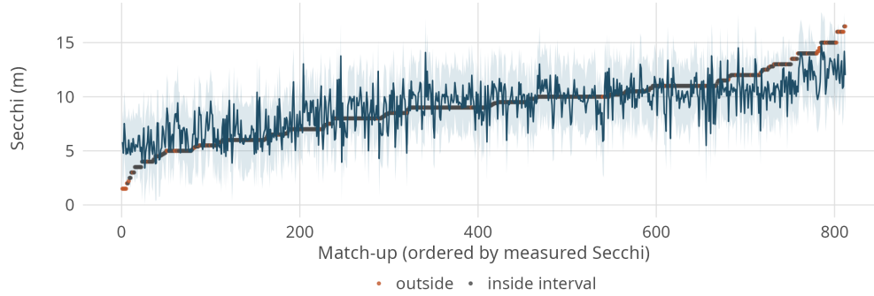
Figure A.7: Conformal prediction intervals under campaign-blocked validation. (a) Empirical versus nominal coverage: marginally calibrated across the 50–95% range. (b) The 90% interval against the measured value. (c) Coverage conditional on measured transparency. Because split conformal uses a single global residual quantile, the interval width is constant ( \approx 6.12 m) and cannot adapt, so the marginal guarantee is bought by over-covering in the middle of the range and under-covering at both extremes.
