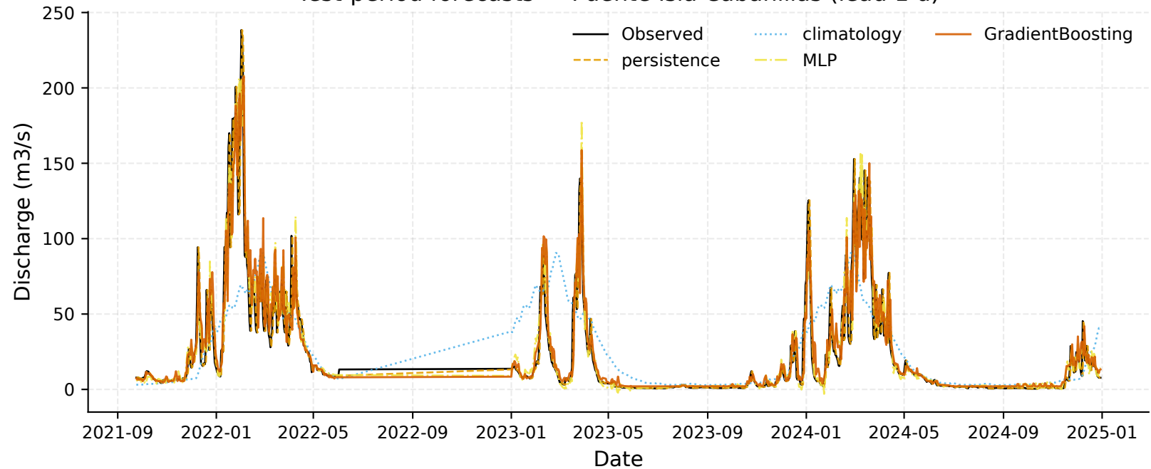
Test-period forecasts — Puente Isla Cabanillas (lead 1 d)
