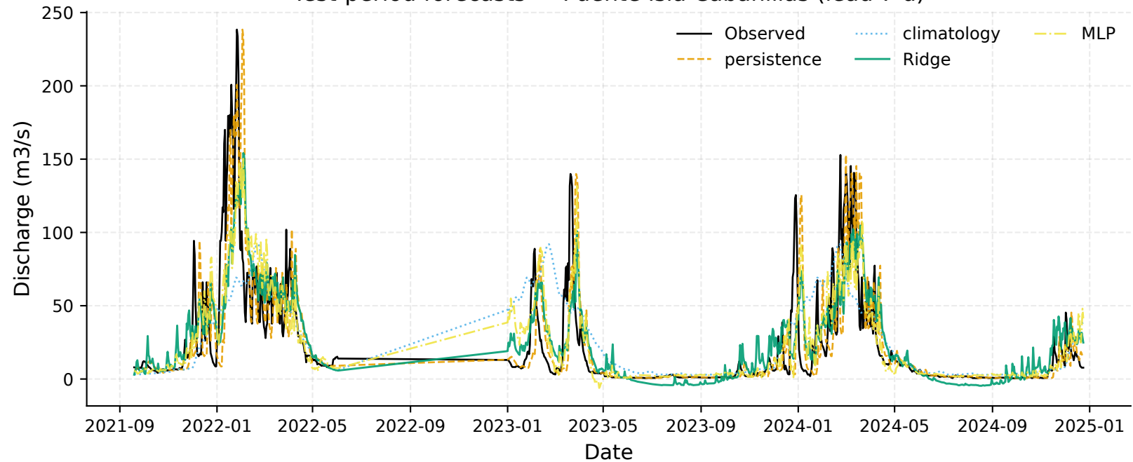
Test-period forecasts — Puente Isla Cabanillas (lead 7 d)
