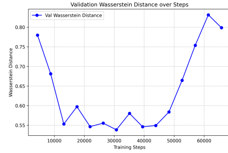
Fig. 3: Validation Wasserstein distance during training. The initial decrease shows the model learning the distribution, while the subsequent increase suggests a potential imbalance between the Generator and the Critic.
