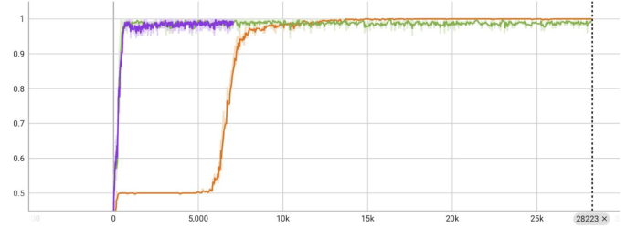
Fig. 2: Discriminator accuracy during the baseline training with BCE loss. The rapid convergence to 1 indicates that the Generator was immediately outperformed, leading to vanishing gradients.
