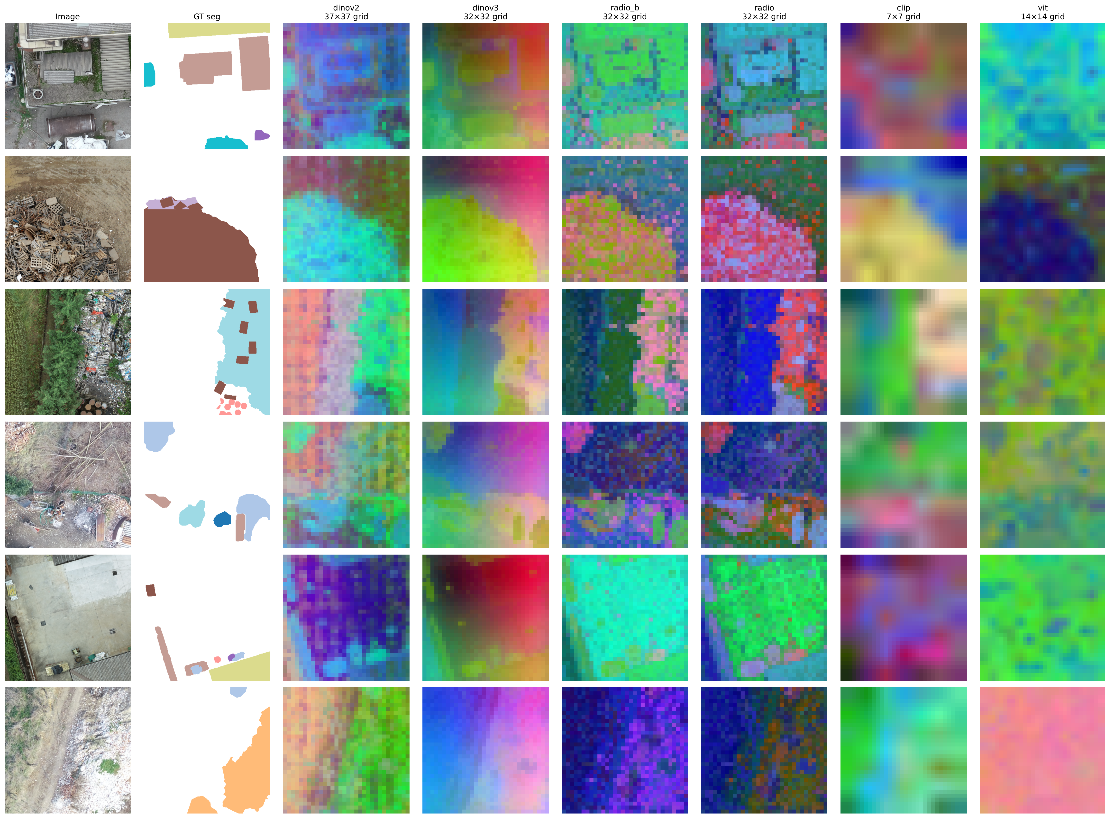
Patch-feature decomposition — 3-comp PCA → RGB
