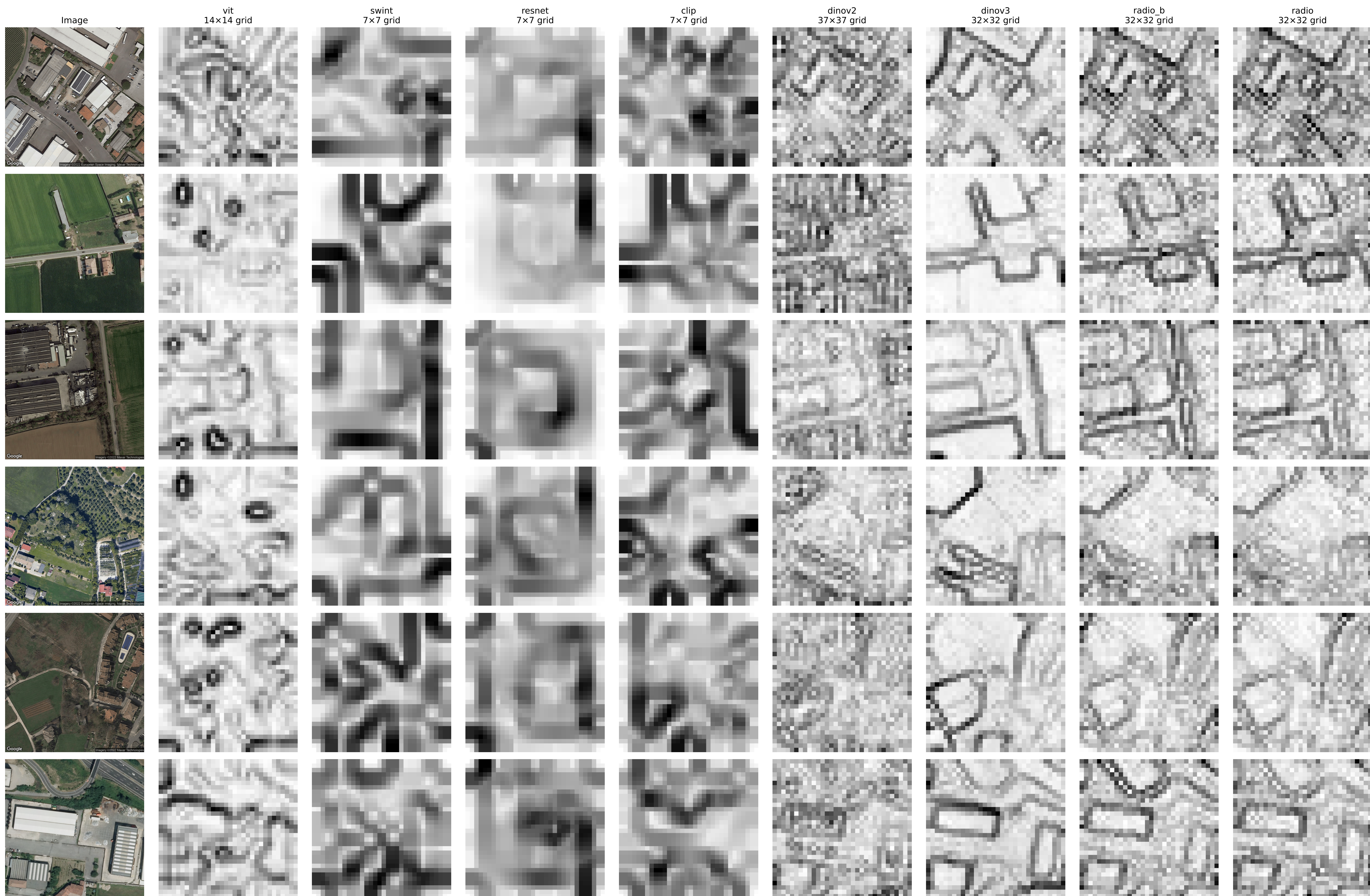
Patch-feature decomposition — PCA region boundaries (B&W)
