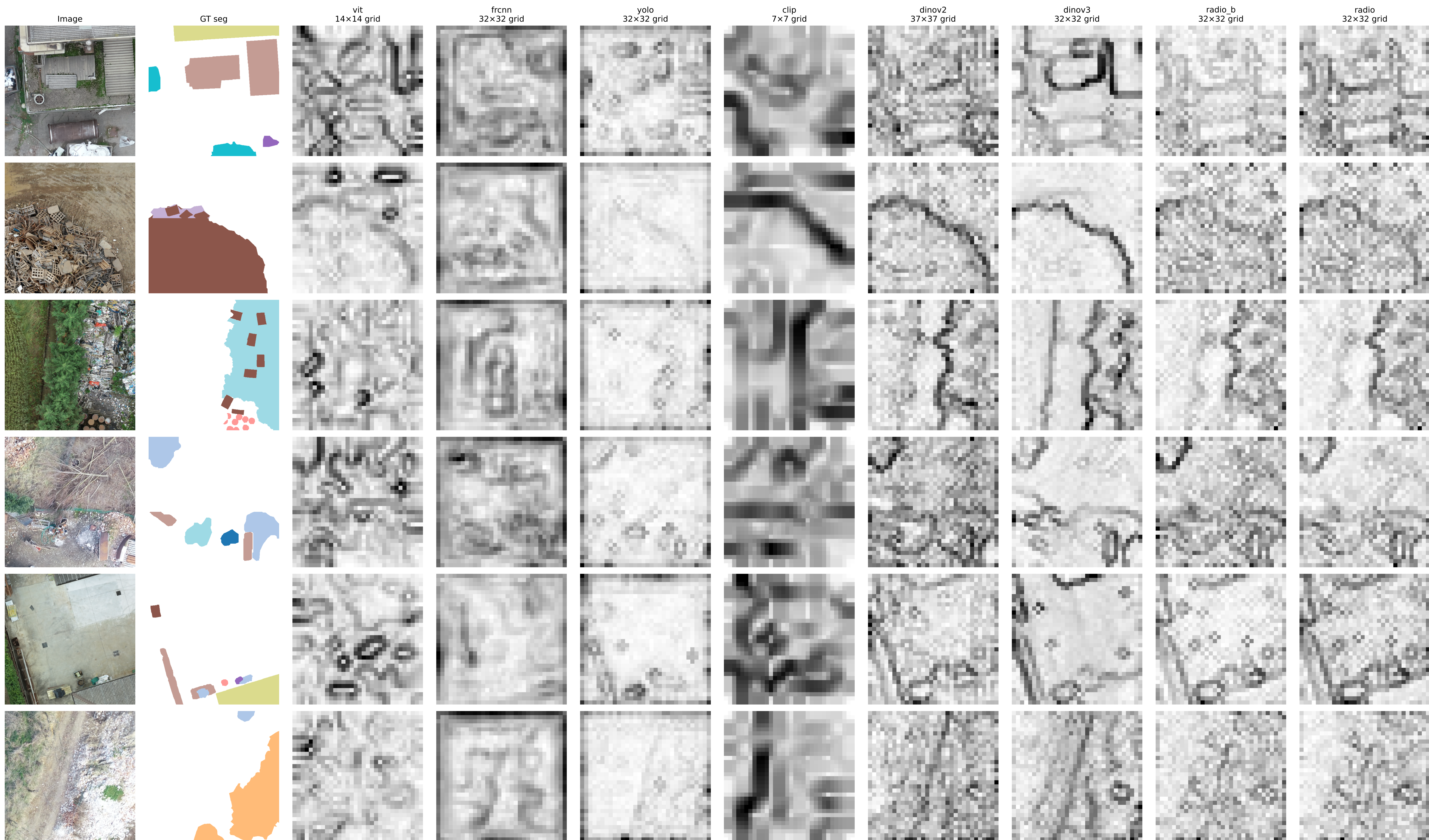
Patch-feature decomposition — PCA region boundaries (B&amp;W)
