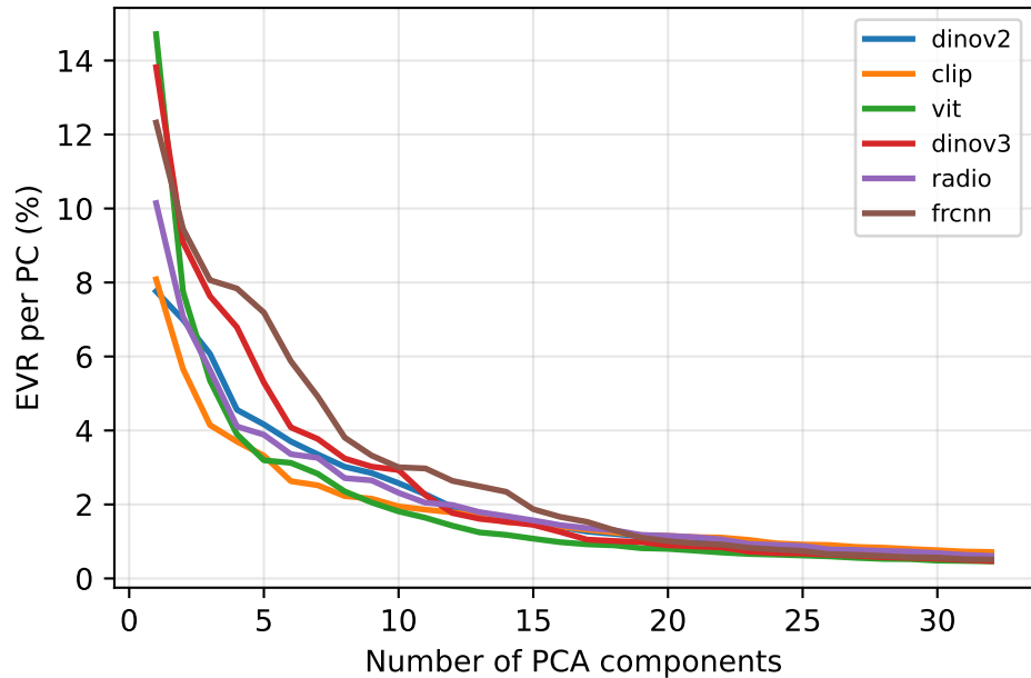
Per-component explained variance
