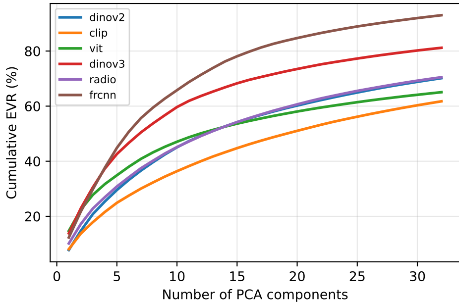
Cumulative explained variance
