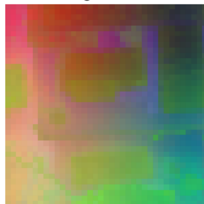
dinov3 @ 592 2 (37×37)
