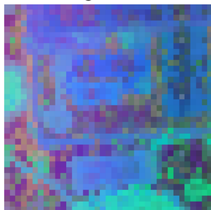
dinov2 @ 518 2 (37×37)
