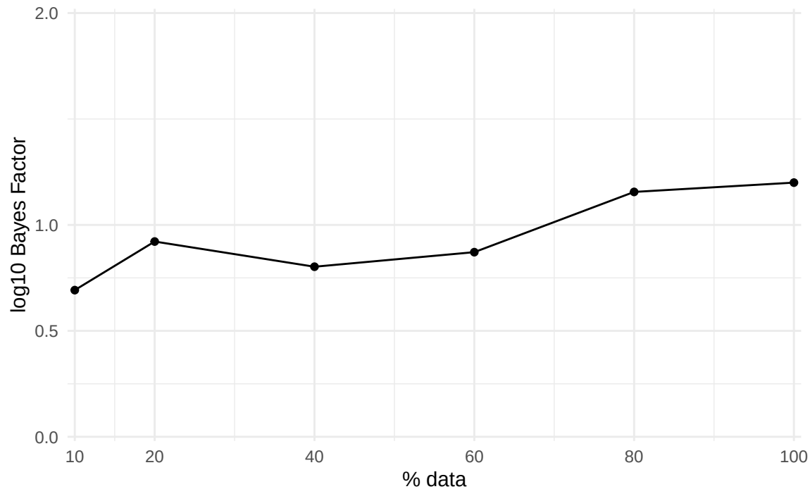
Bayes factor for \sigma_A < 0.01
