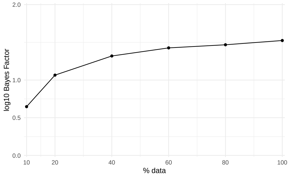
Bayes factor for \sigma_A < 0.05
