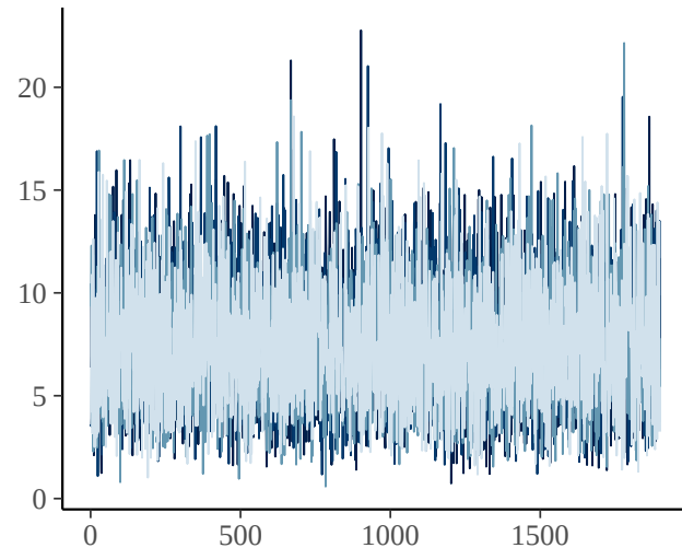
alpha_B
