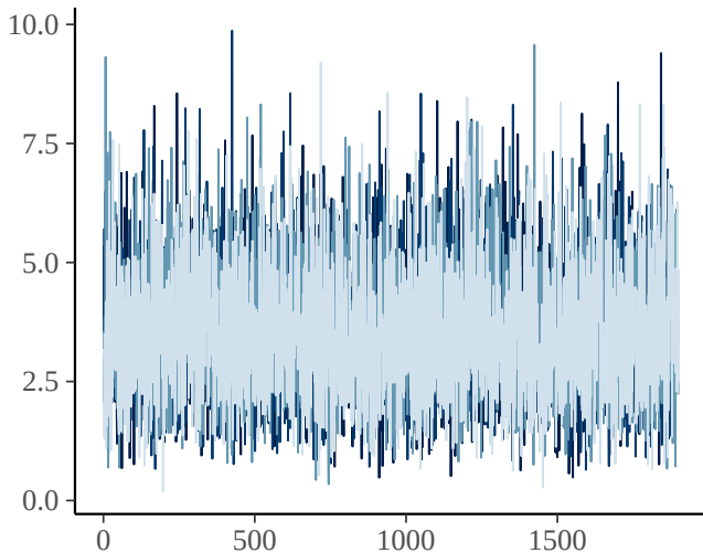
alpha_A
