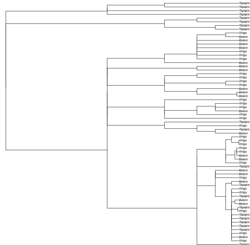
non-focal window 2 random tree sampled from 56 local coalescence trees in window scaffold_32:12260717
