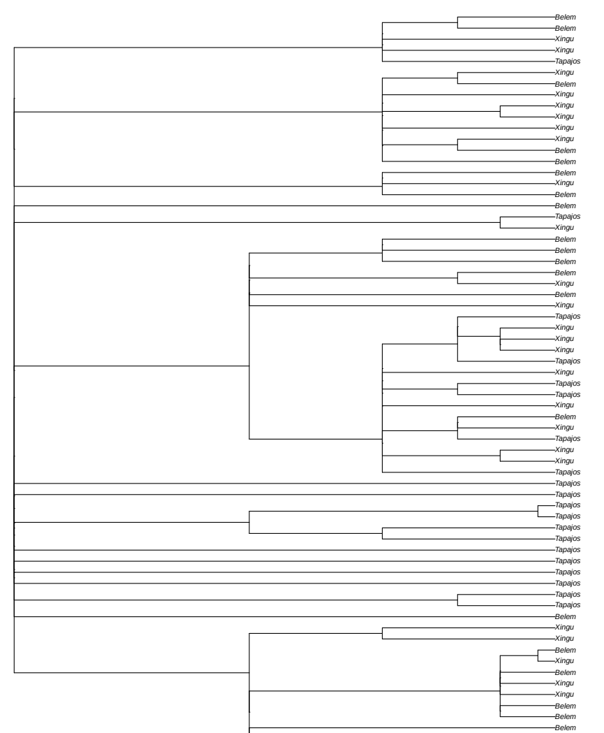
non-focal window 2 random tree sampled from 56 local coalescence trees in window scaffold_32:12260717
