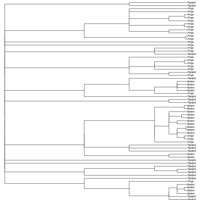
non-focal window 1 random tree sampled from 82 local coalescence trees in window scaffold_32:10764884
