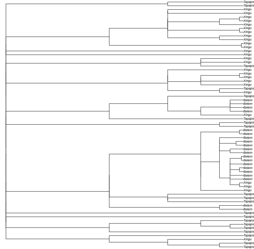
focal window random tree sampled from 47 local coalescence trees in window scaffold_32:11516537
