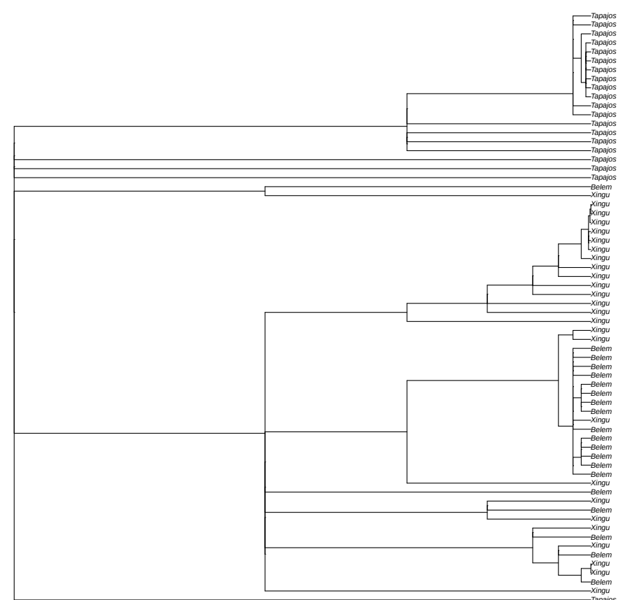
focal window random tree sampled from 9 local coalescence trees in window scaffold_13:16772897
