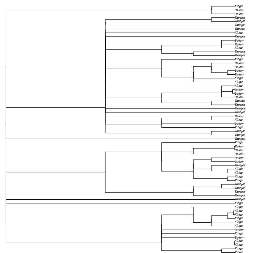
non-focal window 2 random tree sampled from 117 local coalescence trees in window scaffold_13:16270849
