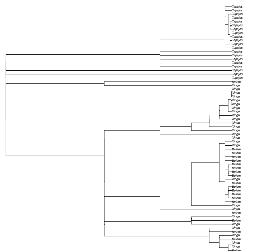
non-focal window 1 random tree sampled from 270 local coalescence trees in window scaffold_13:15771802
