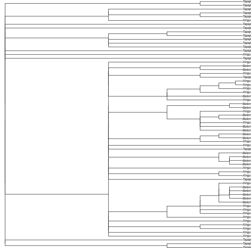
non-focal window 2 random tree sampled from 38 local coalescence trees in window scaffold_22:12854687
