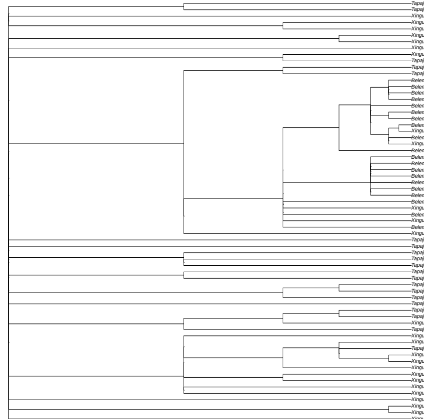
focal window random tree sampled from 53 local coalescence trees in window scaffold_22:12104432
