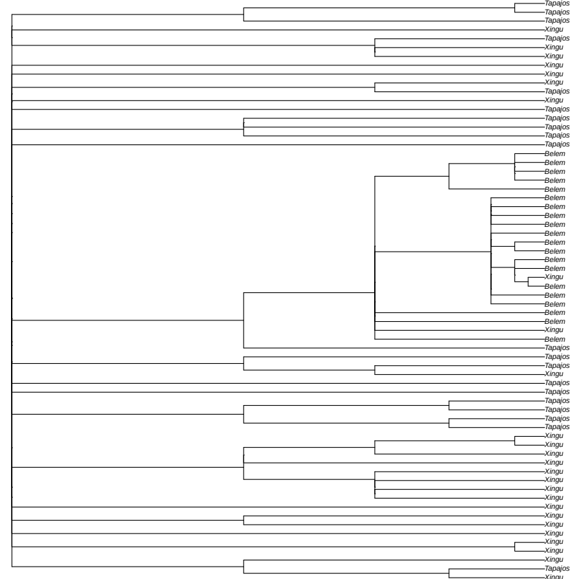
non-focal window 1 random tree sampled from 33 local coalescence trees in window scaffold_22:11352053
