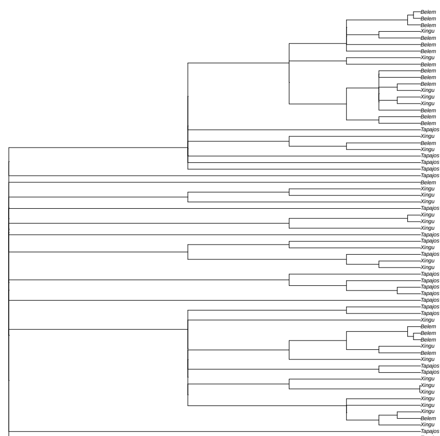
non-focal window 1 random tree sampled from 101 local coalescence trees in window scaffold_6:4123512
