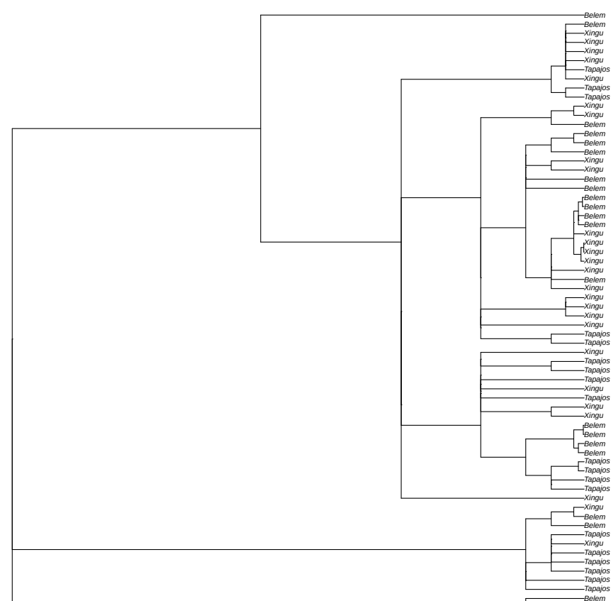
non-focal window 2 random tree sampled from 88 local coalescence trees in window scaffold_6:5620752
