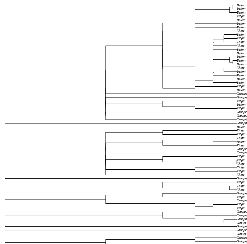
focal window random tree sampled from 96 local coalescence trees in window scaffold_6:4870269
