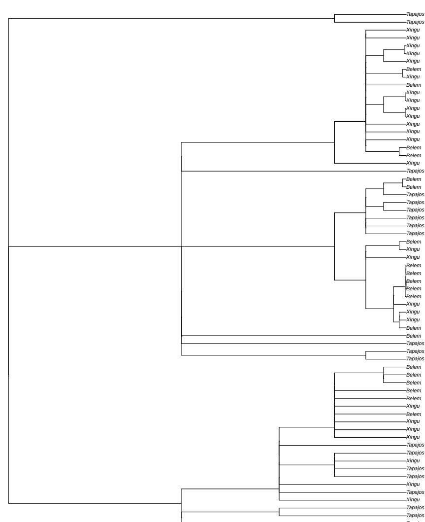
non-focal window 2 random tree sampled from 88 local coalescence trees in window scaffold_6:5620752
