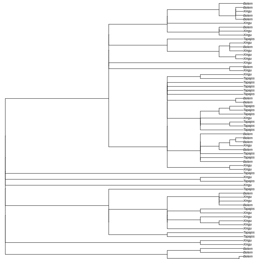
non-focal window 2 random tree sampled from 119 local coalescence trees in window scaffold_9:6268347
