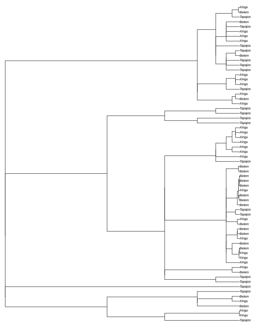
non-focal window 2 random tree sampled from 119 local coalescence trees in window scaffold_9:6268347
