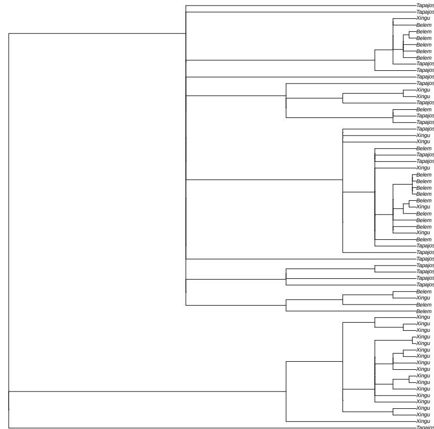
non-focal window 1 random tree sampled from 102 local coalescence trees in window scaffold_9:4763084
