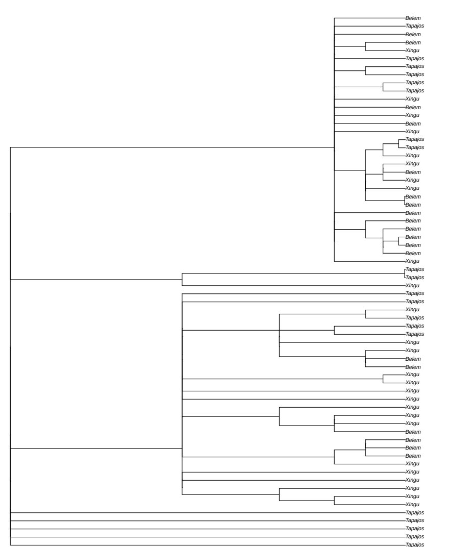
non-focal window 2 random tree sampled from 96 local coalescence trees in window scaffold_26:7697584
