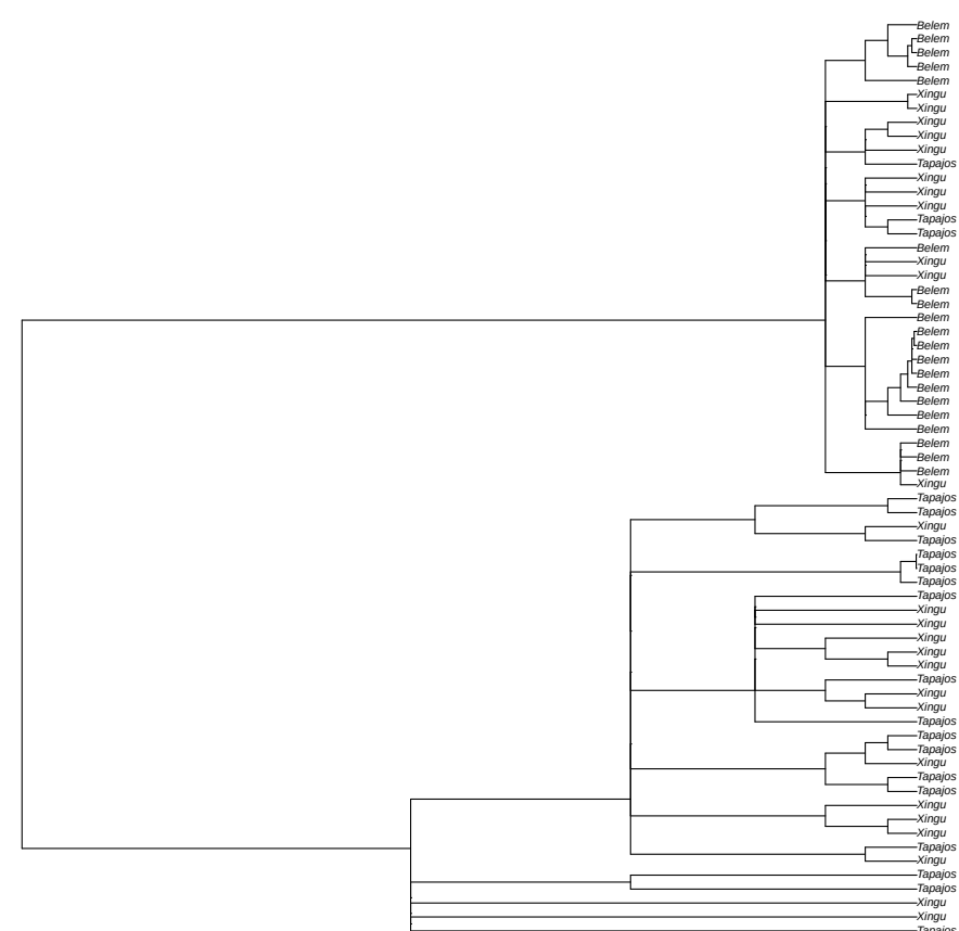
focal window random tree sampled from 69 local coalescence trees in window scaffold_26:6941234
