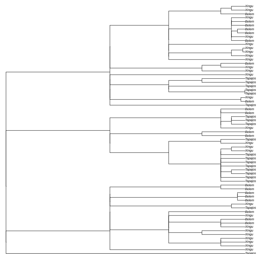
non-focal window 2 random tree sampled from 96 local coalescence trees in window scaffold_26:7697584
