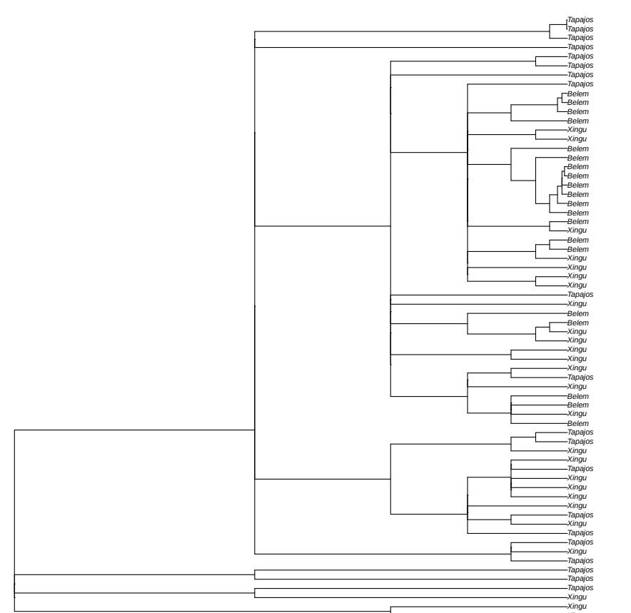
non-focal window 1 random tree sampled from 124 local coalescence trees in window scaffold_26:6198007
