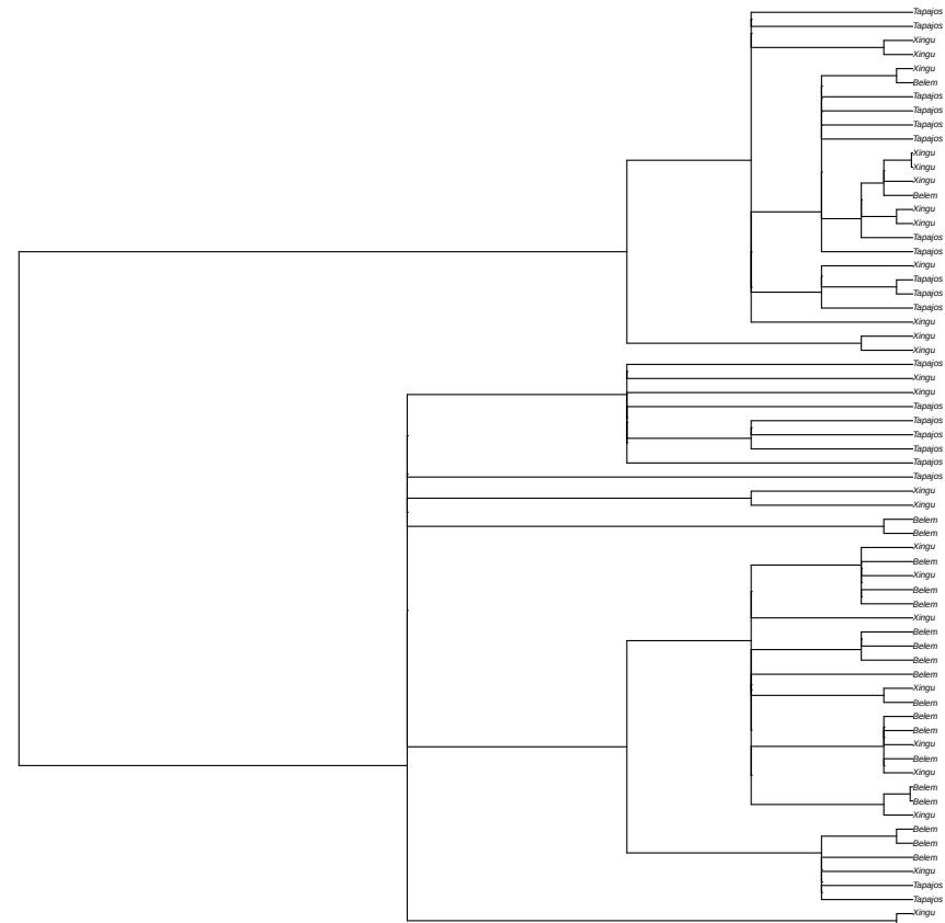
non-focal window 2 random tree sampled from 517 local coalescence trees in window scaffold_52:1359919
