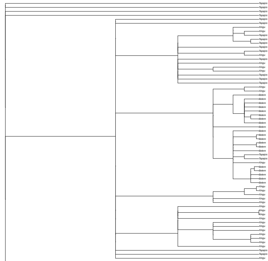
non-focal window 1 random tree sampled from 349 local coalescence trees in window scaffold_52:856842
