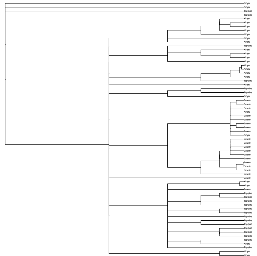
non-focal window 1 random tree sampled from 487 local coalescence trees in window scaffold_24:563537
