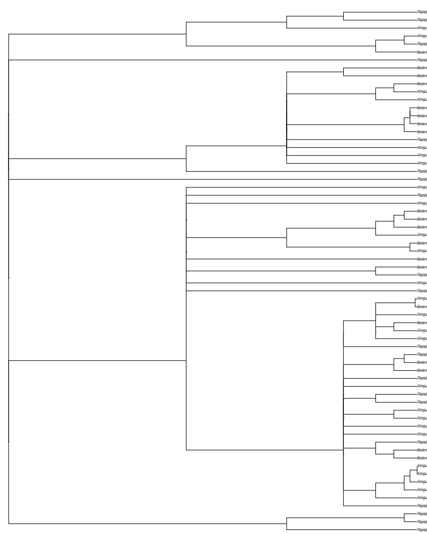
non-focal window 2 random tree sampled from 510 local coalescence trees in window scaffold_24:1064229
