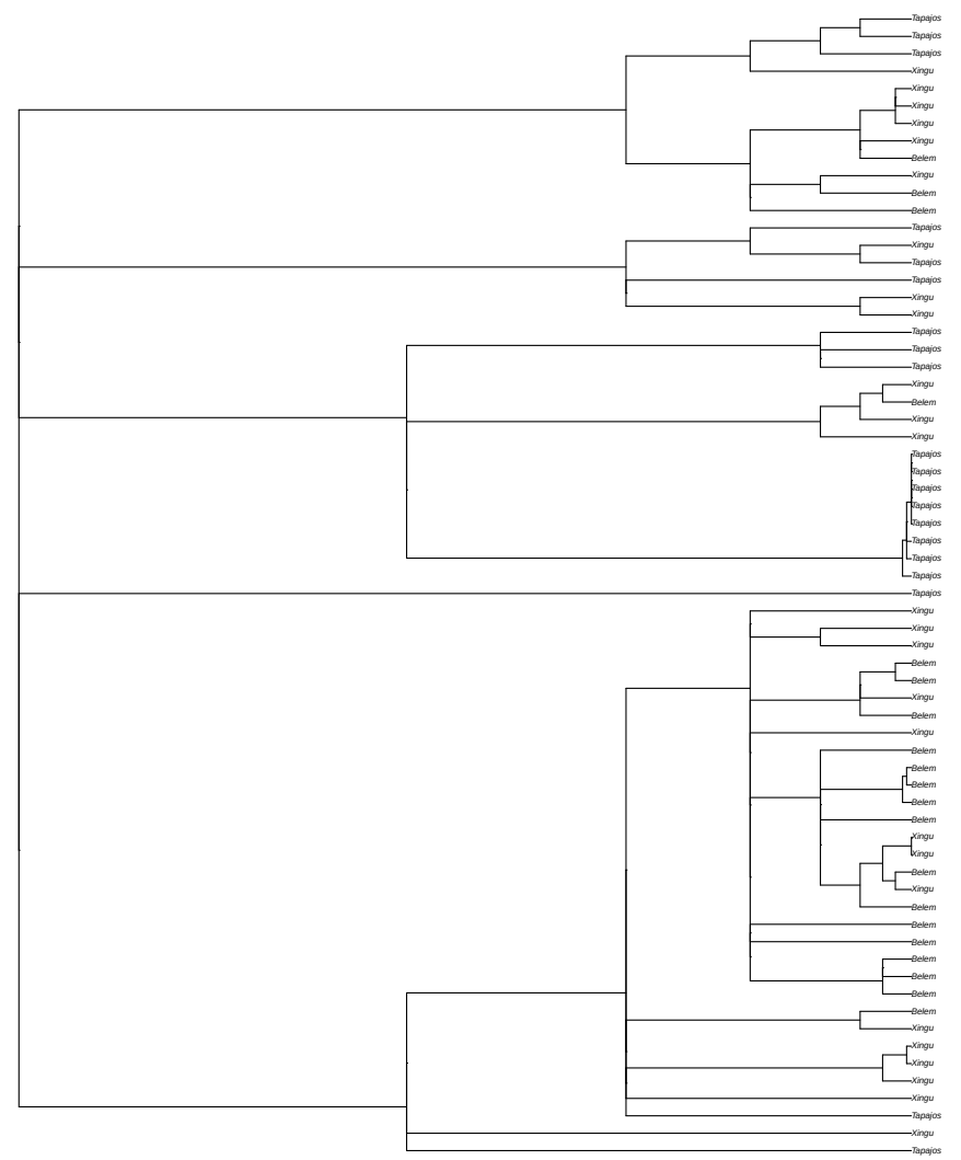
non-focal window 2 random tree sampled from 117 local coalescence trees in window scaffold_13:16270849
