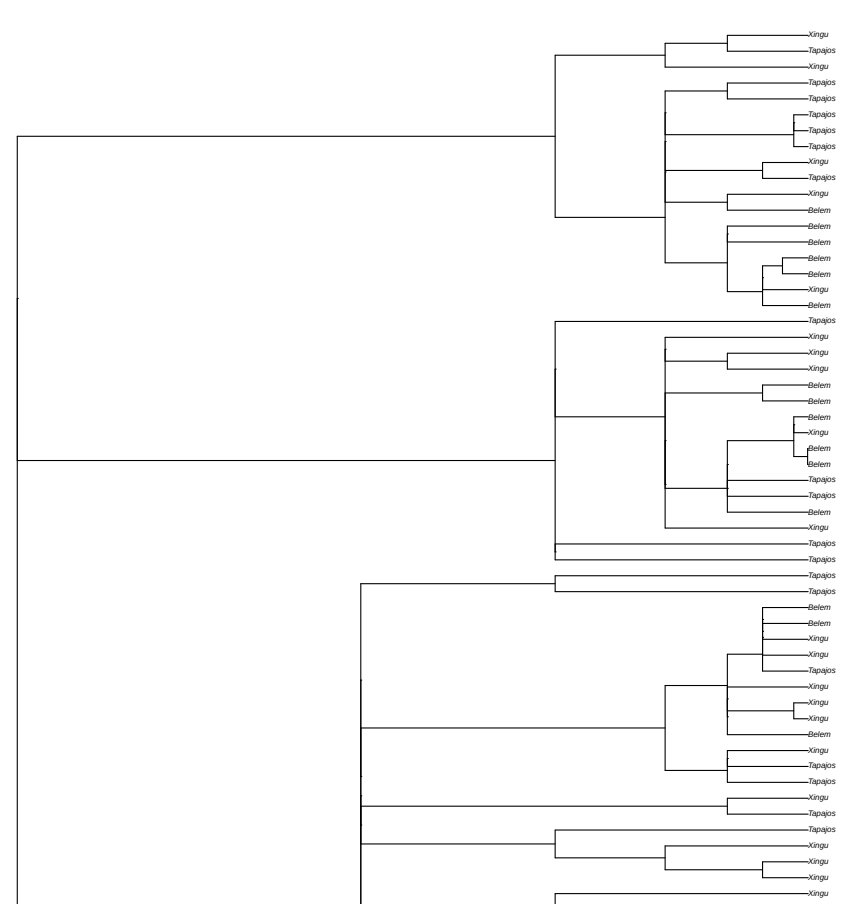
non-focal window 2 random tree sampled from 612 local coalescence trees in window scaffold_64:2523724
