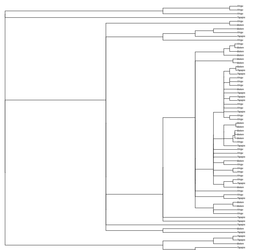
non-focal window 2 random tree sampled from 612 local coalescence trees in window scaffold_64:2523724
