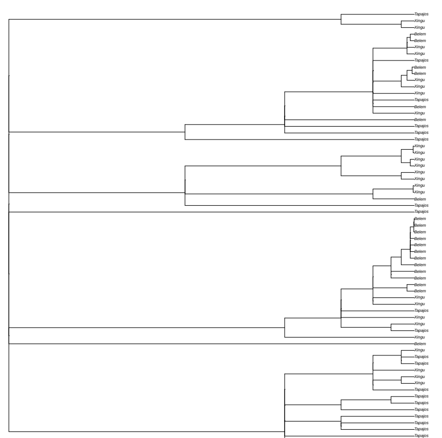
non-focal window 1 random tree sampled from 550 local coalescence trees in window scaffold_64:1020329
