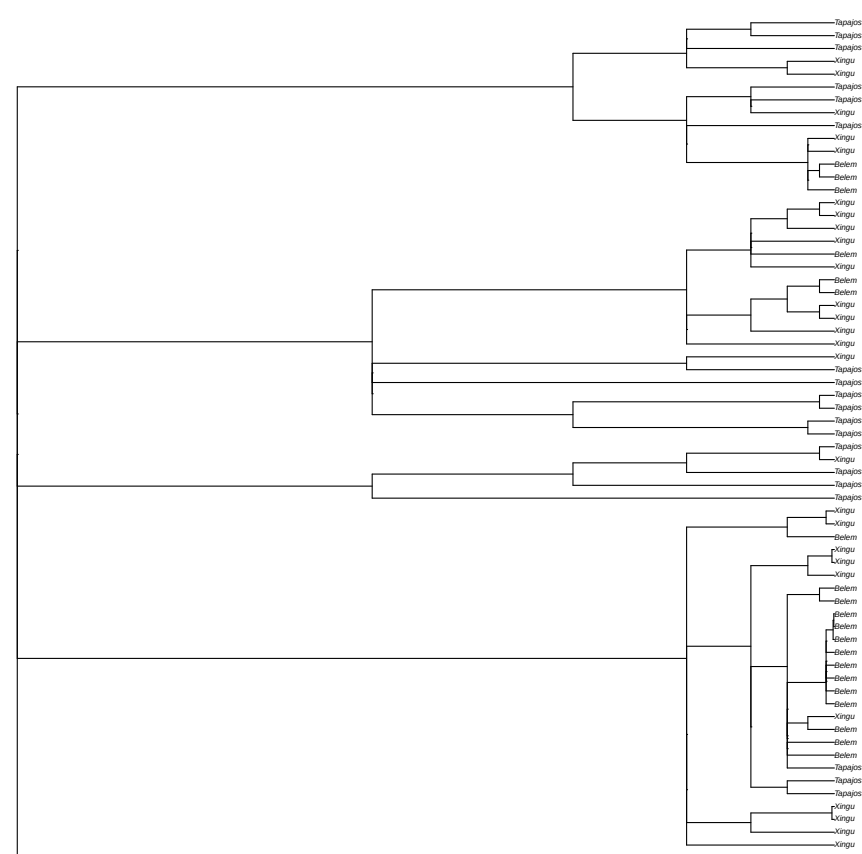
focal window random tree sampled from 448 local coalescence trees in window scaffold_64:1770579
