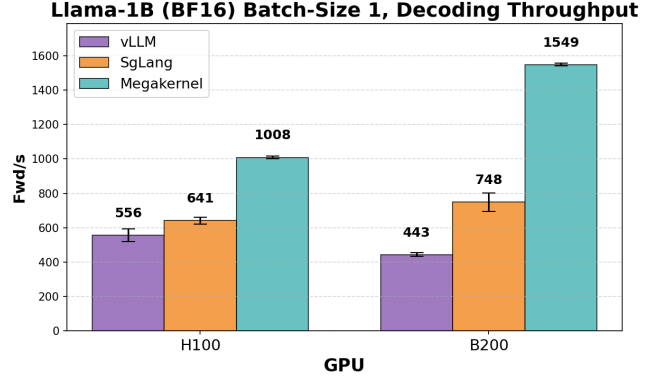
Figure 1. Reproduced baseline and mega-kernel results on both H100 and B200. Each bar graph is mean token/s over 3 iterations.
