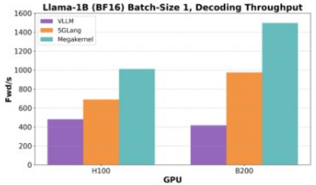
Figure 2. Baseline results from the blog
